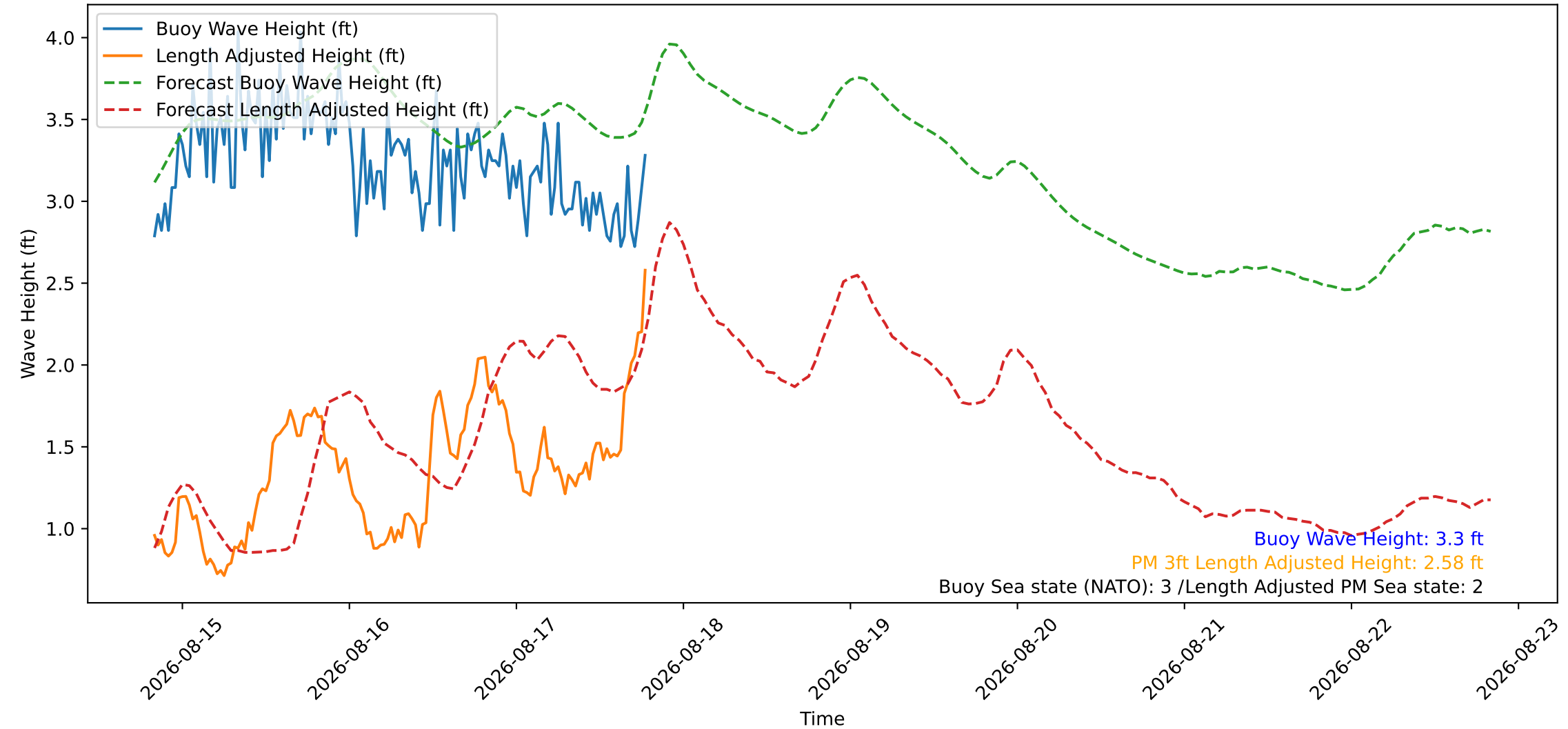
Wave Heights over Time for Red Beach at 2026-08-17 19:30:46
