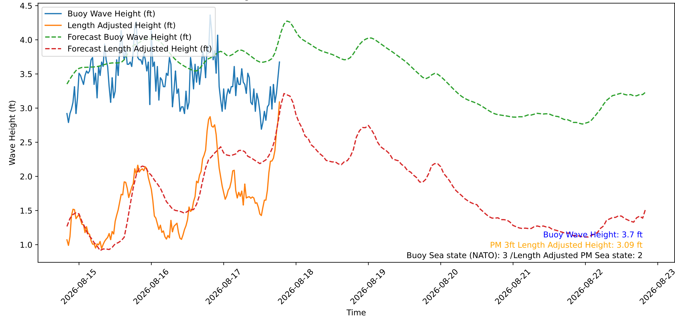
Wave Heights over Time for Green Beach at 2026-08-17 19:31:09
