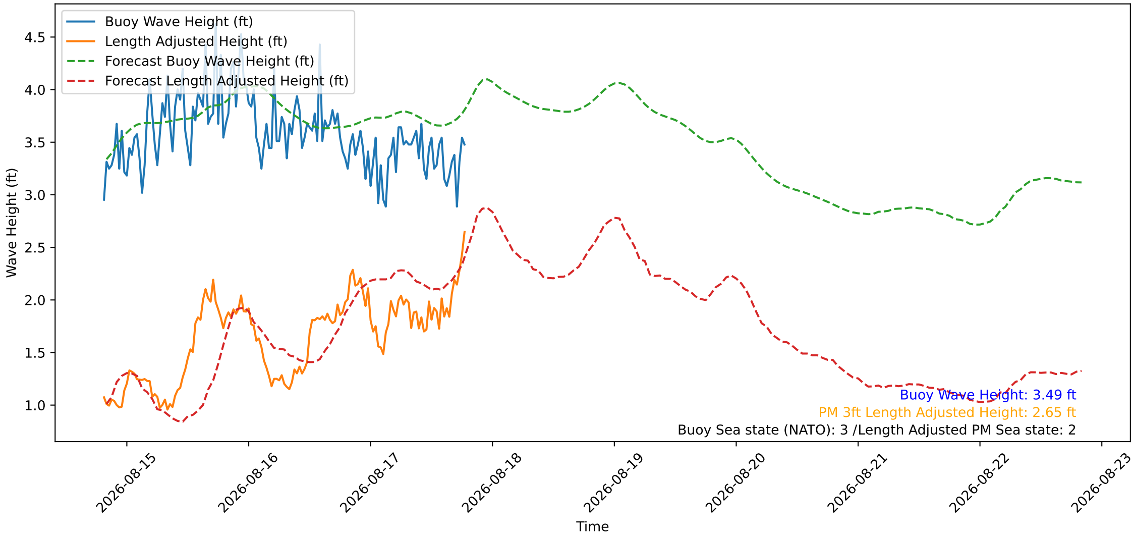
Wave Heights over Time for Oceanside Harbor at 2026-08-17 19:30:26
