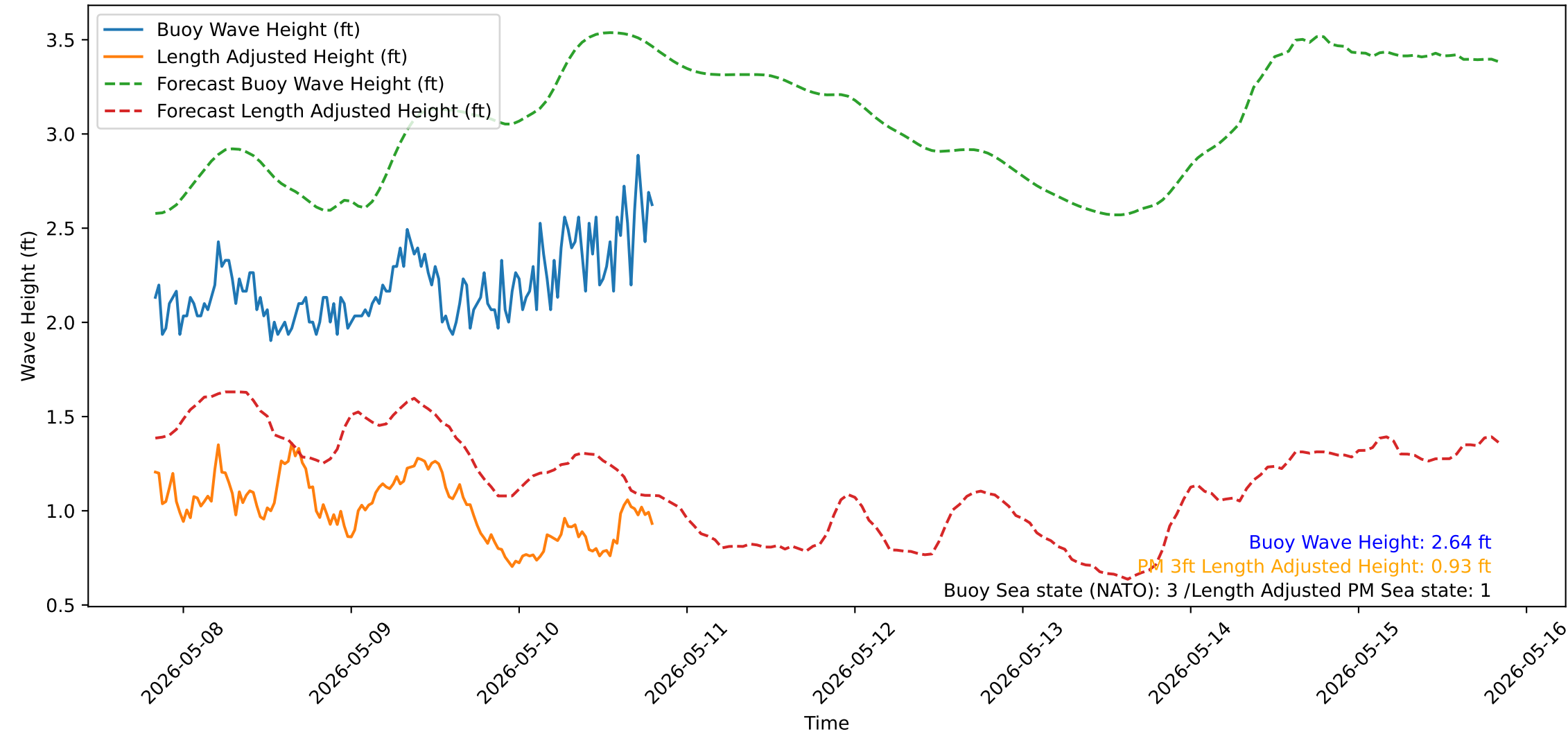
Wave Heights over Time for Red Beach at 2026-05-10 19:50:52
