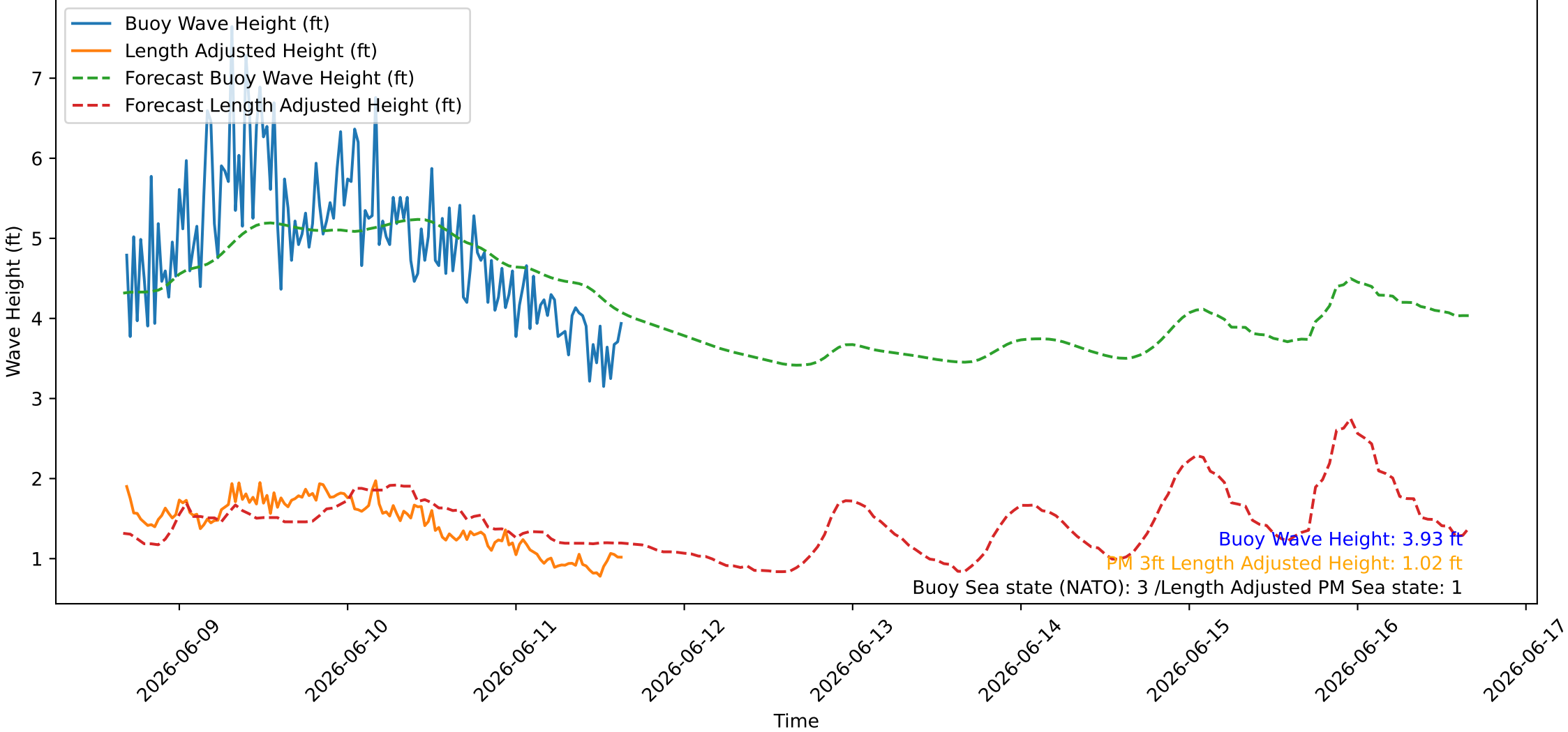
Wave Heights over Time for Red Beach at 2026-06-11 16:00:46
