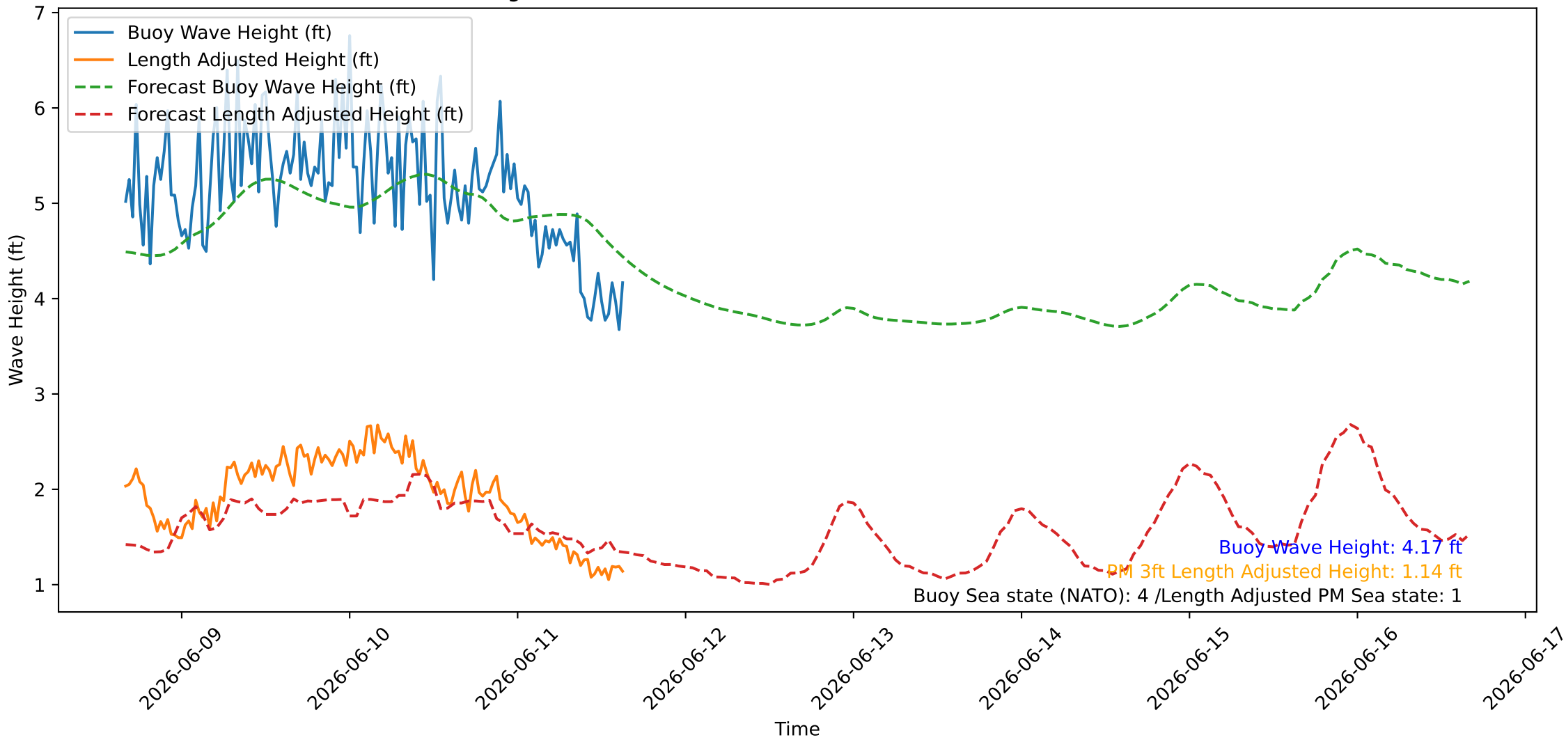
Wave Heights over Time for Oceanside Harbor at 2026-06-11 16:00:26
