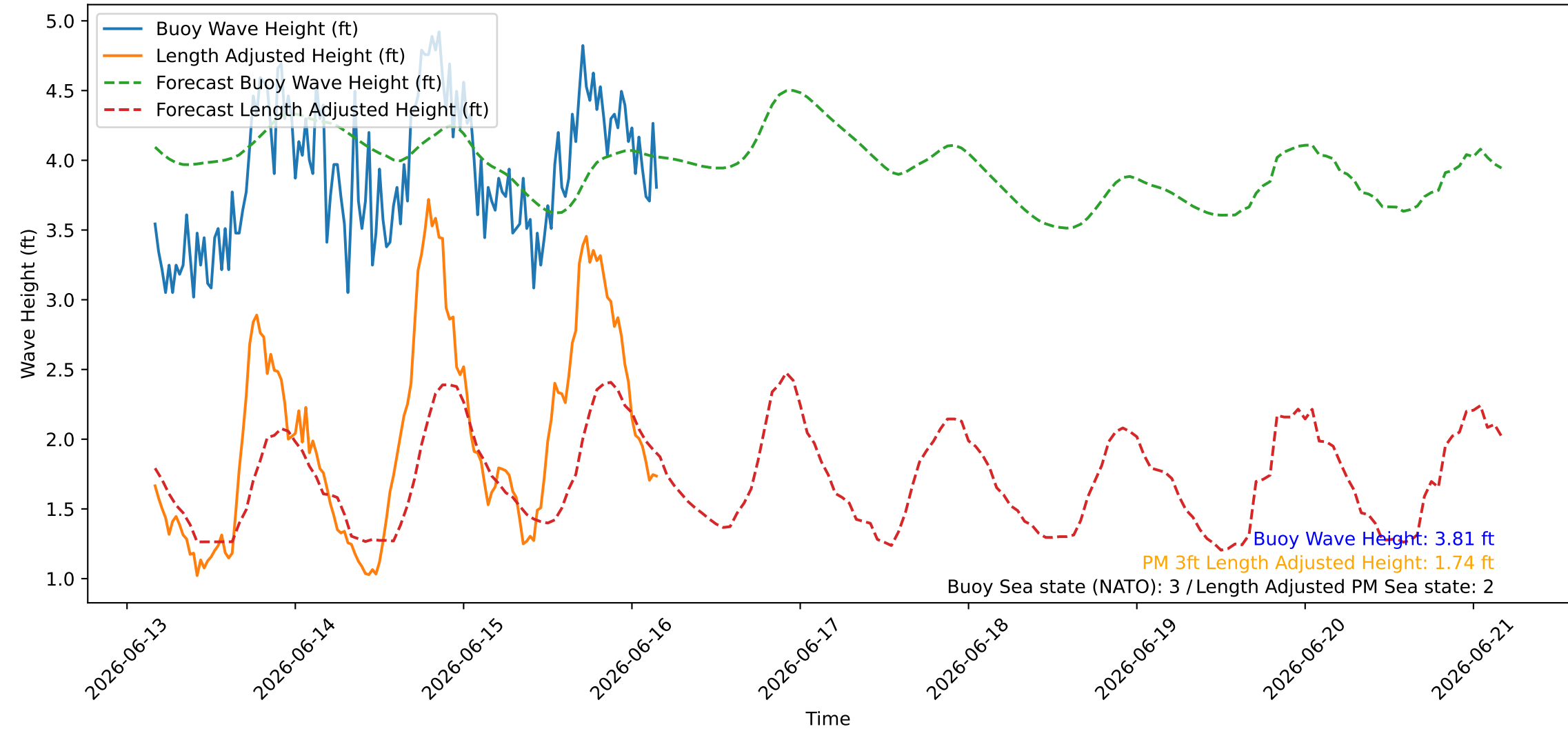
Wave Heights over Time for Green Beach at 2026-06-16 04:11:08
