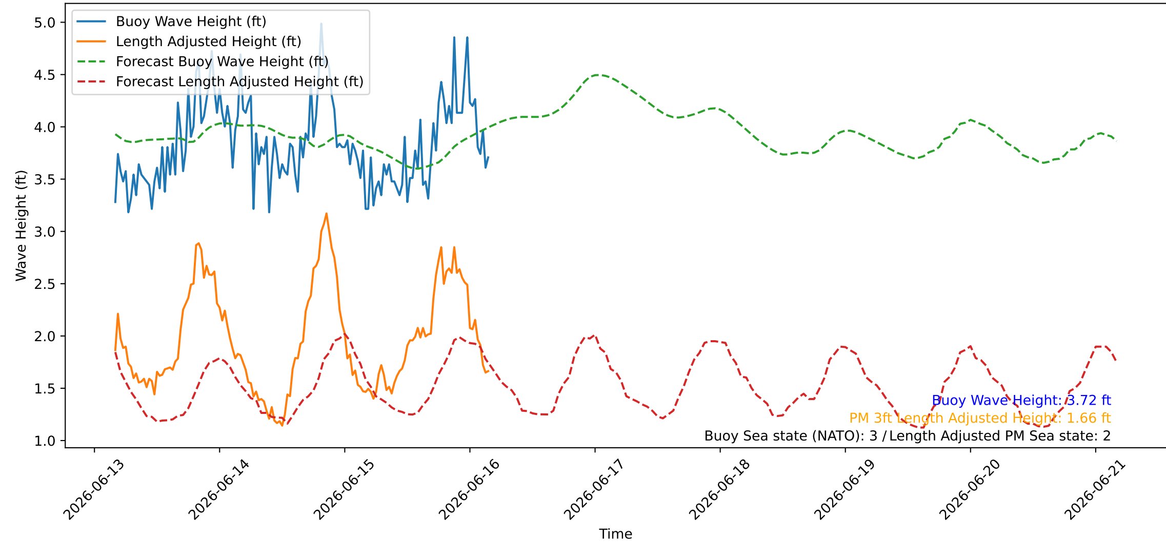
Wave Heights over Time for Oceanside Harbor at 2026-06-16 04:10:26
