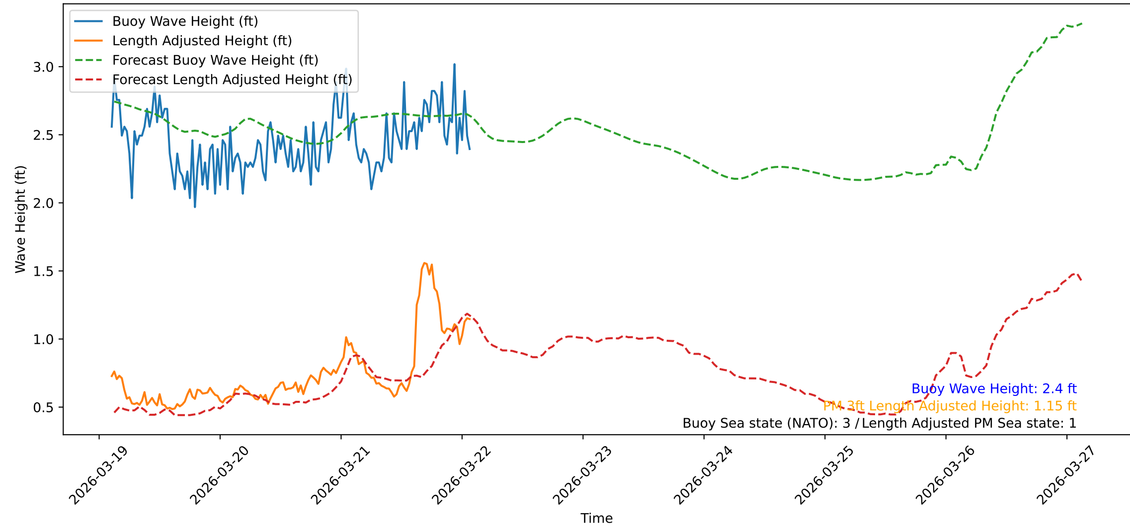
Wave Heights over Time for Oceanside Harbor at 2026-03-22 02:40:32
