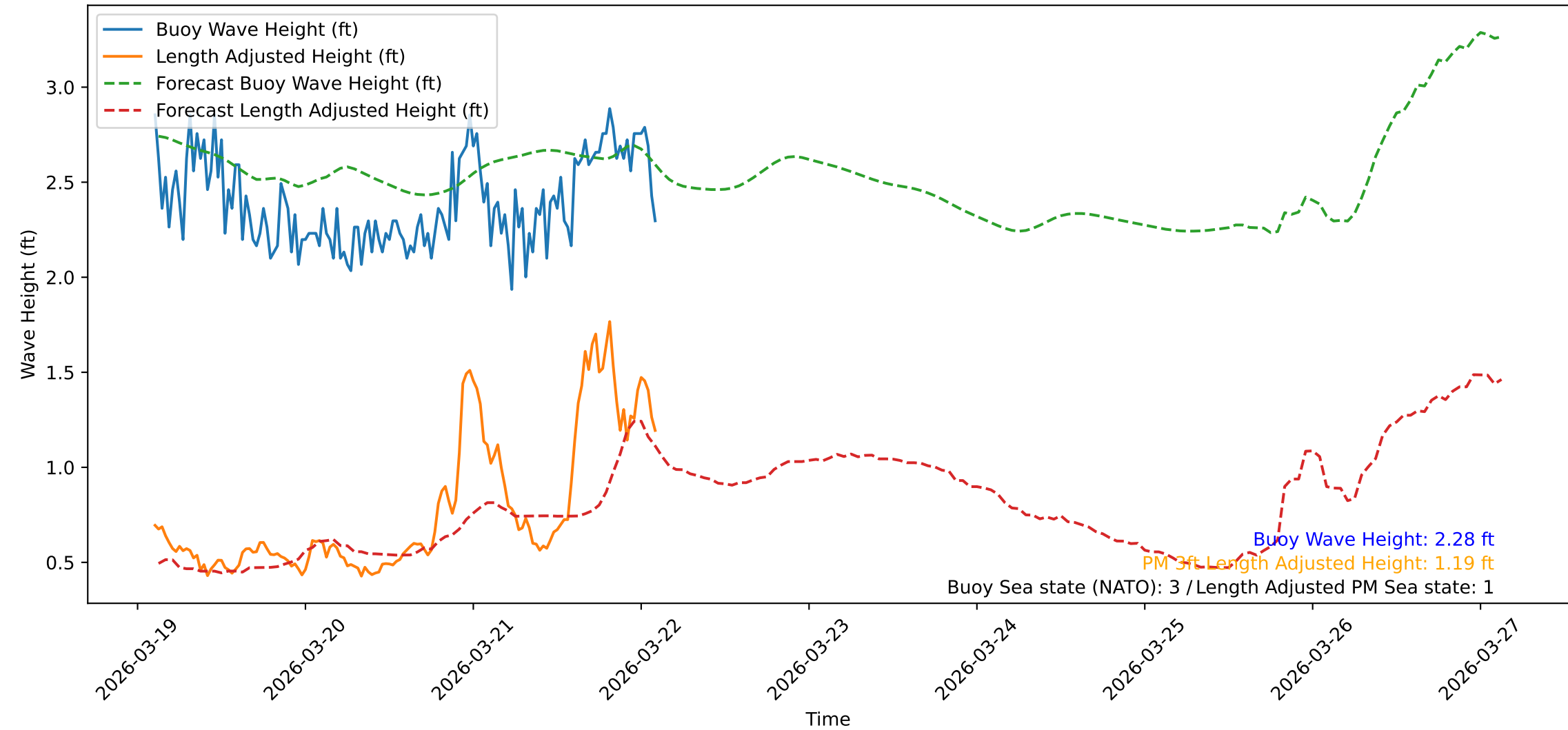
Wave Heights over Time for Green Beach at 2026-03-22 02:41:10
