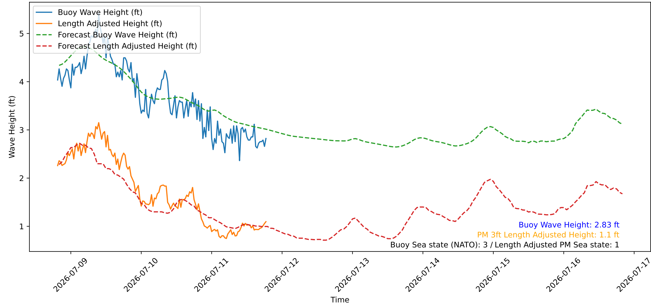
Wave Heights over Time for Oceanside Harbor at 2026-07-11 19:30:26
