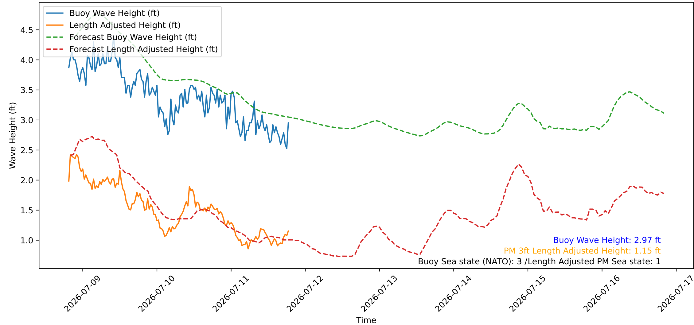
Wave Heights over Time for Green Beach at 2026-07-11 19:31:08
