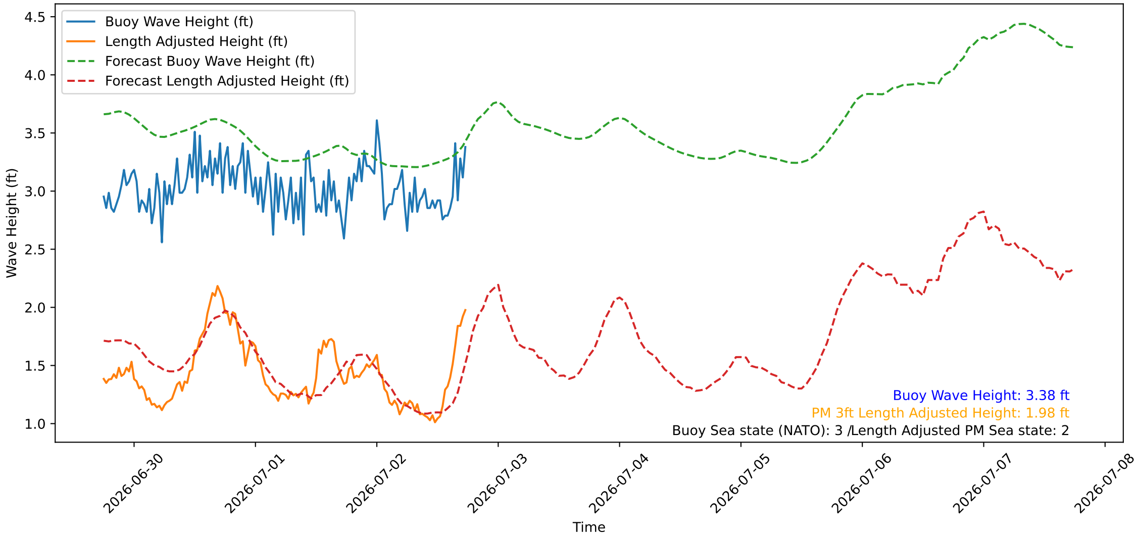
Wave Heights over Time for Oceanside Harbor at 2026-07-02 18:00:26
