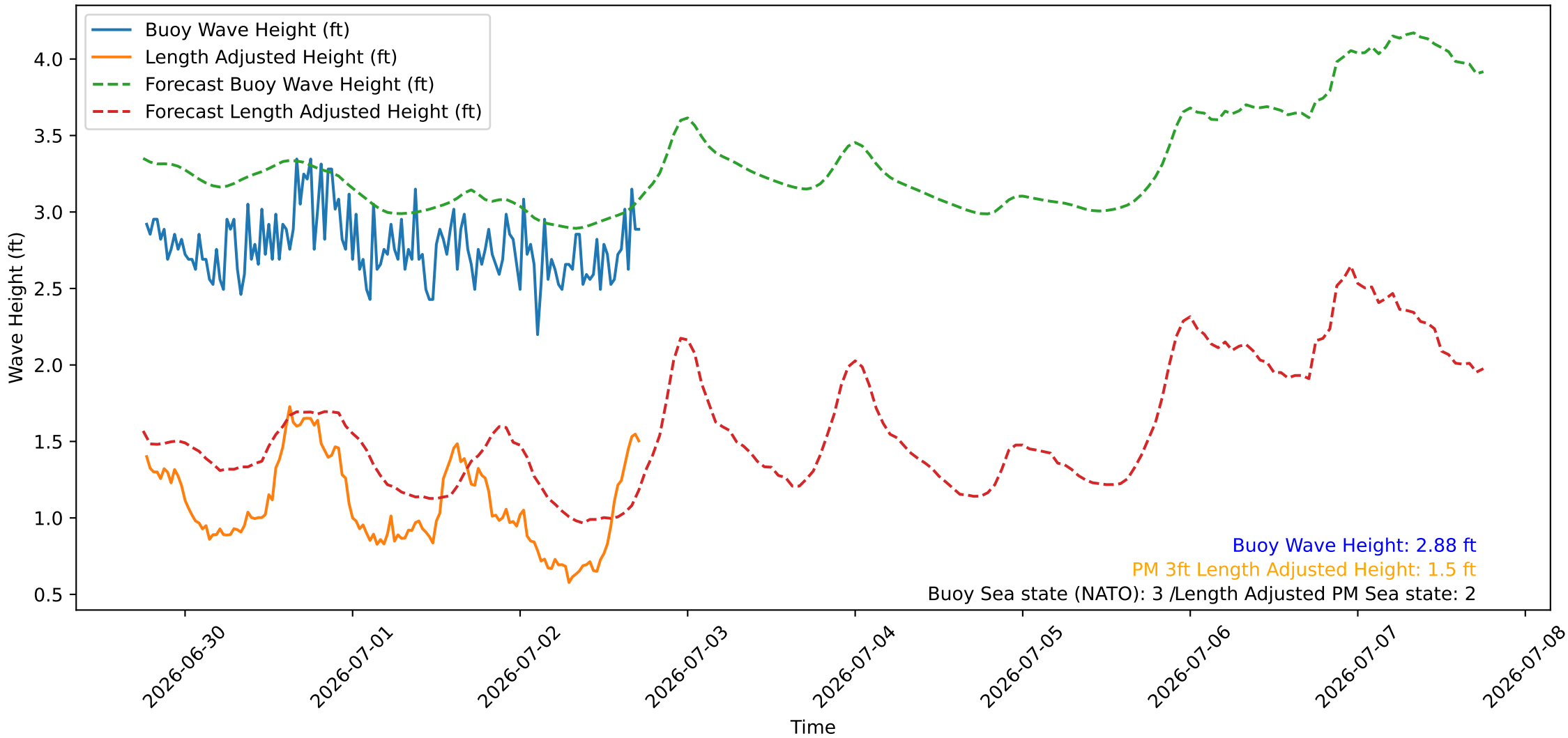
Wave Heights over Time for Red Beach at 2026-07-02 18:00:45
