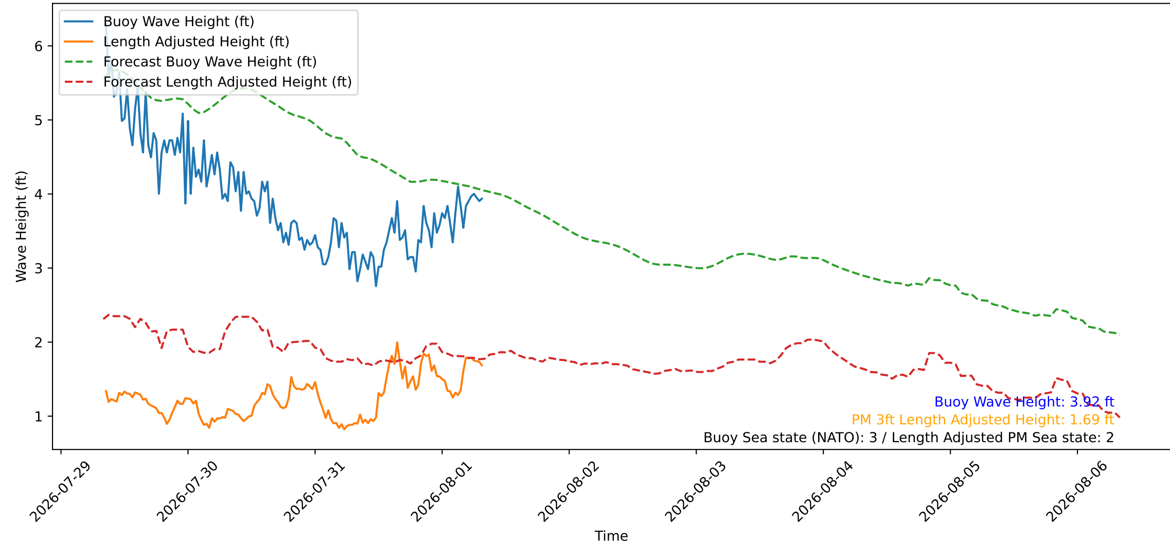
Wave Heights over Time for Green Beach at 2026-08-01 08:21:10
