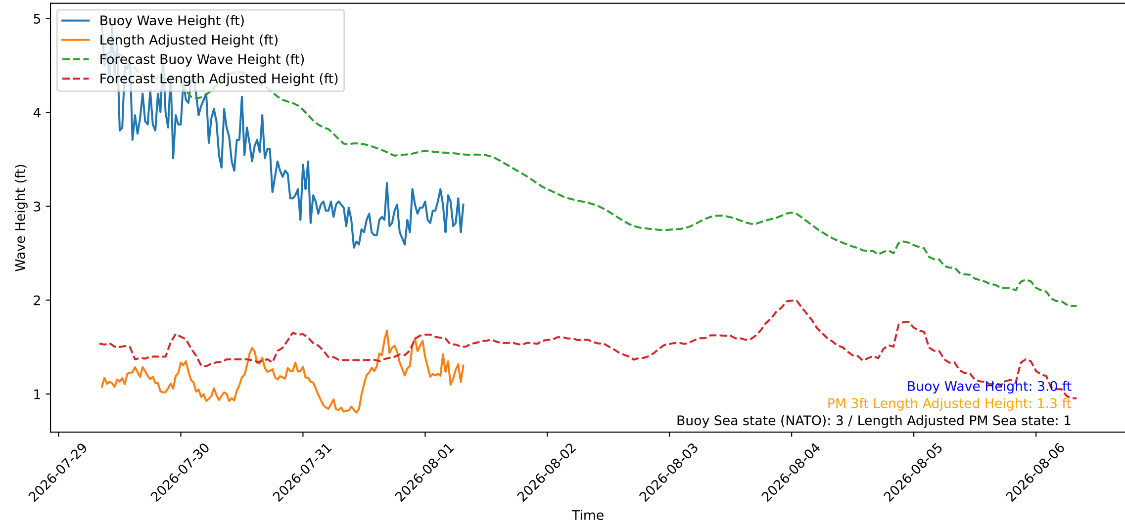
Wave Heights over Time for Red Beach at 2026-08-01 08:20:47
