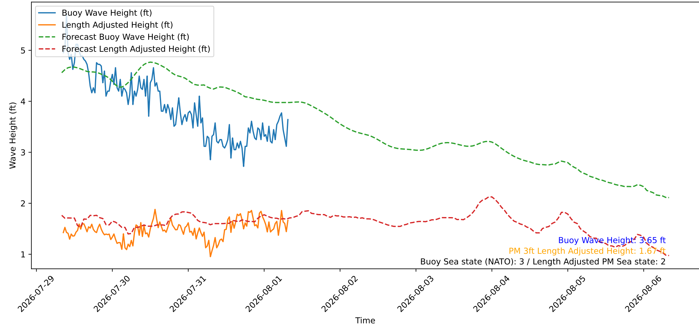
Wave Heights over Time for Oceanside Harbor at 2026-08-01 08:20:26
