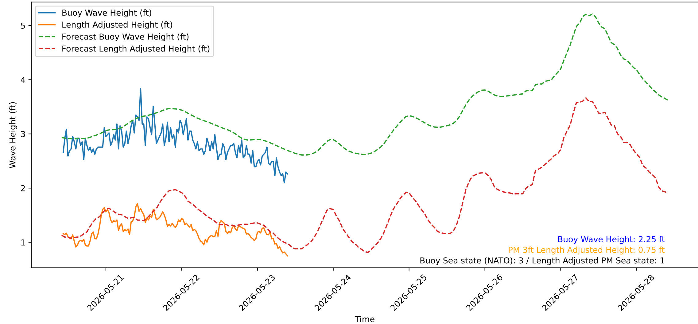
Wave Heights over Time for Oceanside Harbor at 2026-05-23 10:20:32
