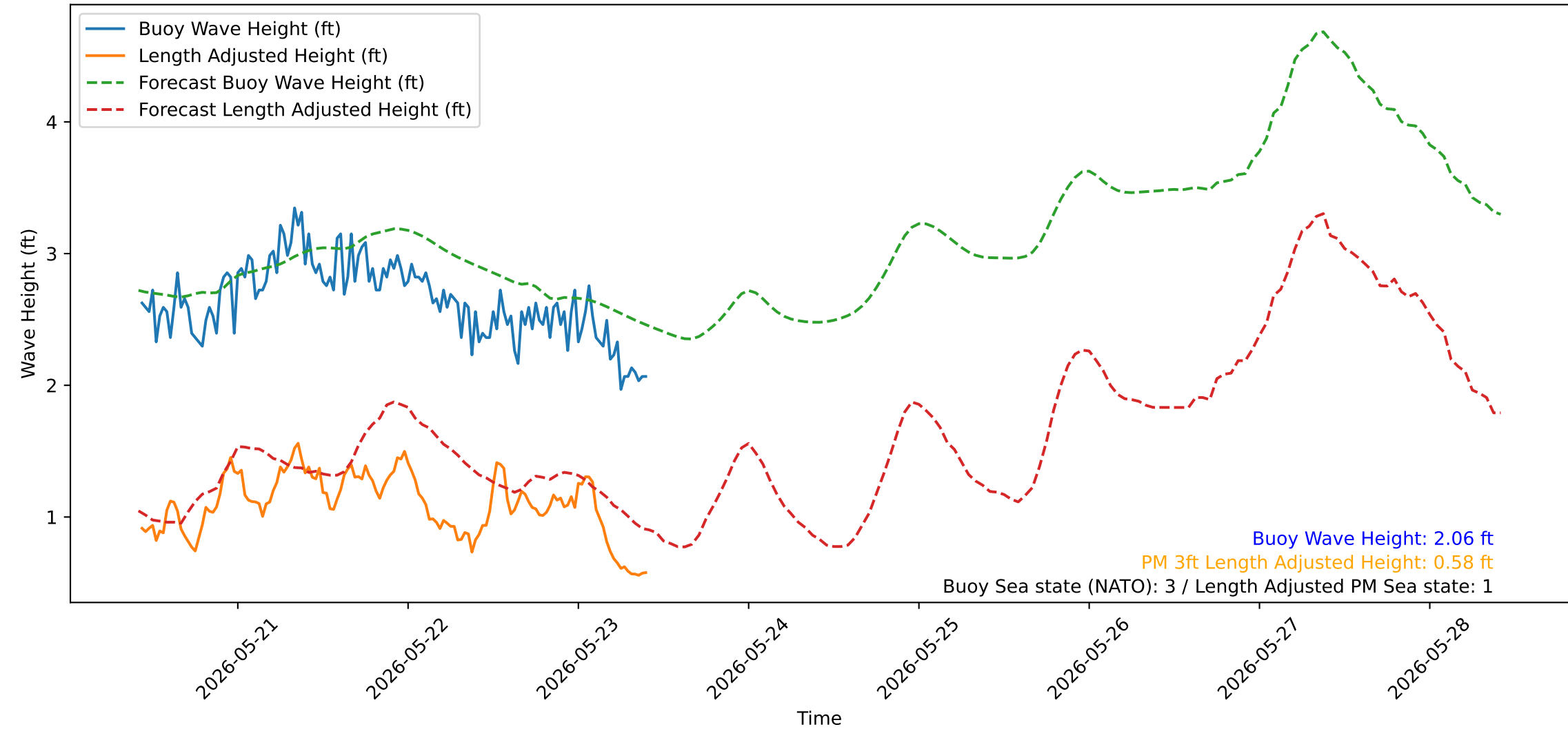
Wave Heights over Time for Red Beach at 2026-05-23 10:20:52
