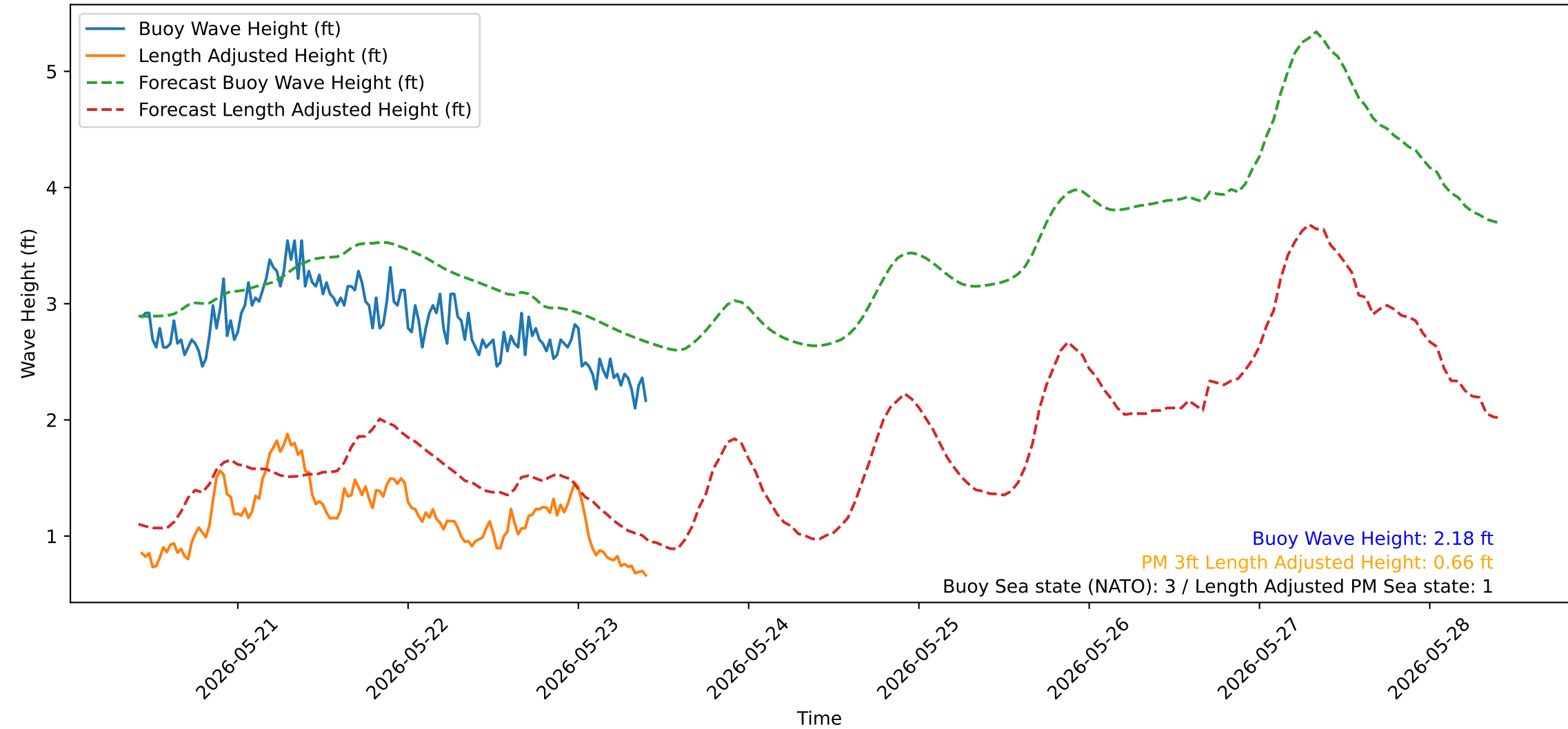
Wave Heights over Time for Green Beach at 2026-05-23 10:21:14
