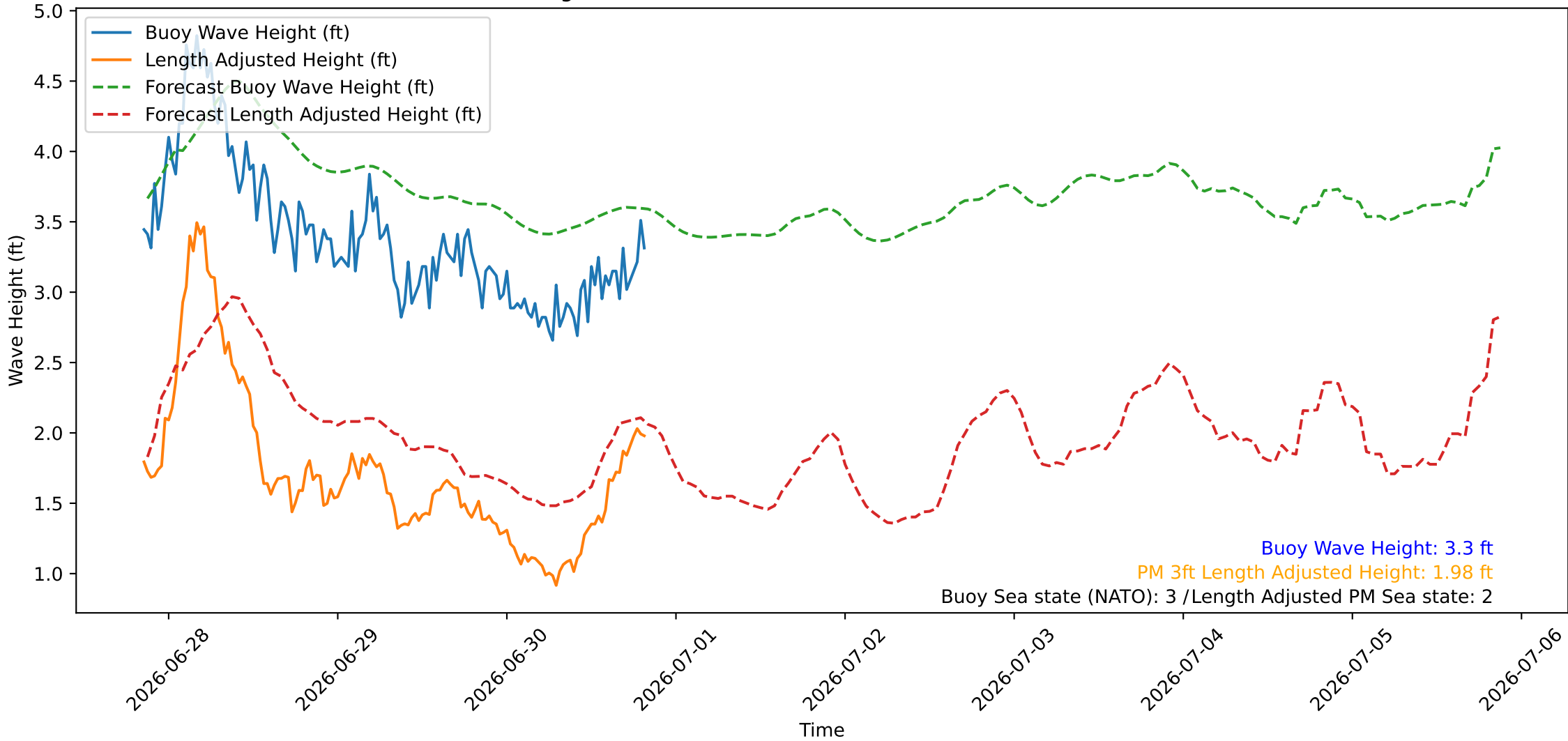
Wave Heights over Time for Green Beach at 2026-06-30 20:31:08
