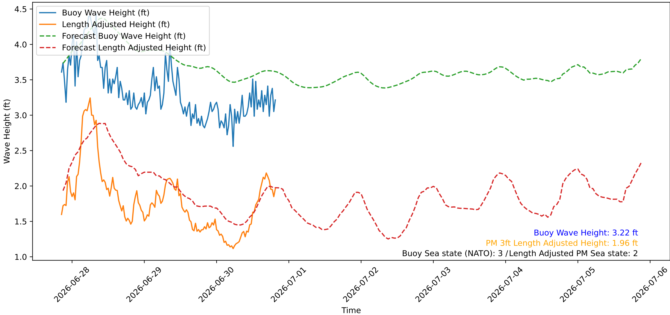
Wave Heights over Time for Oceanside Harbor at 2026-06-30 20:30:27
