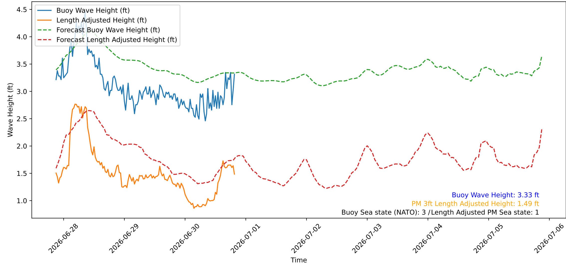
Wave Heights over Time for Red Beach at 2026-06-30 20:30:46
