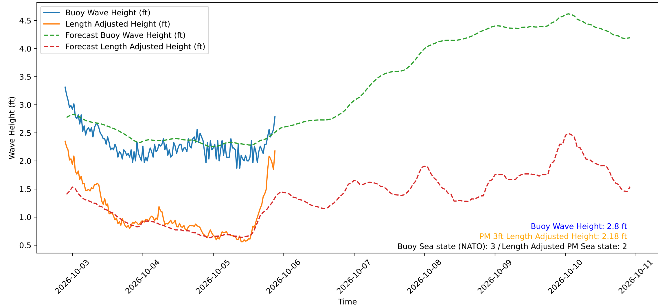
Wave Heights over Time for Oceanside Harbor at 2026-10-05 21:40:29
