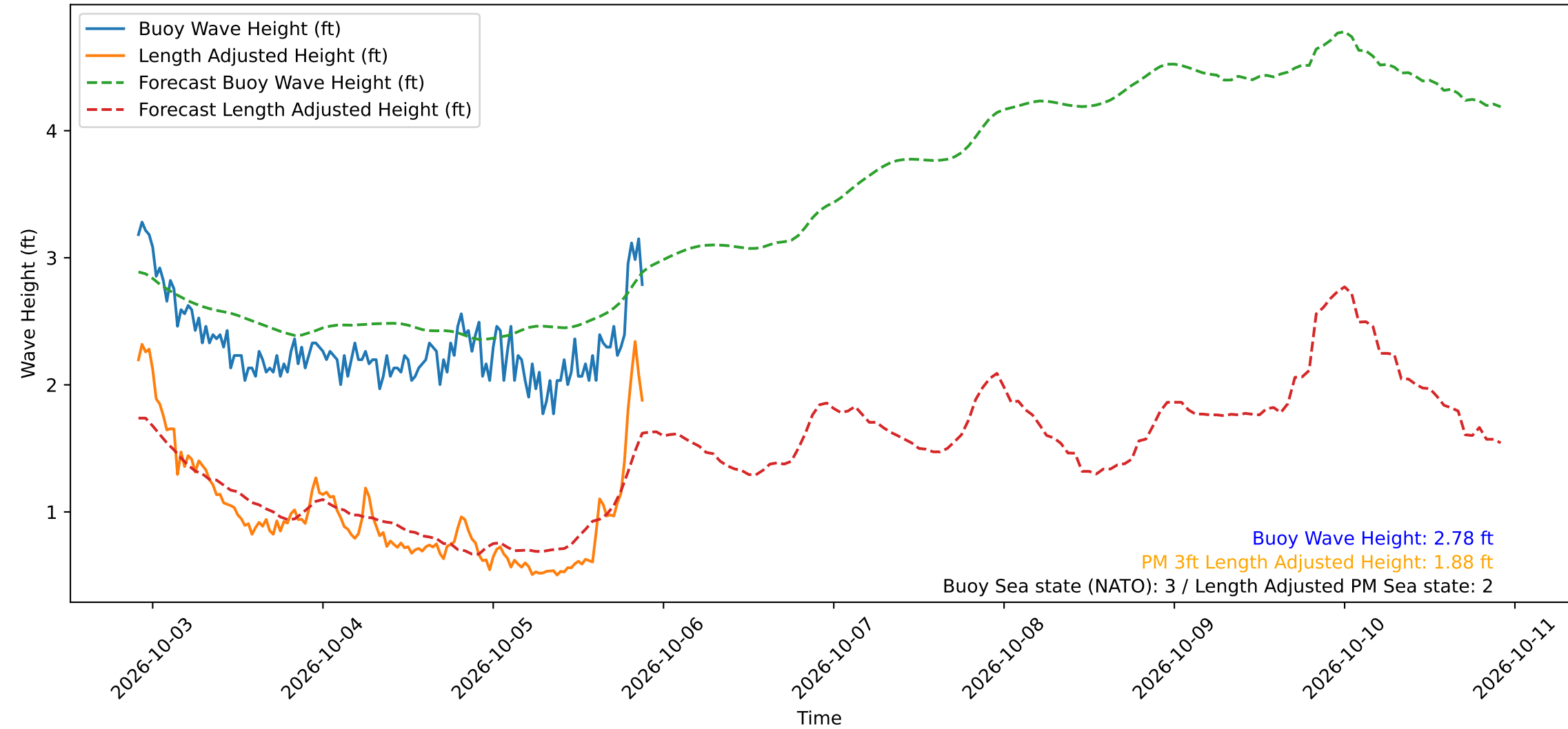
Wave Heights over Time for Green Beach at 2026-10-05 21:41:11
