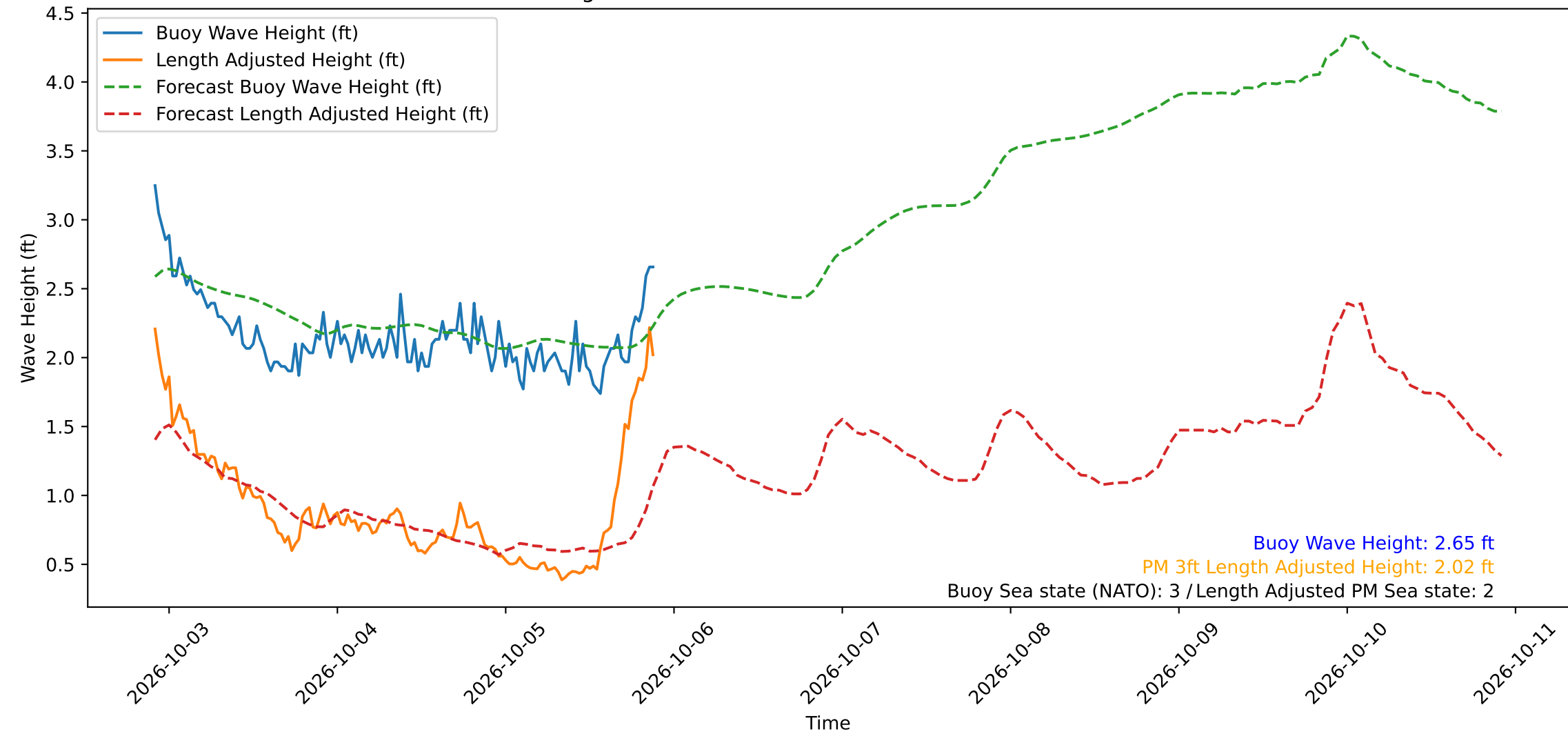
Wave Heights over Time for Red Beach at 2026-10-05 21:40:48
