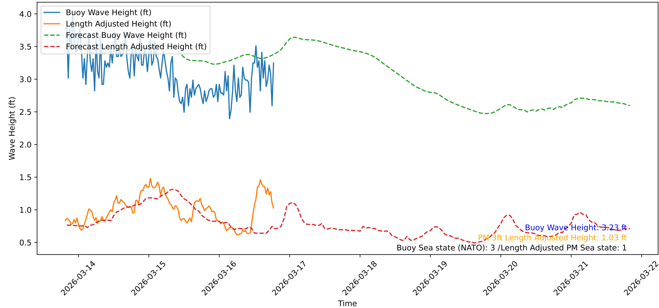
Wave Heights over Time for Oceanside Harbor at 2026-03-16 19:40:42
