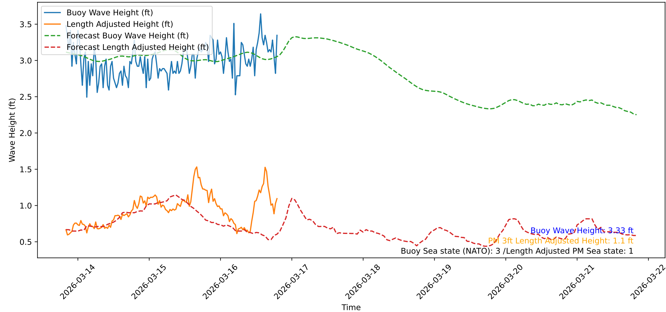
Wave Heights over Time for Red Beach at 2026-03-16 19:41:04
