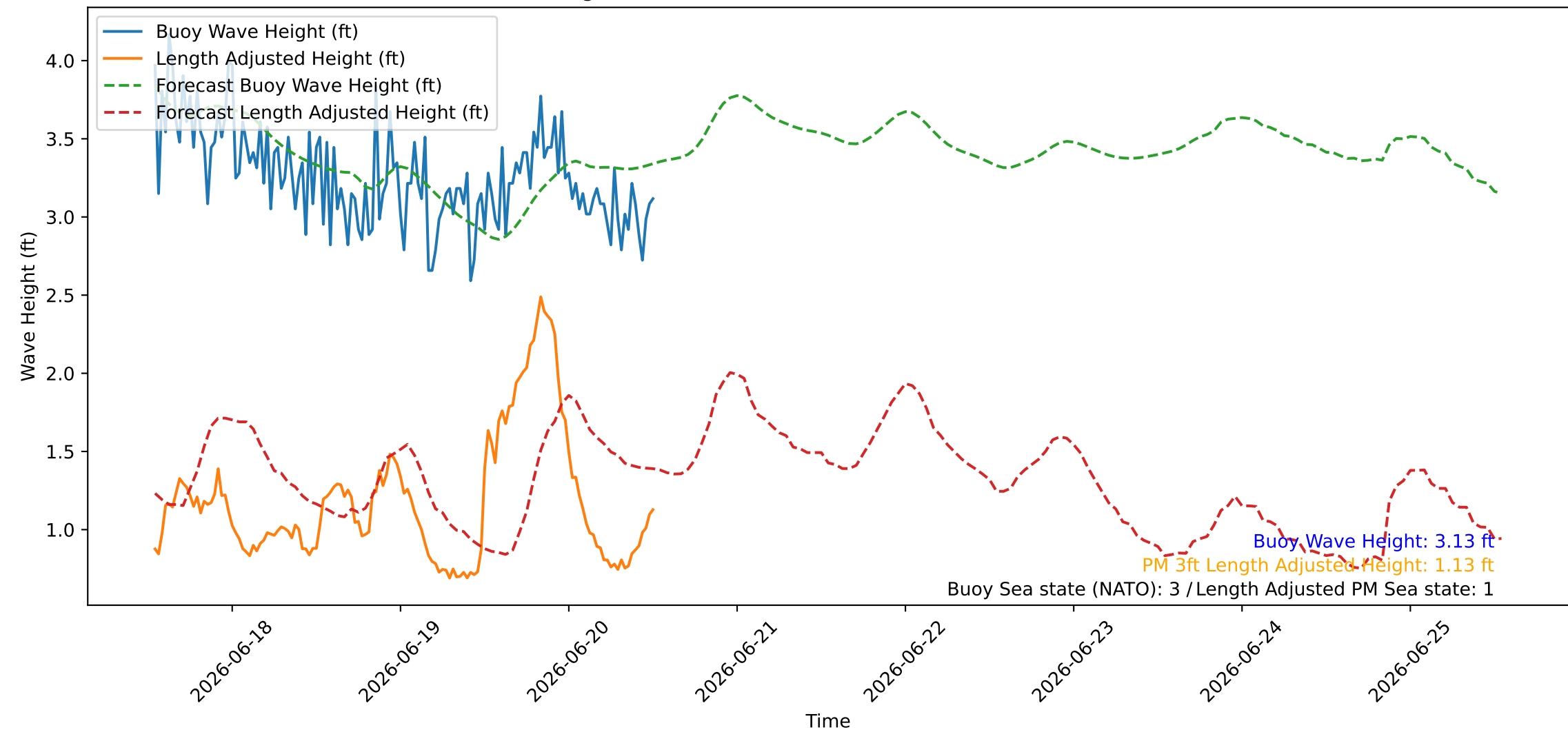
Wave Heights over Time for Red Beach at 2026-06-20 12:50:46
