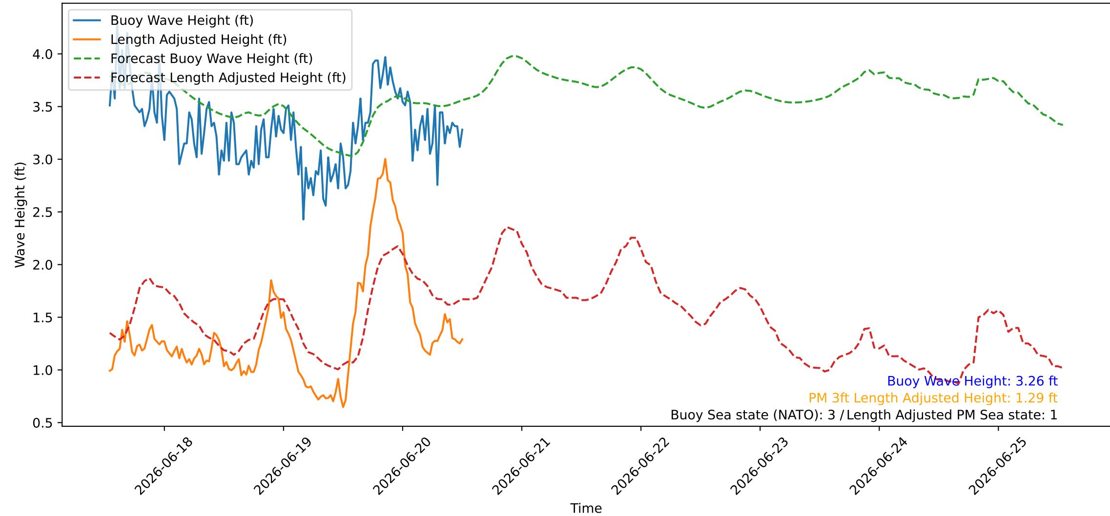
Wave Heights over Time for Green Beach at 2026-06-20 12:51:08
