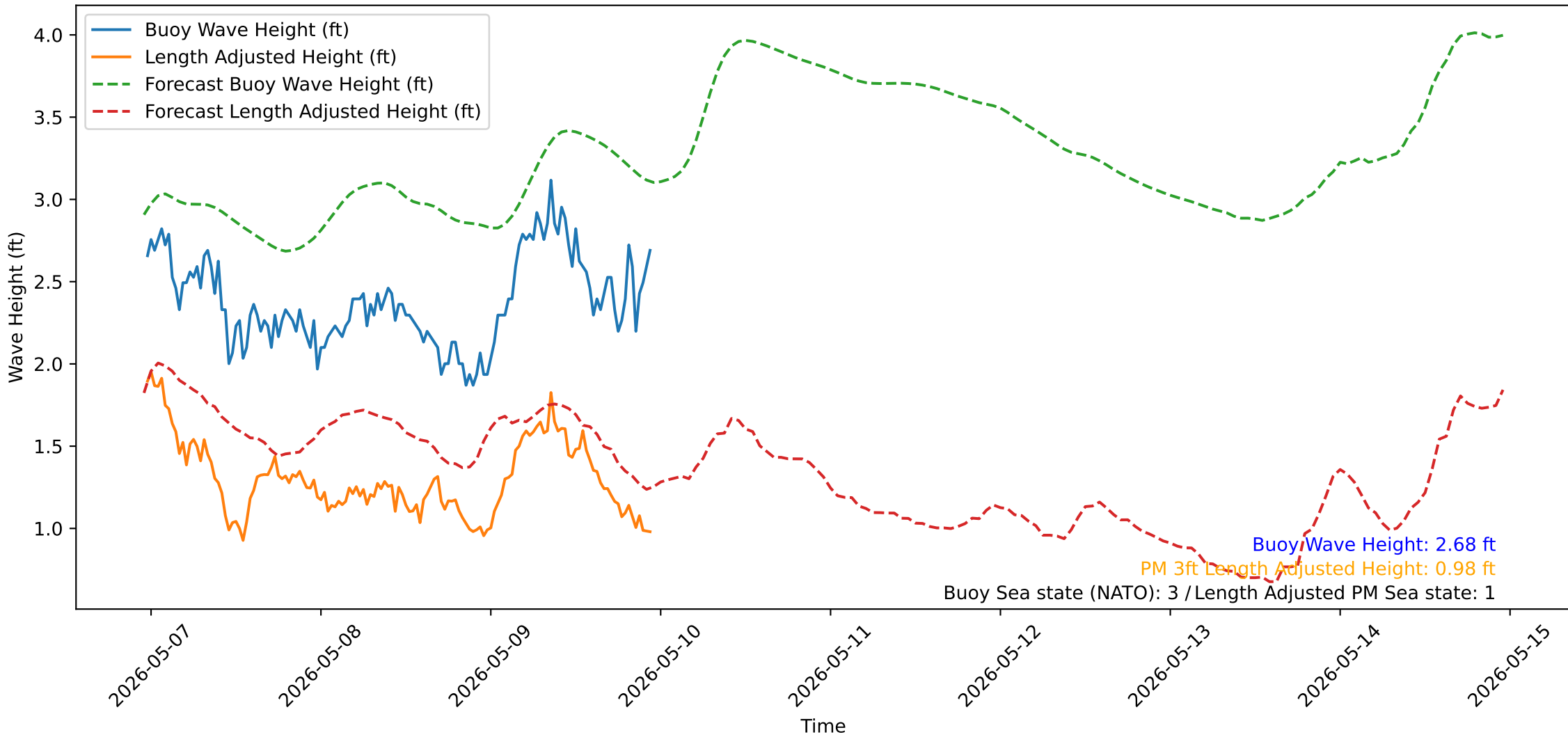
Wave Heights over Time for Oceanside Harbor at 2026-05-09 23:20:31
