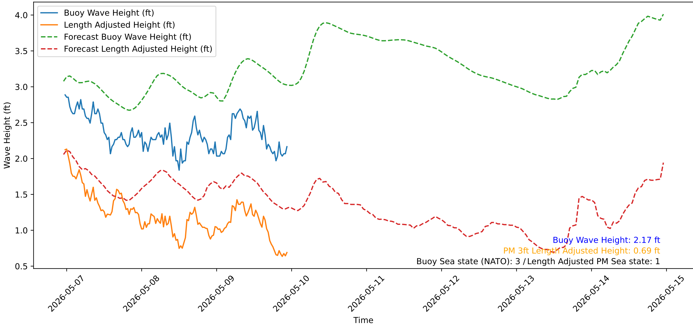
Wave Heights over Time for Green Beach at 2026-05-09 23:21:14
