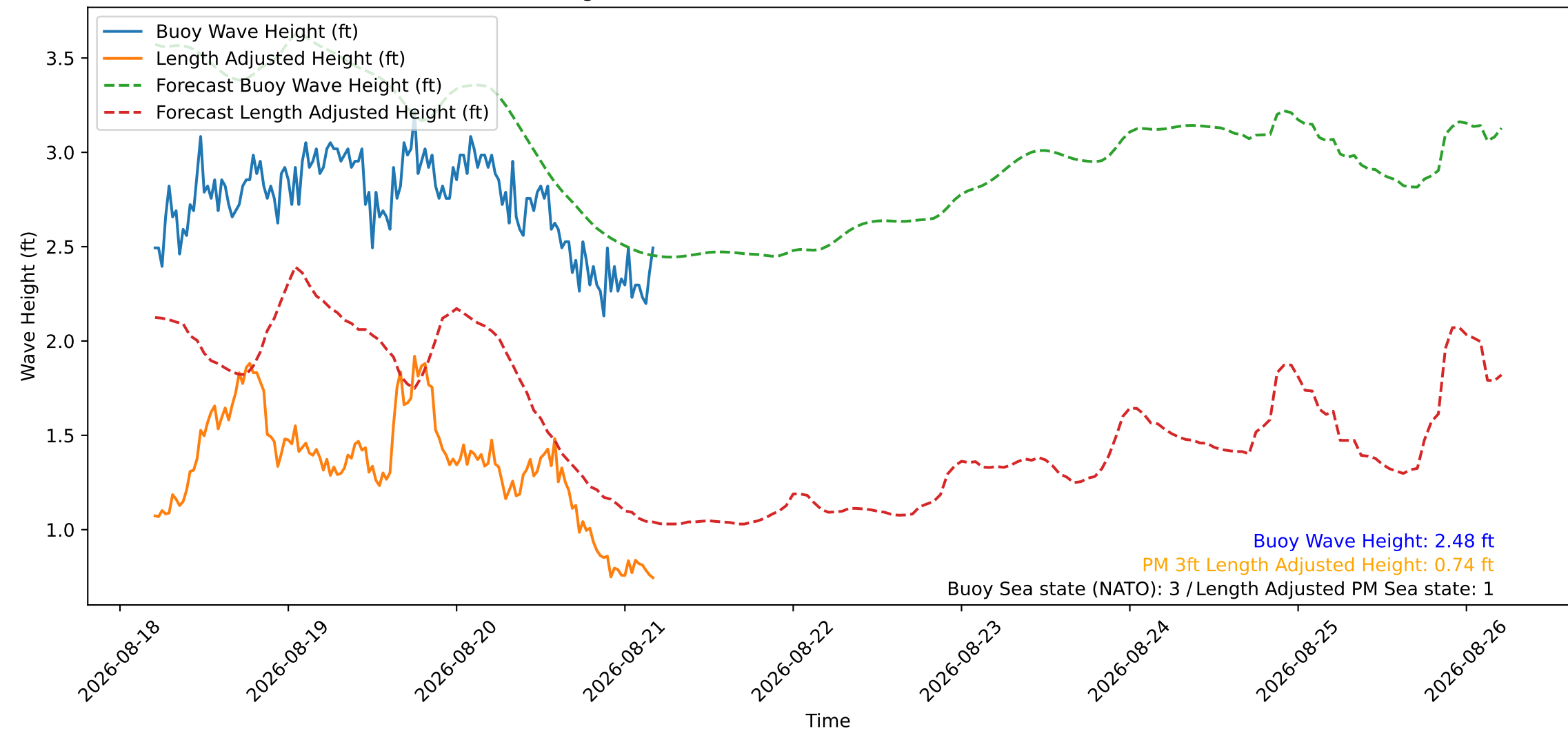
Wave Heights over Time for Red Beach at 2026-08-21 04:40:46
