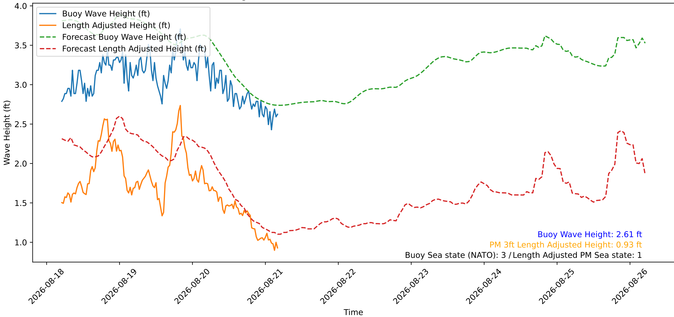
Wave Heights over Time for Green Beach at 2026-08-21 04:41:08
