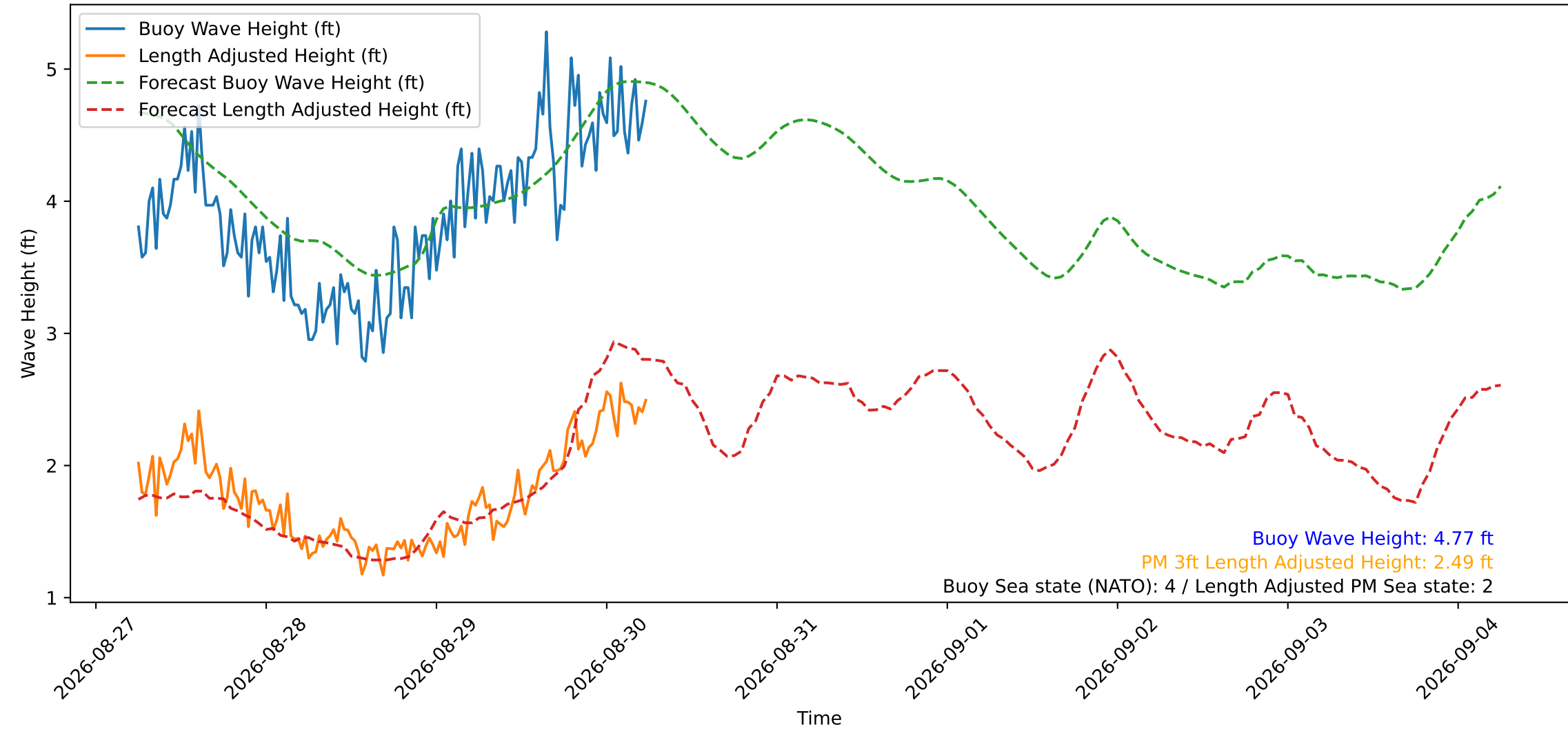
Wave Heights over Time for Oceanside Harbor at 2026-08-30 06:10:30
