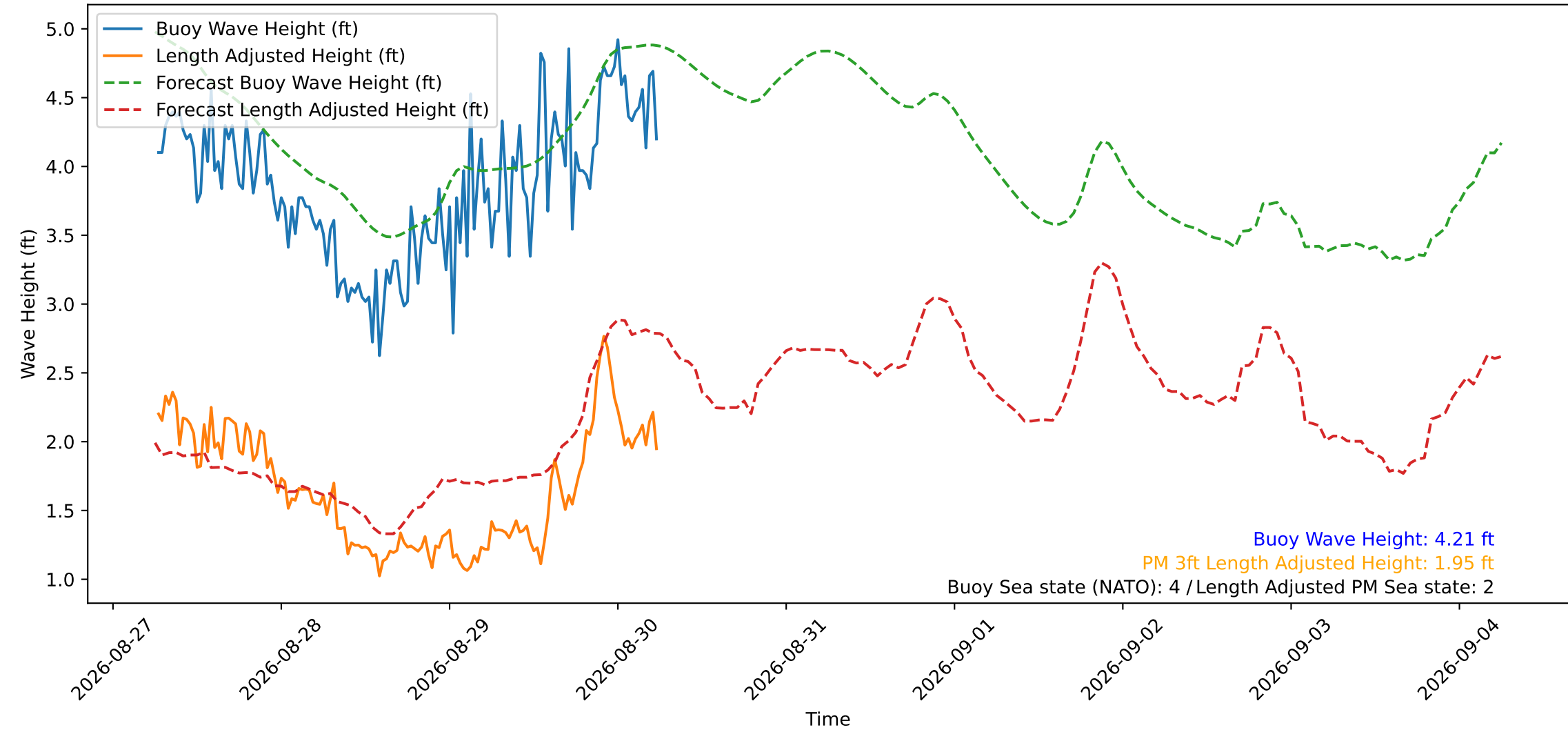
Wave Heights over Time for Green Beach at 2026-08-30 06:11:12
