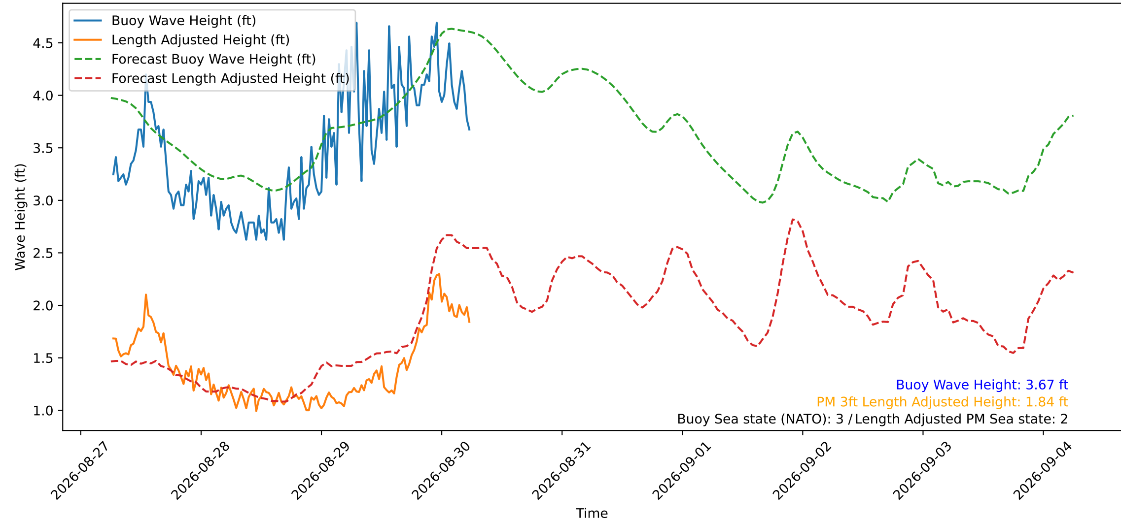
Wave Heights over Time for Red Beach at 2026-08-30 06:10:50
