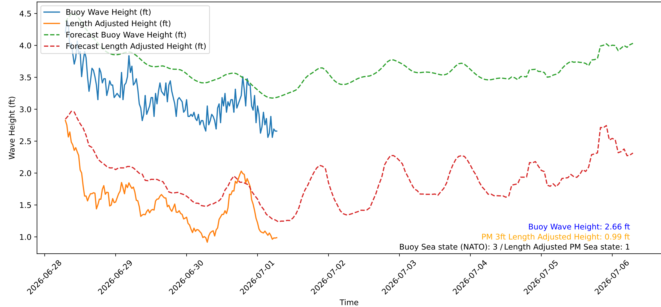
Wave Heights over Time for Green Beach at 2026-07-01 07:11:08
