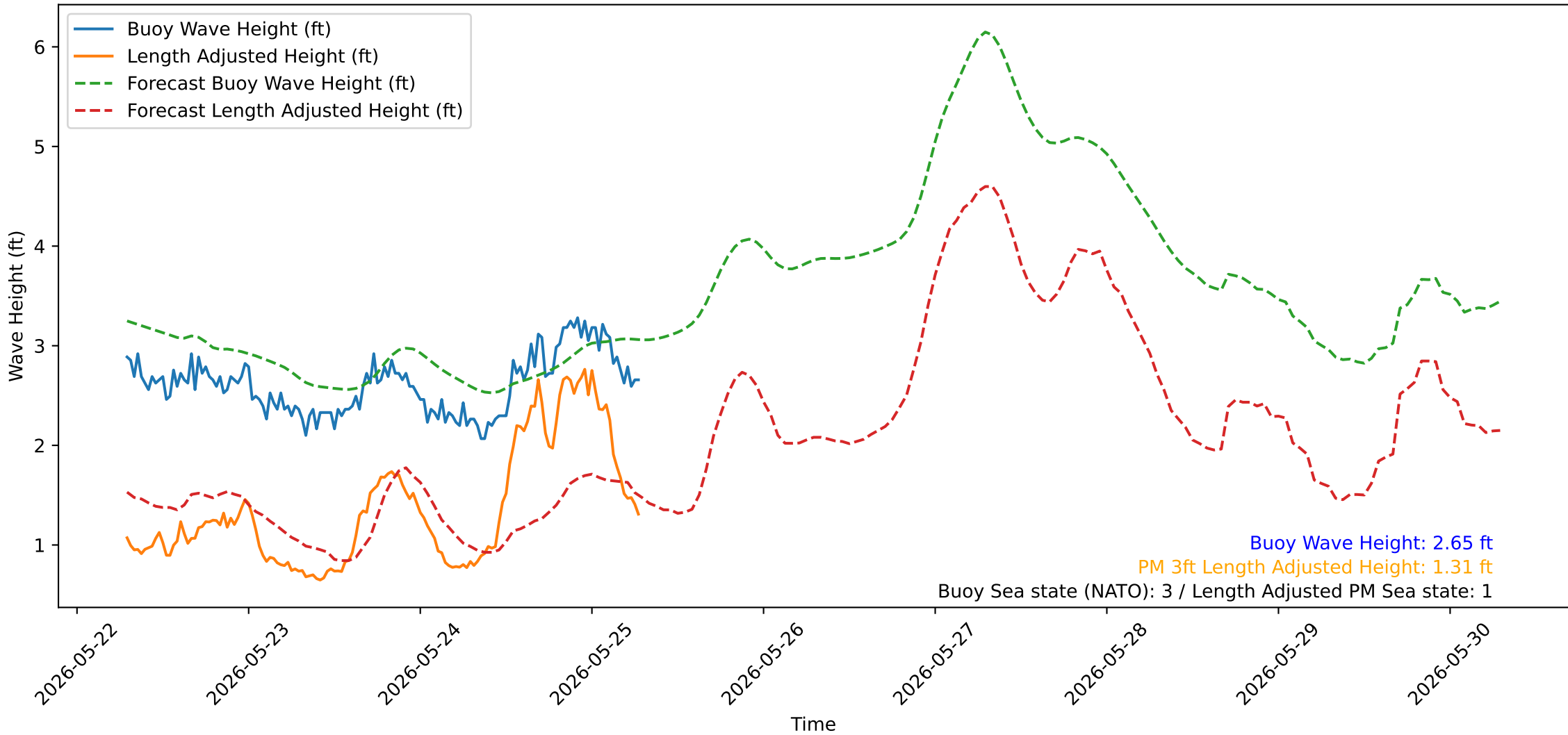
Wave Heights over Time for Green Beach at 2026-05-25 07:11:13
