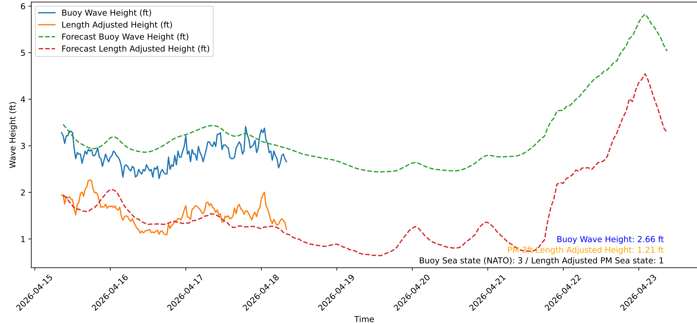
Wave Heights over Time for Oceanside Harbor at 2026-04-18 08:40:31
