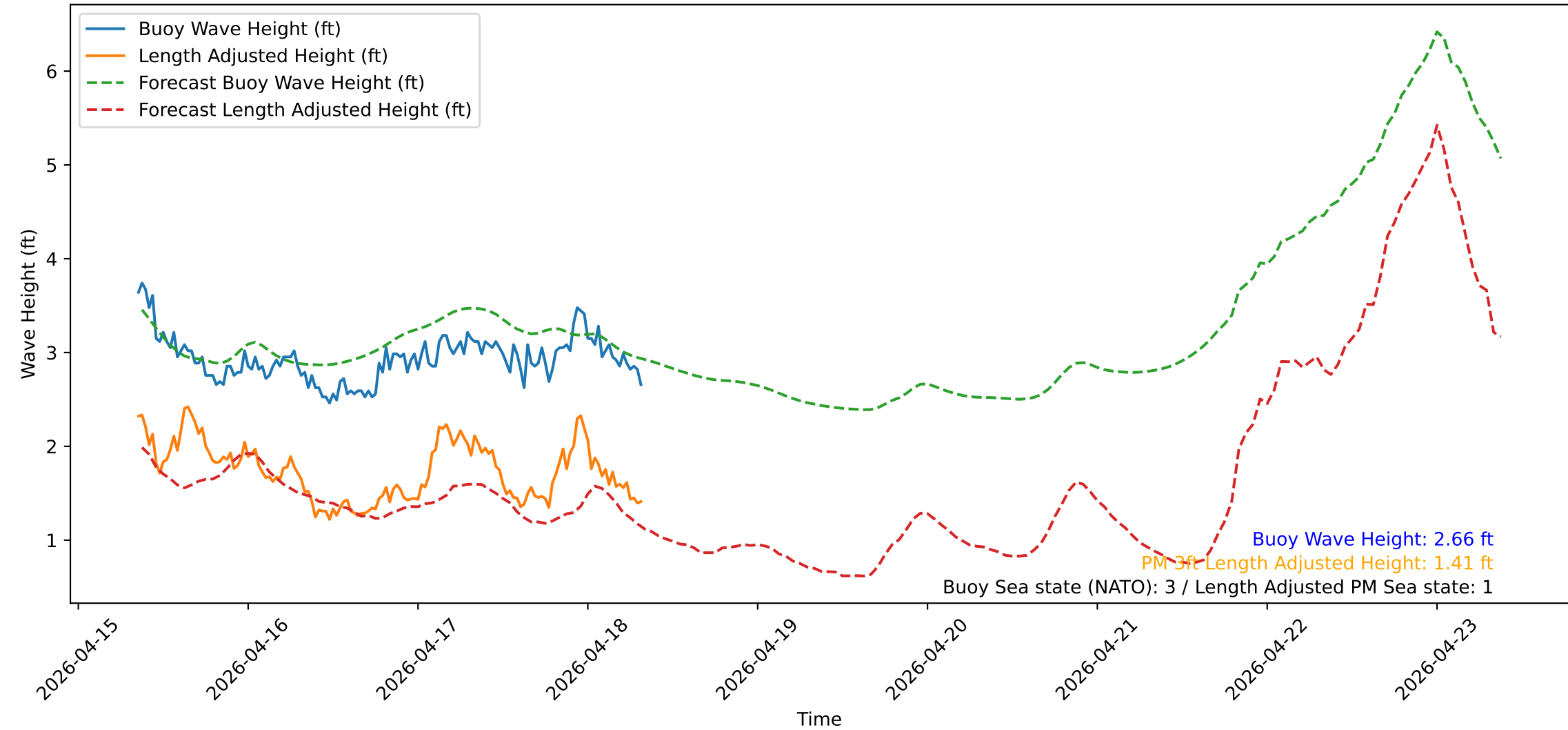
Wave Heights over Time for Green Beach at 2026-04-18 08:41:12
