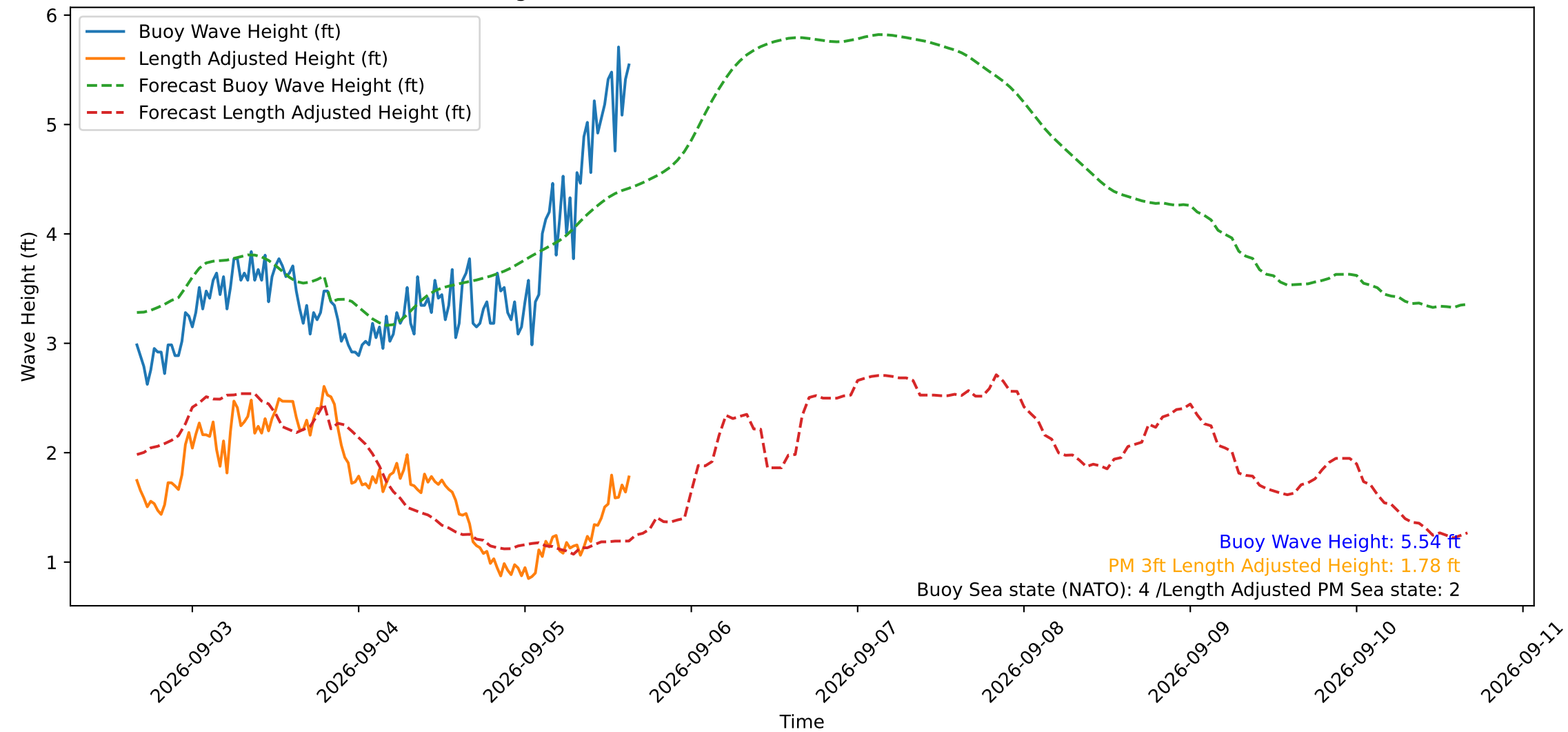
Wave Heights over Time for Oceanside Harbor at 2026-09-05 15:50:30
