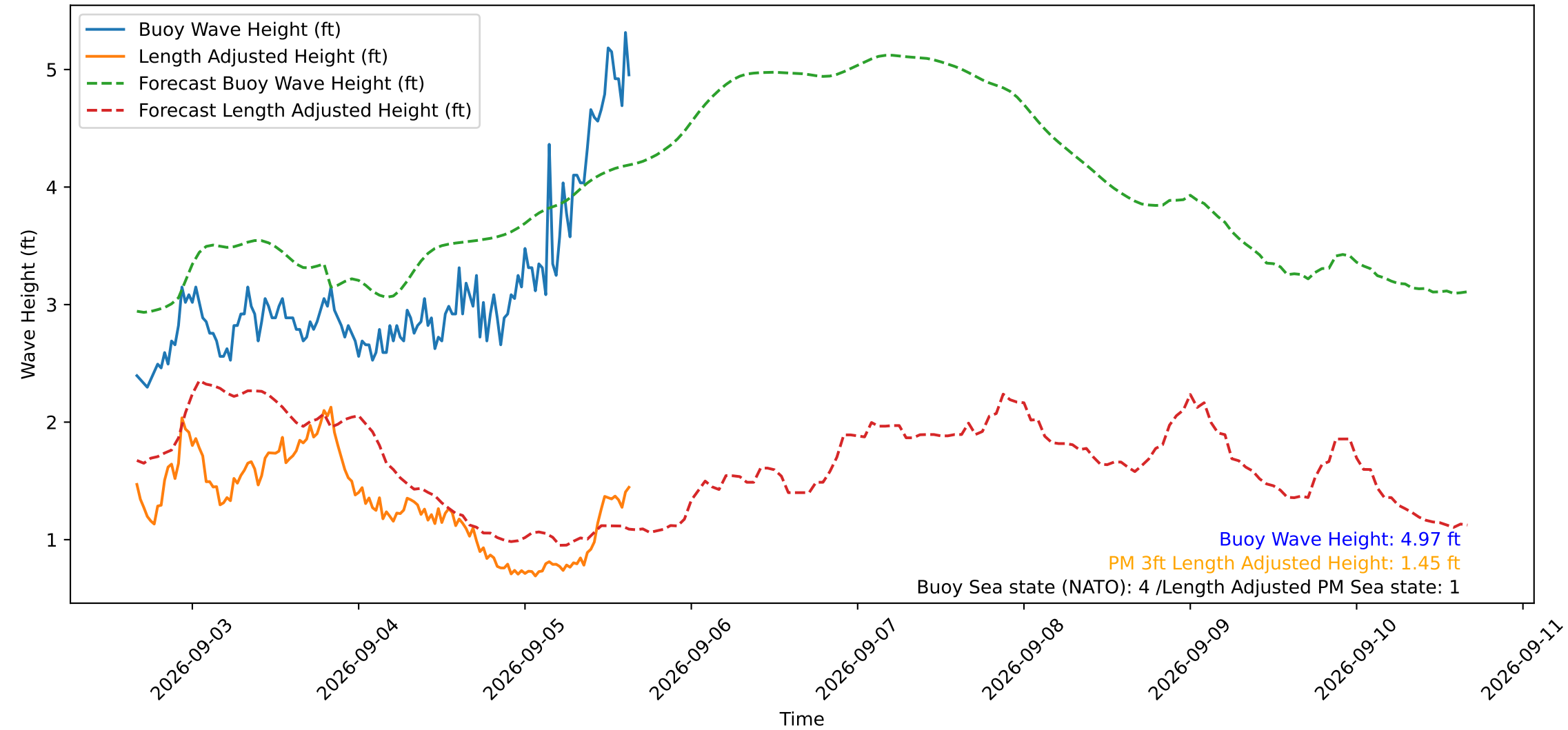
Wave Heights over Time for Red Beach at 2026-09-05 15:50:51
