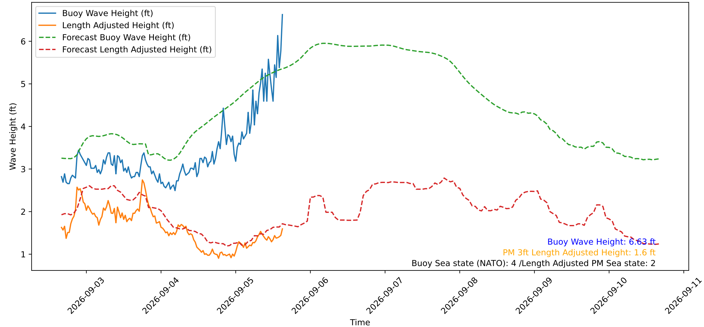
Wave Heights over Time for Green Beach at 2026-09-05 15:51:15
