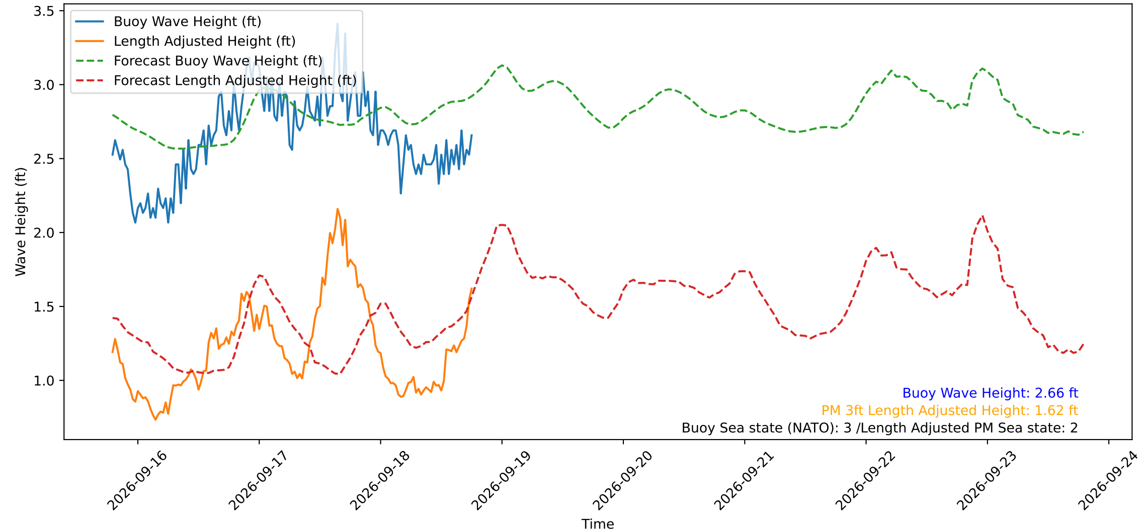
Wave Heights over Time for Red Beach at 2026-09-18 18:40:49
