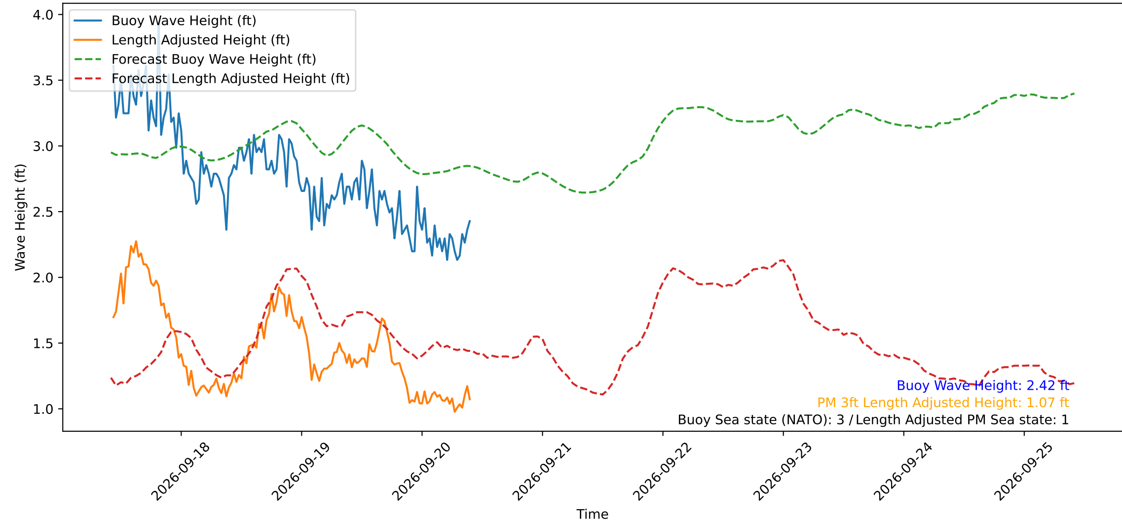
Wave Heights over Time for Oceanside Harbor at 2026-09-20 10:20:30
