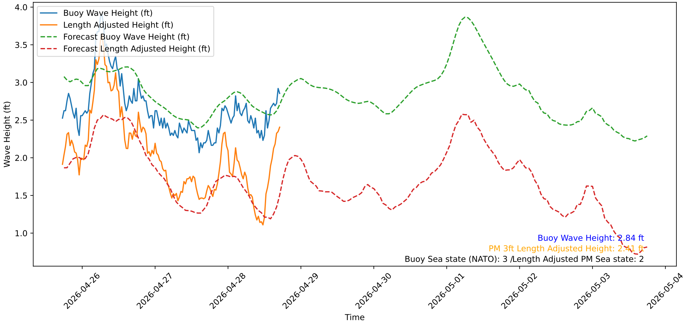
Wave Heights over Time for Oceanside Harbor at 2026-04-28 17:30:32
