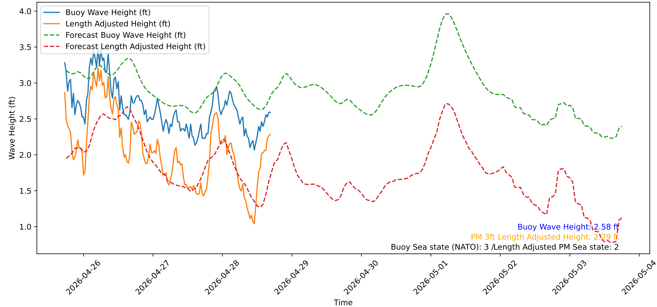
Wave Heights over Time for Green Beach at 2026-04-28 17:31:14
