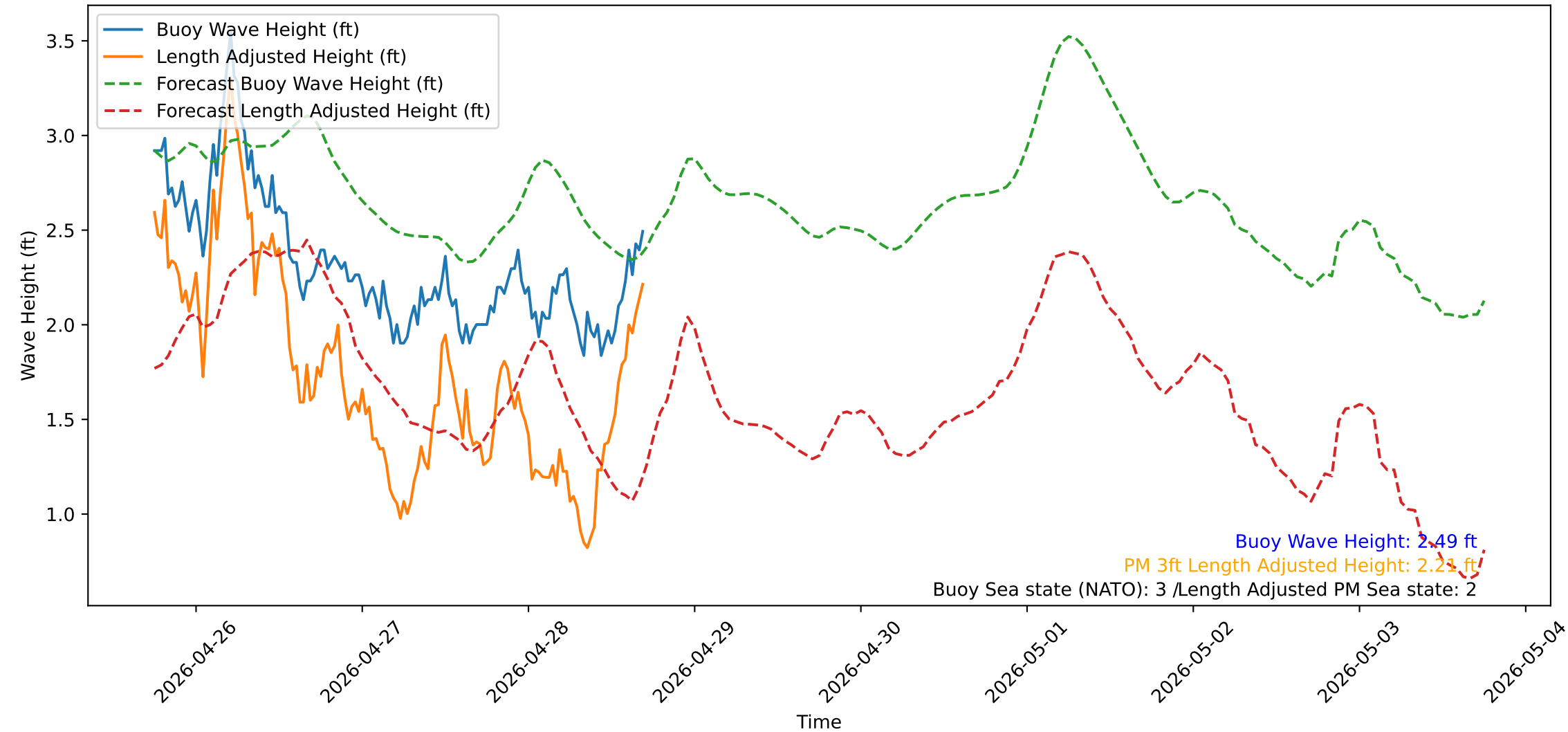
Wave Heights over Time for Red Beach at 2026-04-28 17:30:51
