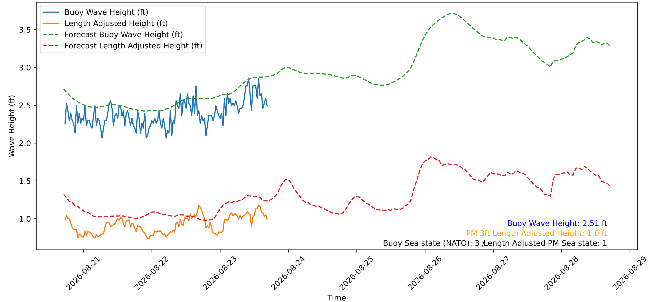
Wave Heights over Time for Red Beach at 2026-08-23 17:20:51
