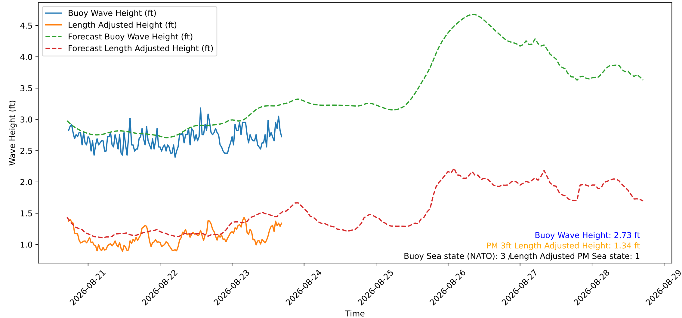
Wave Heights over Time for Green Beach at 2026-08-23 17:21:14
