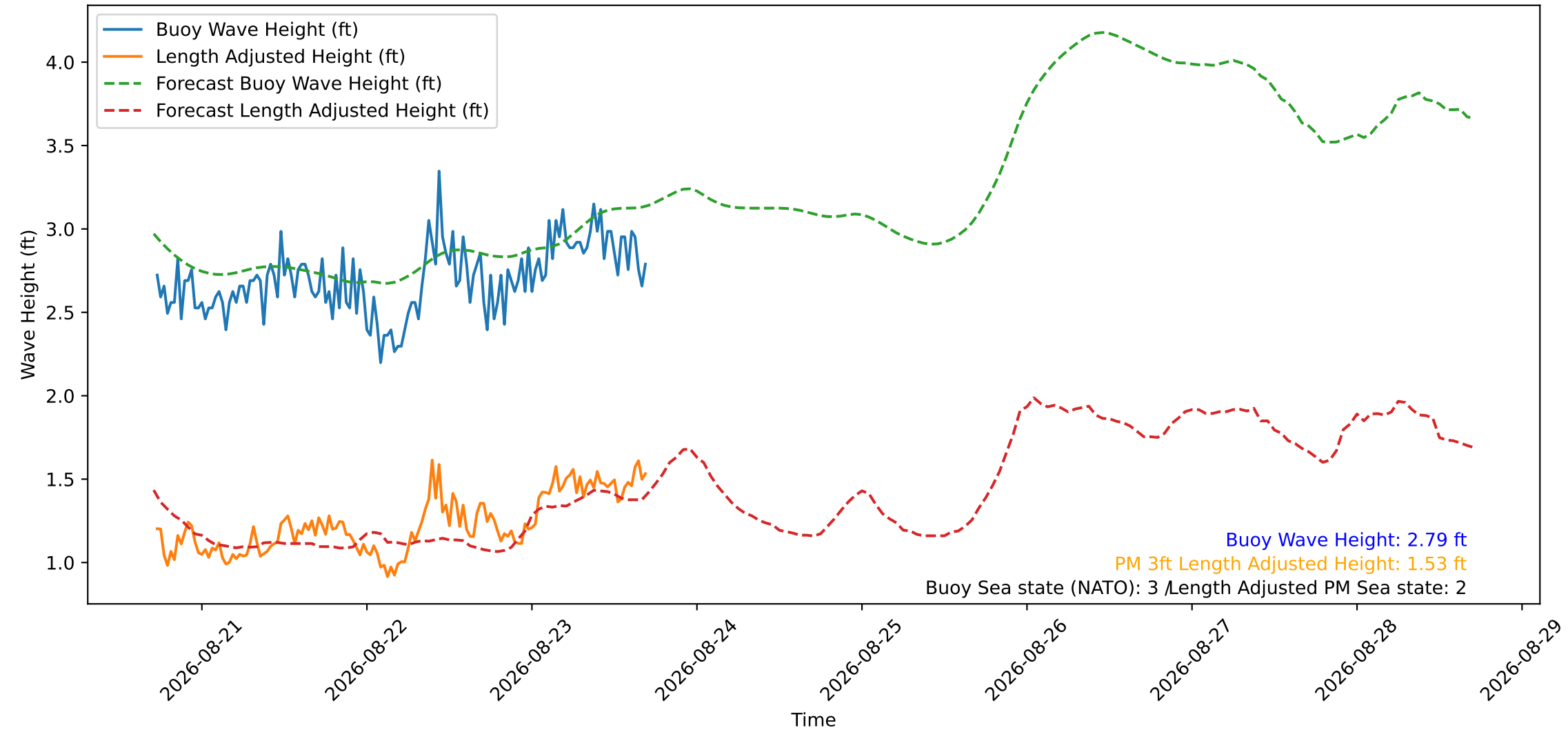
Wave Heights over Time for Oceanside Harbor at 2026-08-23 17:20:29
