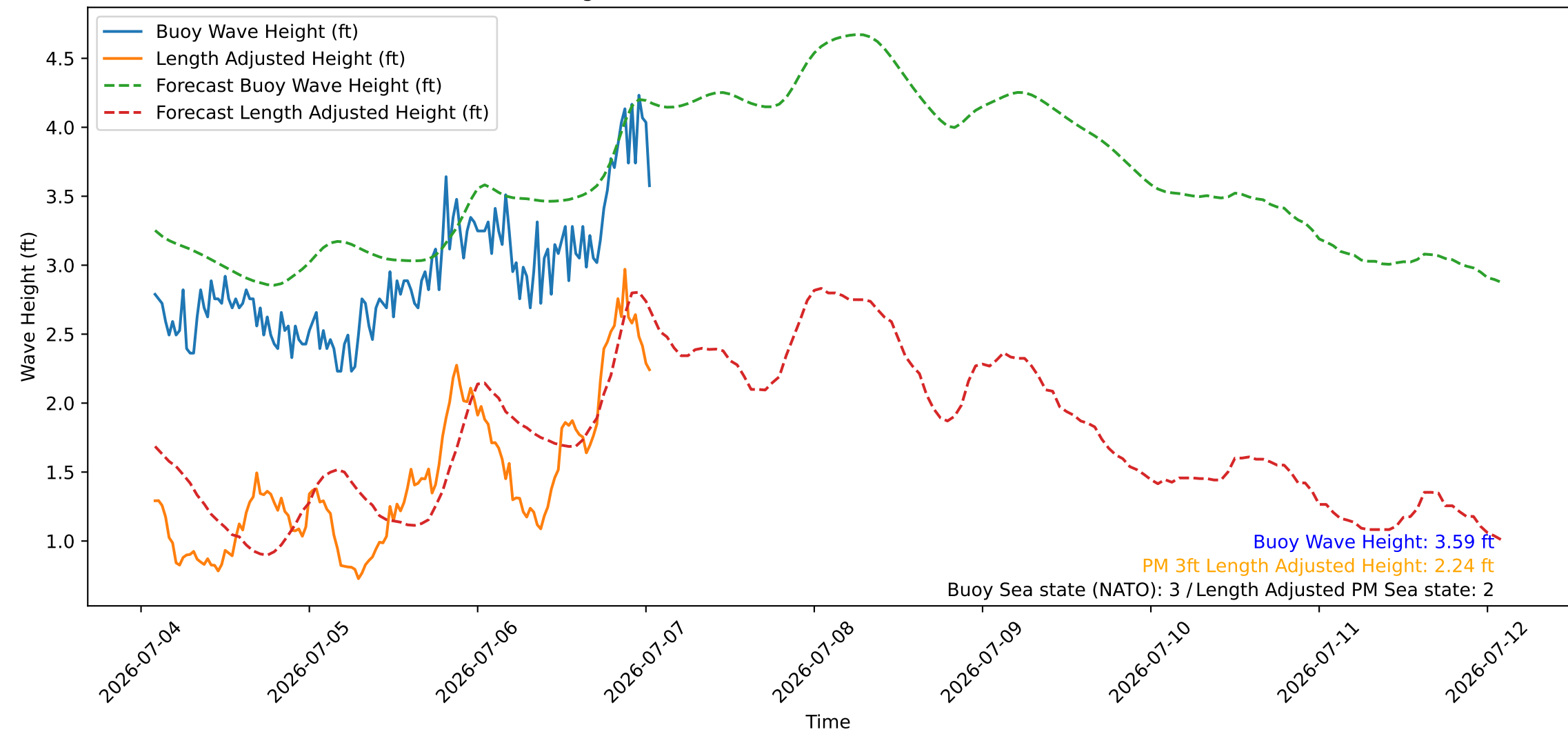
Wave Heights over Time for Red Beach at 2026-07-07 01:30:46
