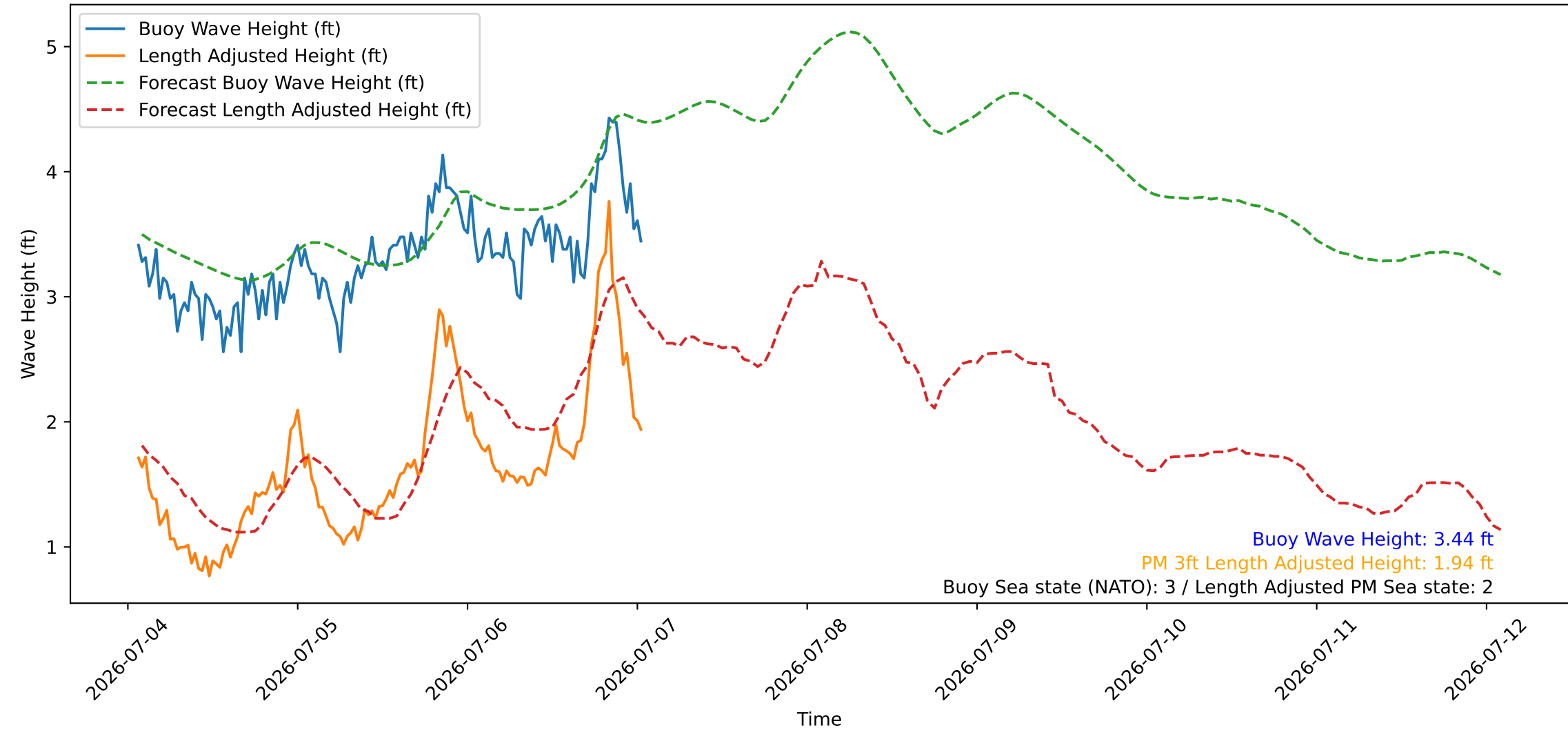
Wave Heights over Time for Green Beach at 2026-07-07 01:31:09
