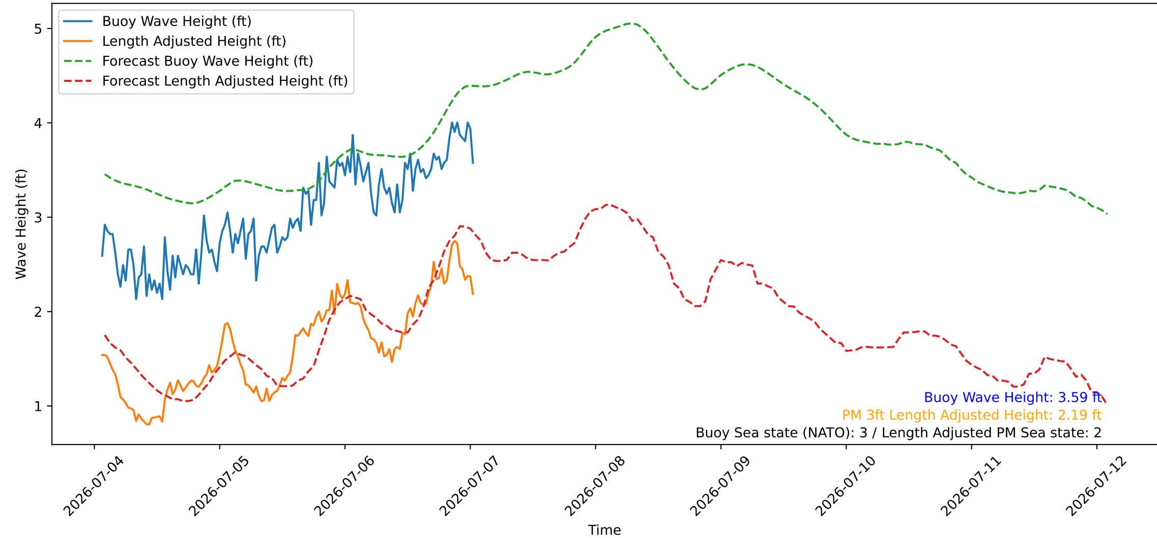
Wave Heights over Time for Oceanside Harbor at 2026-07-07 01:30:26
