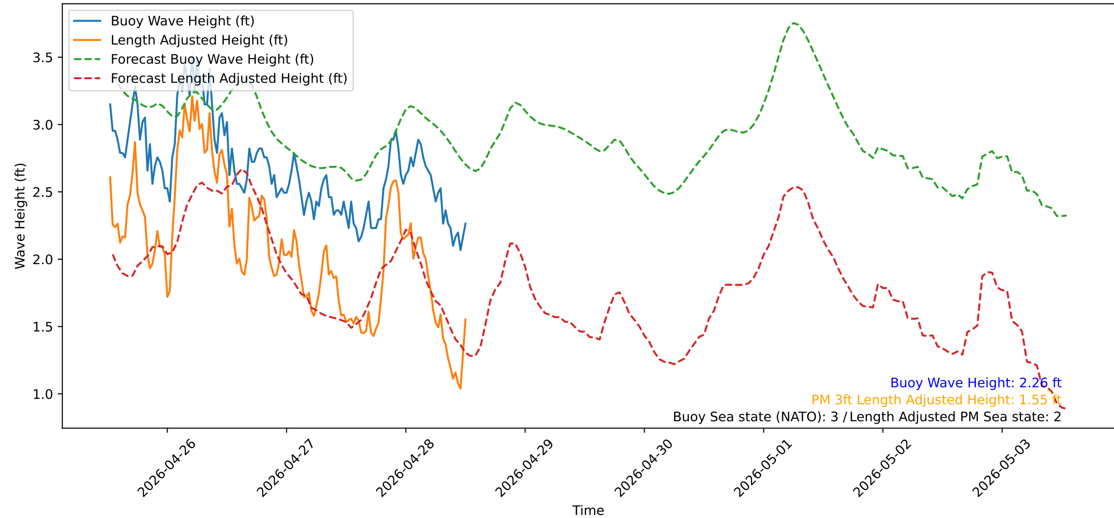
Wave Heights over Time for Green Beach at 2026-04-28 12:41:14
