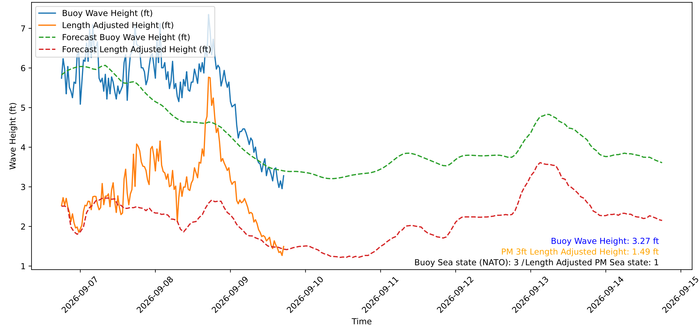
Wave Heights over Time for Oceanside Harbor at 2026-09-09 18:10:29
