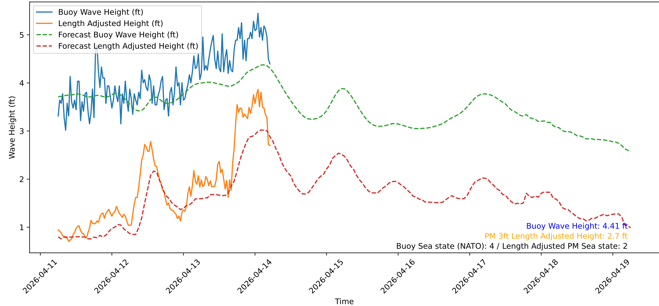
Wave Heights over Time for Oceanside Harbor at 2026-04-14 06:00:31
