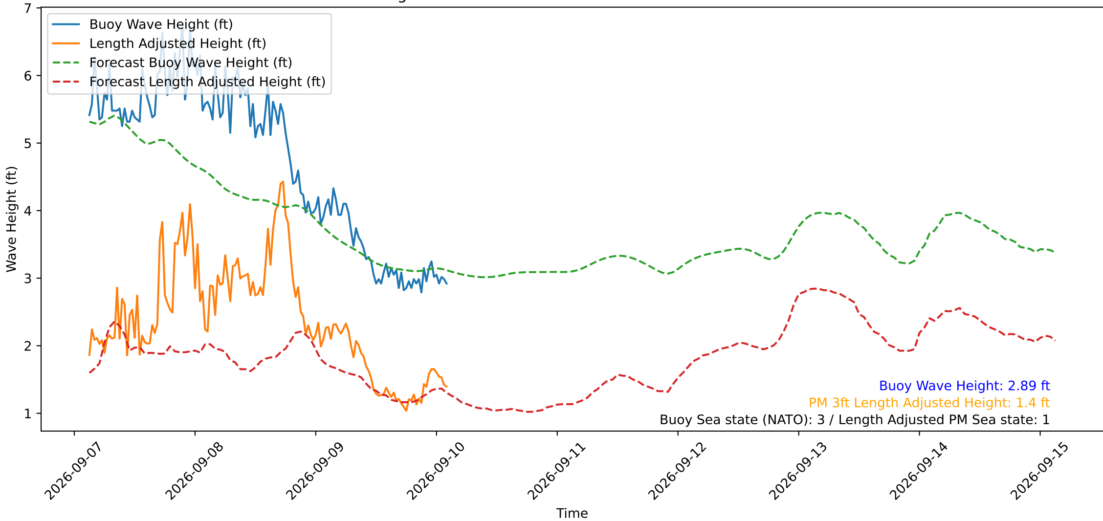
Wave Heights over Time for Red Beach at 2026-09-10 02:40:49
