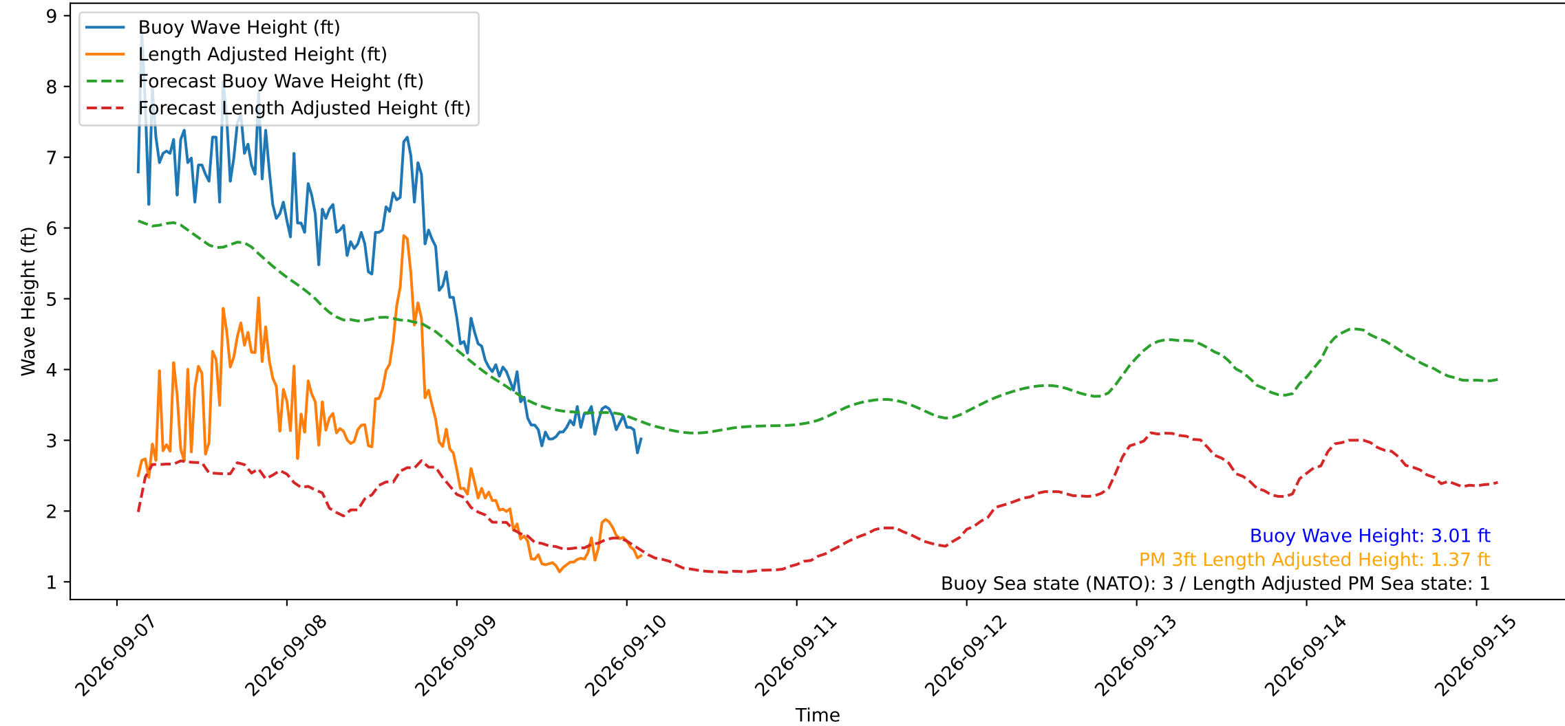
Wave Heights over Time for Green Beach at 2026-09-10 02:41:11
