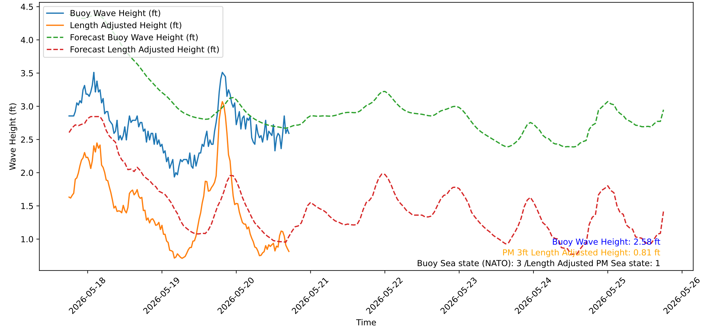
Wave Heights over Time for Red Beach at 2026-05-20 17:40:51
