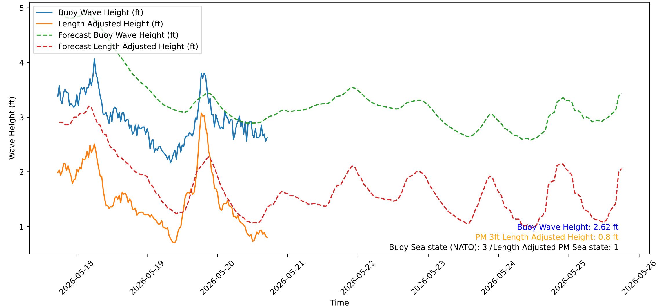
Wave Heights over Time for Green Beach at 2026-05-20 17:41:14
