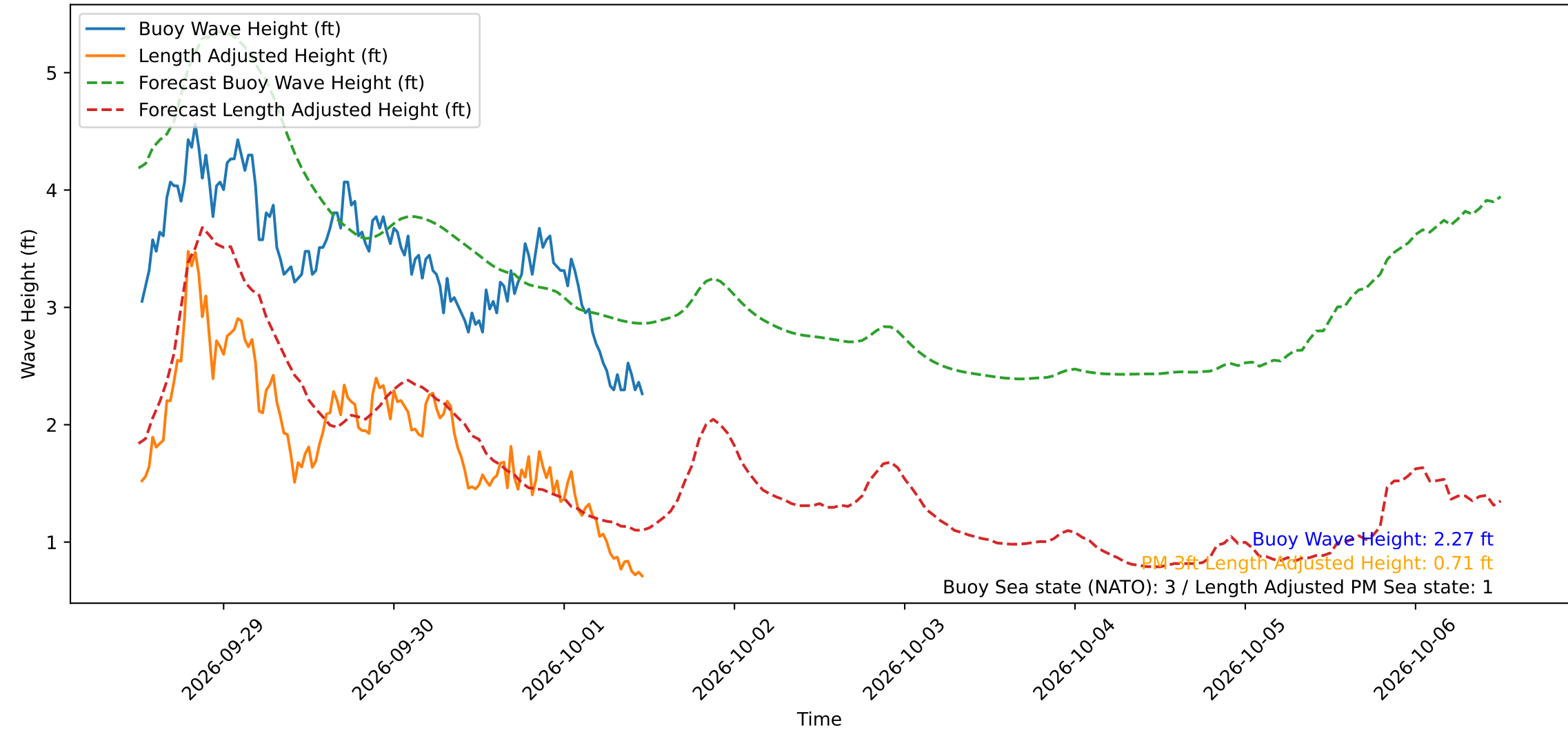
Wave Heights over Time for Green Beach at 2026-10-01 12:01:13
