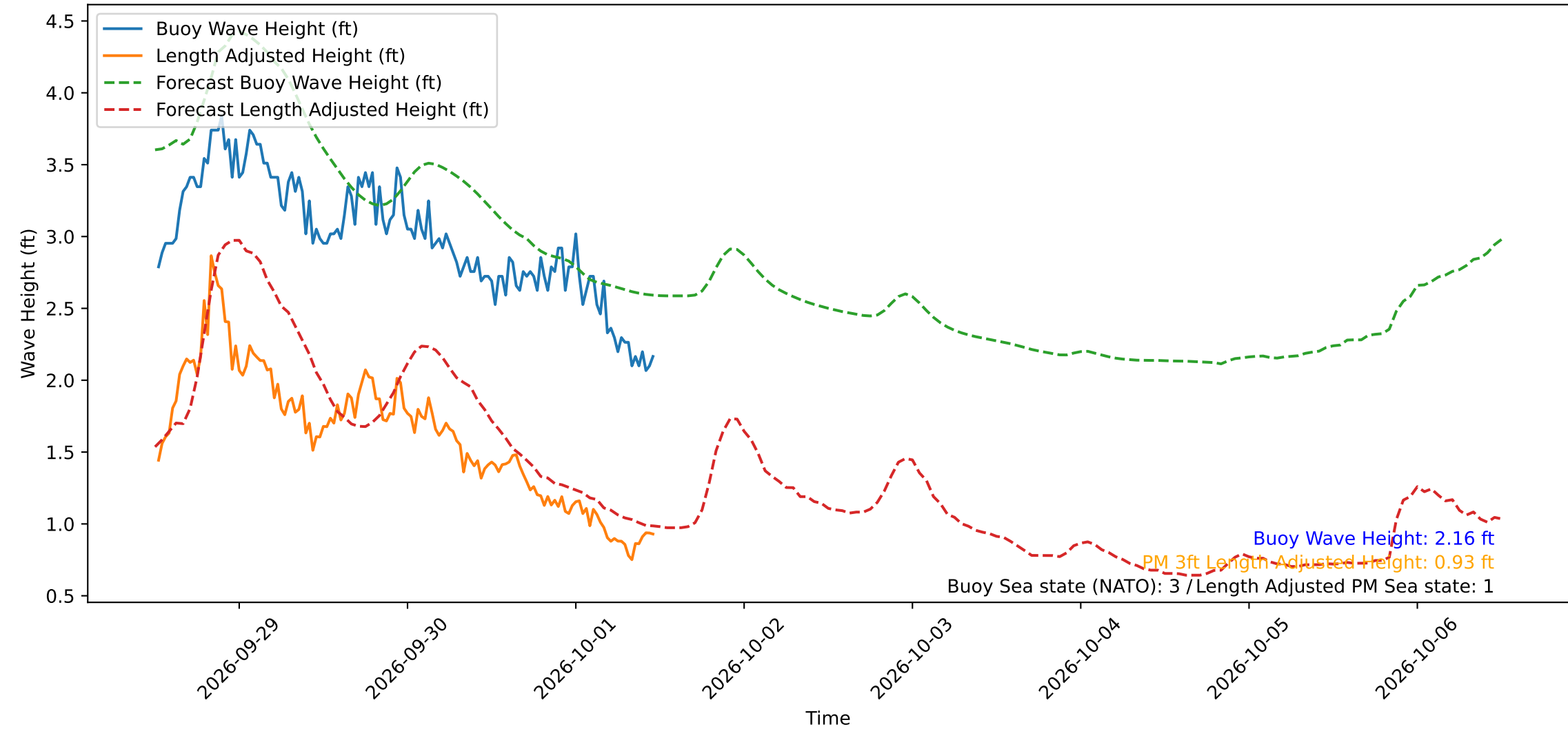
Wave Heights over Time for Red Beach at 2026-10-01 12:00:50
