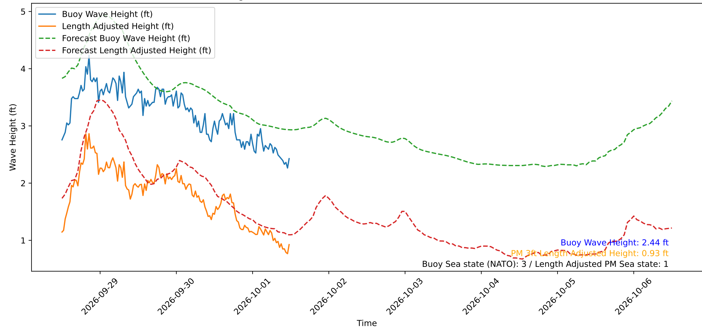
Wave Heights over Time for Oceanside Harbor at 2026-10-01 12:00:30
