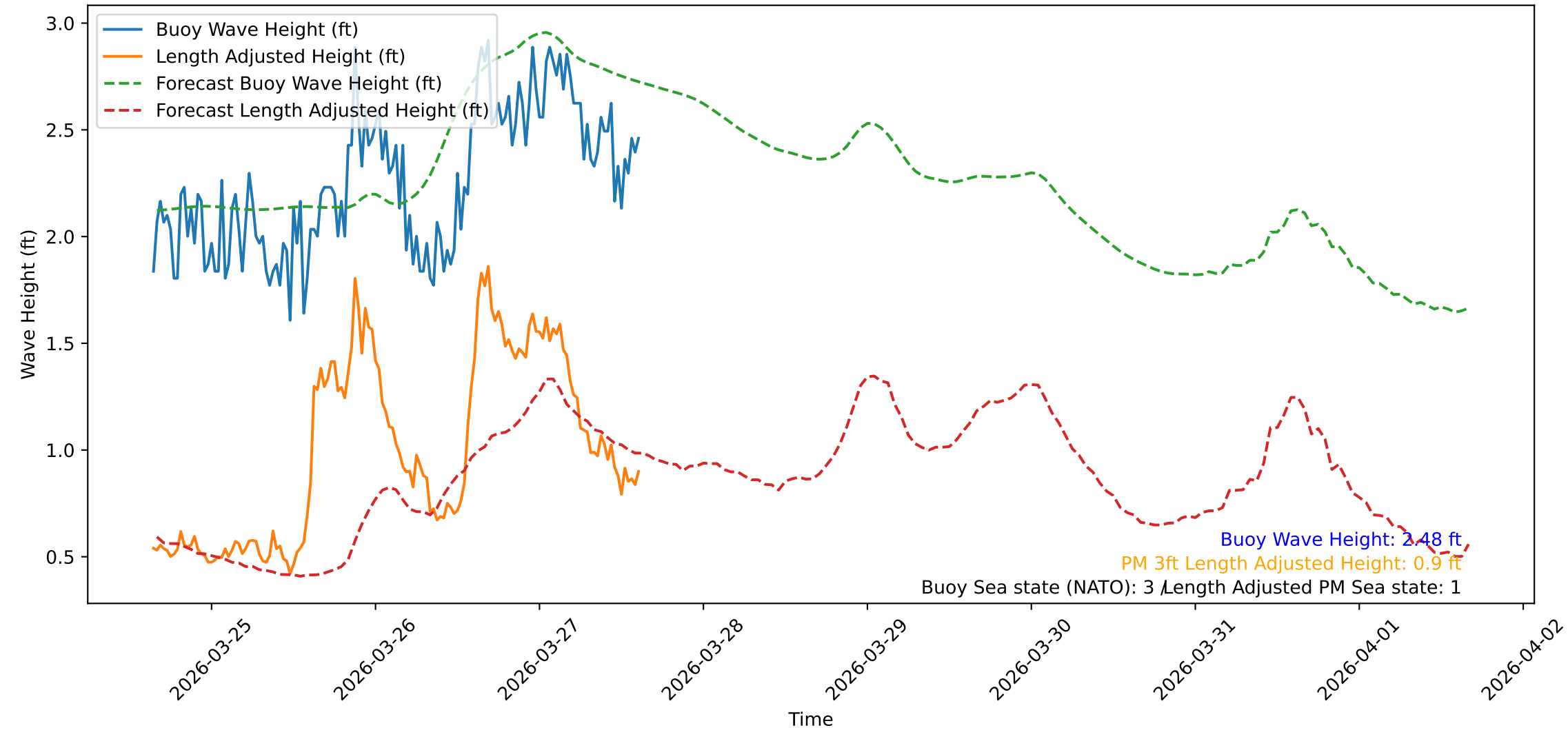
Wave Heights over Time for Oceanside Harbor at 2026-03-27 15:40:31
