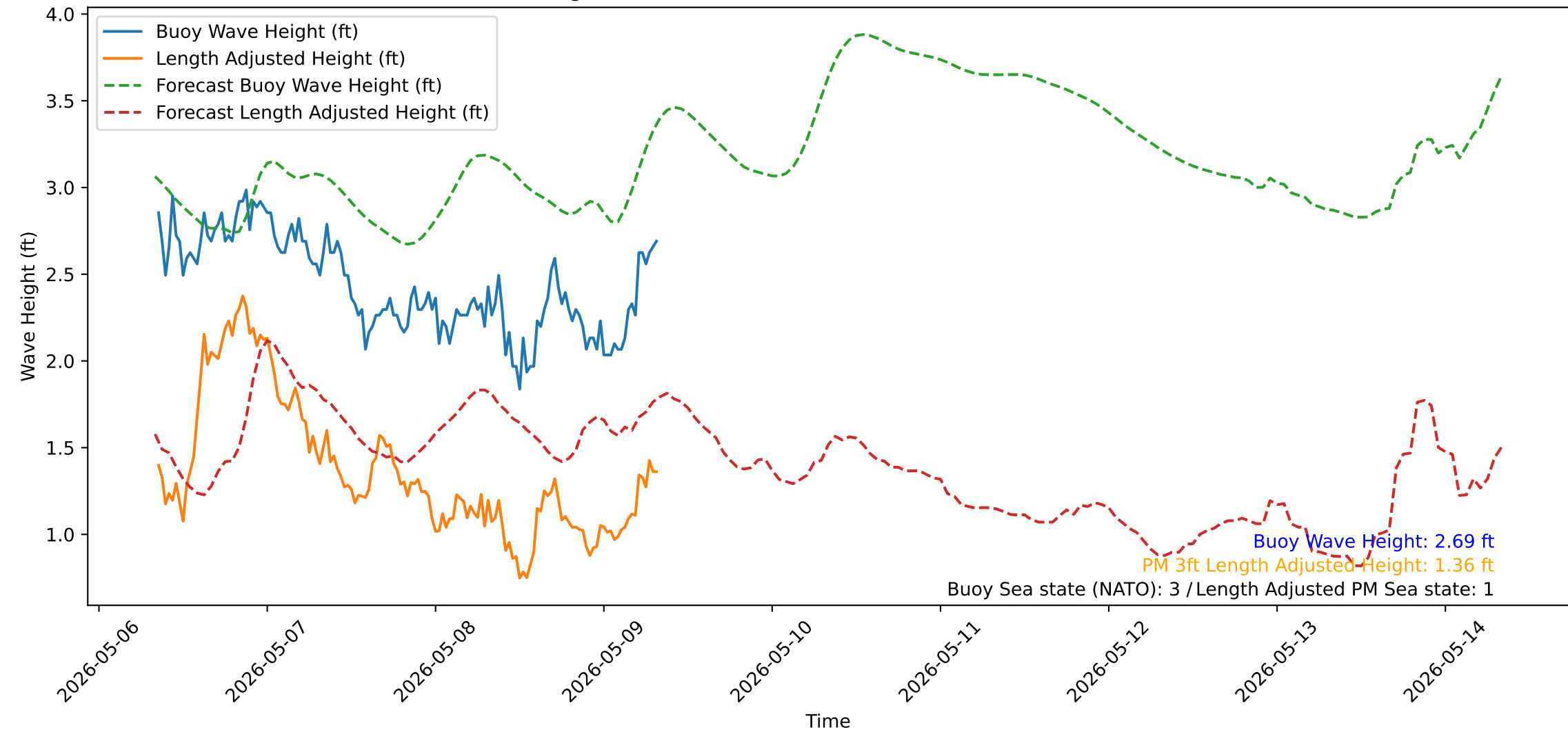
Wave Heights over Time for Green Beach at 2026-05-09 08:21:14
