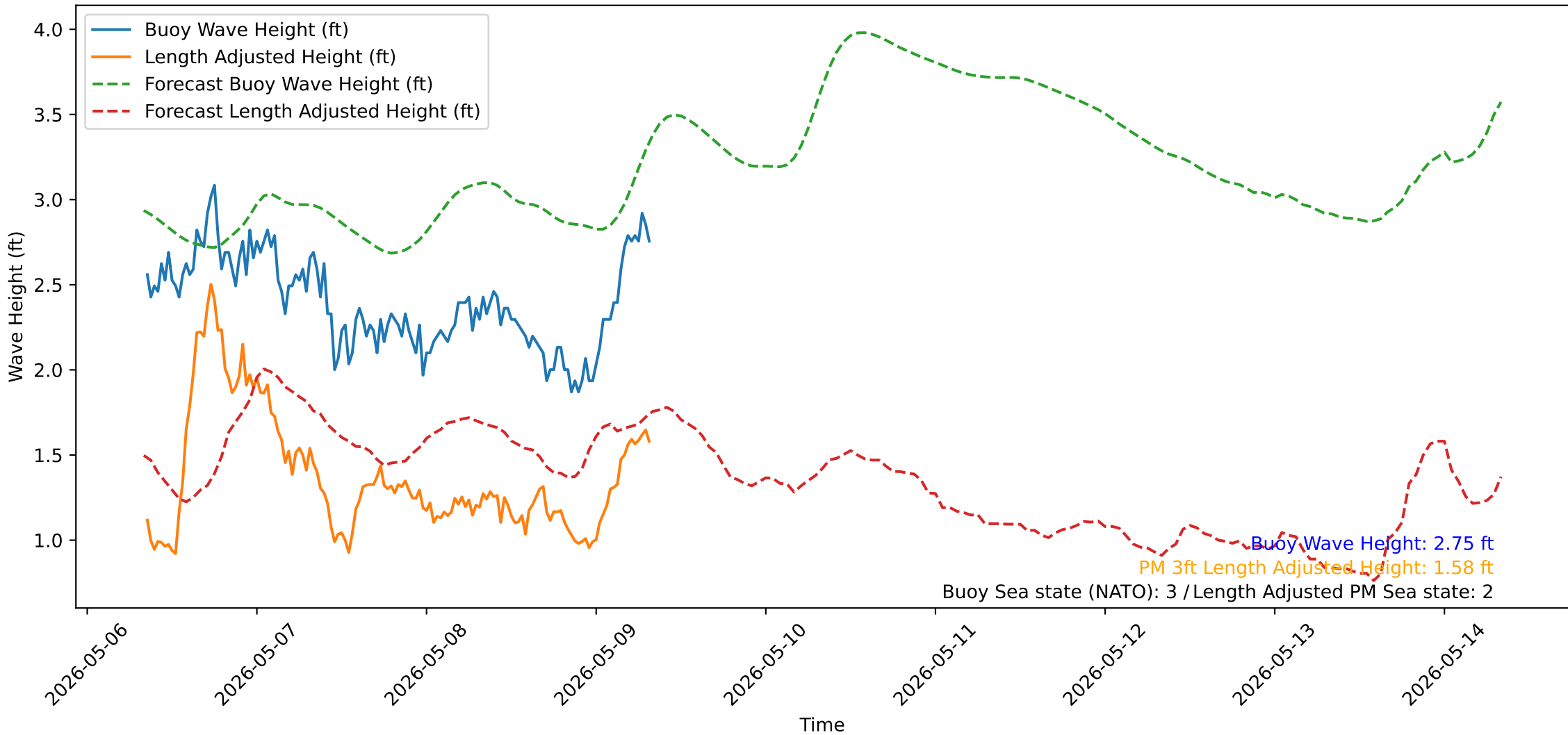
Wave Heights over Time for Oceanside Harbor at 2026-05-09 08:20:31
