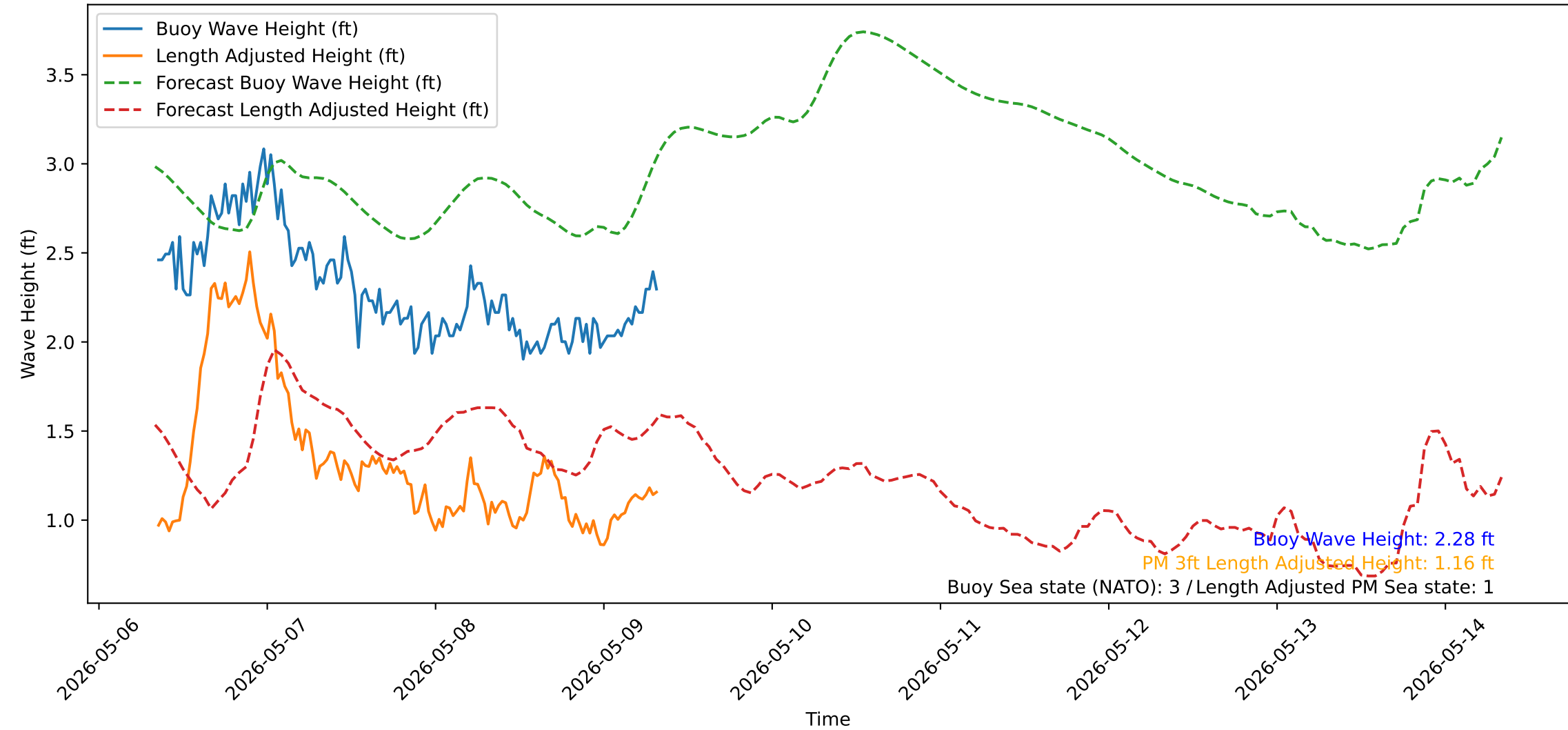
Wave Heights over Time for Red Beach at 2026-05-09 08:20:51
