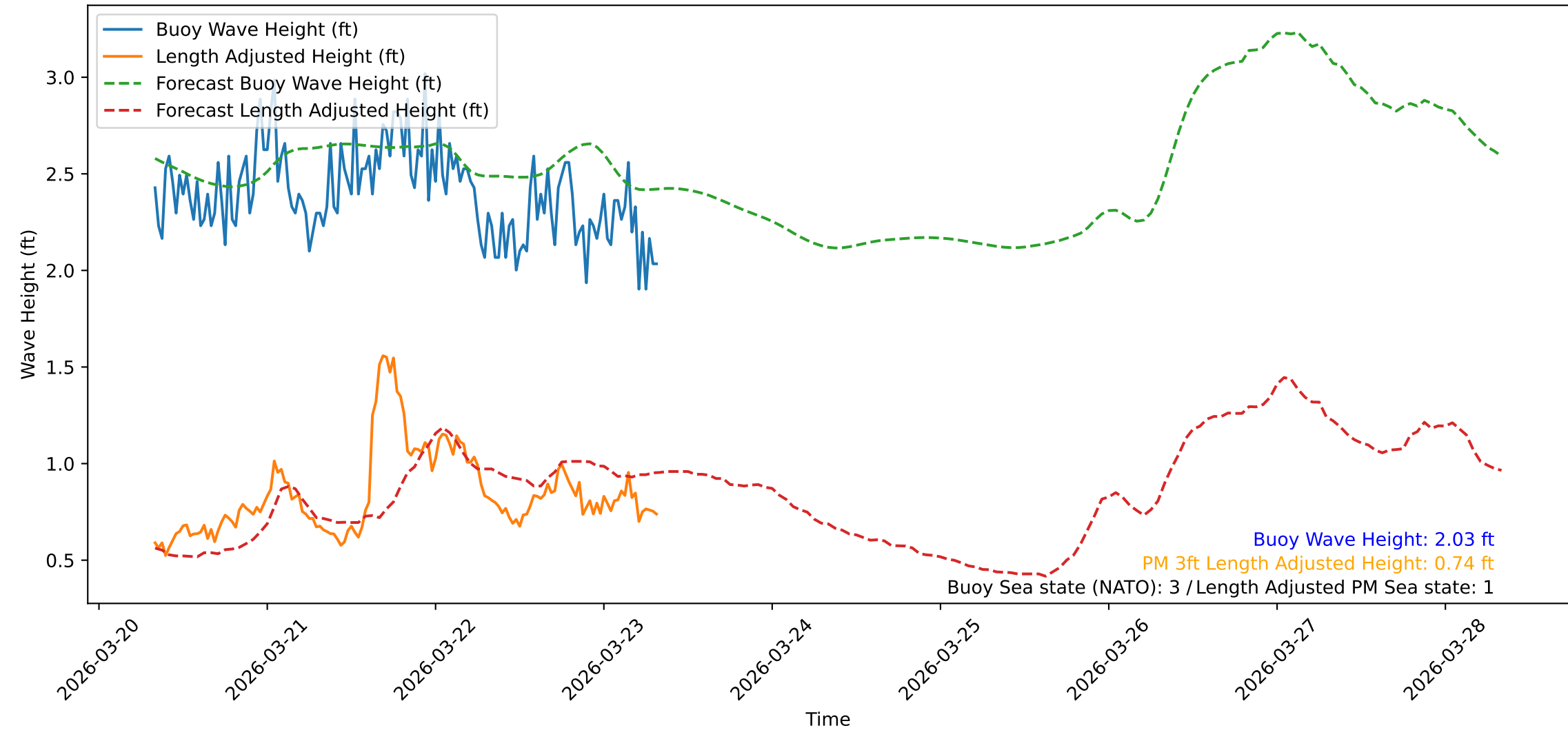
Wave Heights over Time for Oceanside Harbor at 2026-03-23 08:10:31
