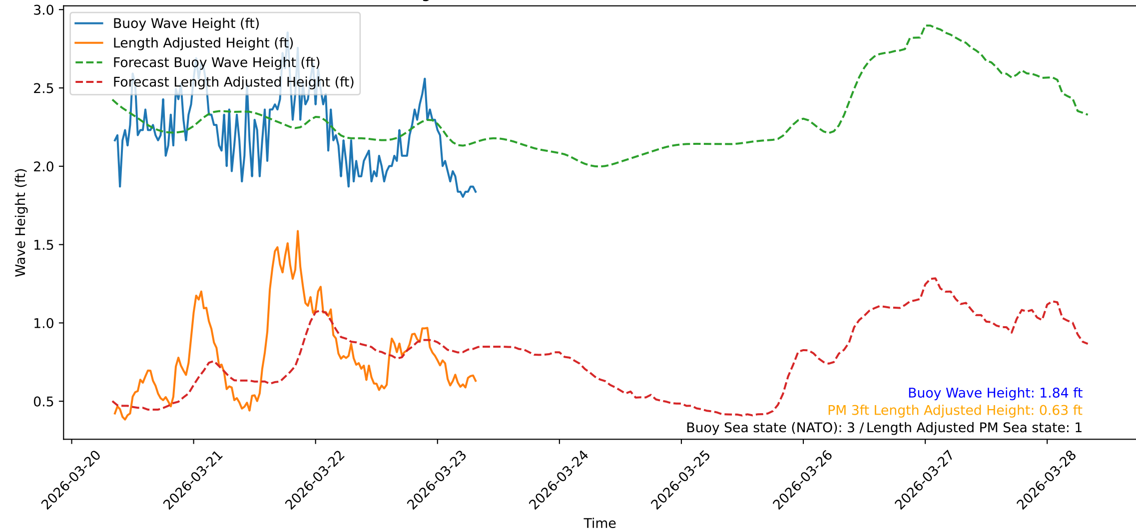
Wave Heights over Time for Red Beach at 2026-03-23 08:10:47
