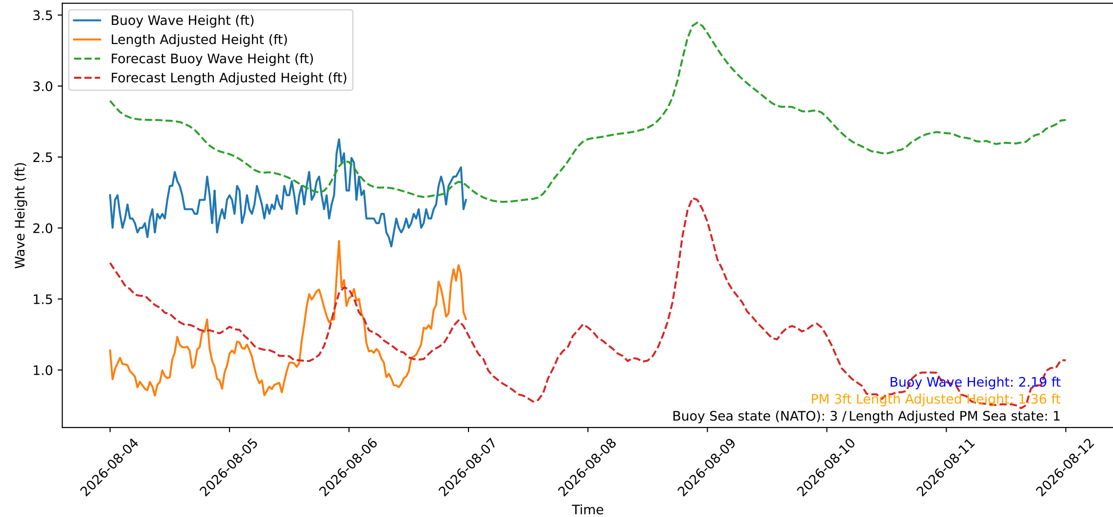
Wave Heights over Time for Green Beach at 2026-08-07 00:11:07
