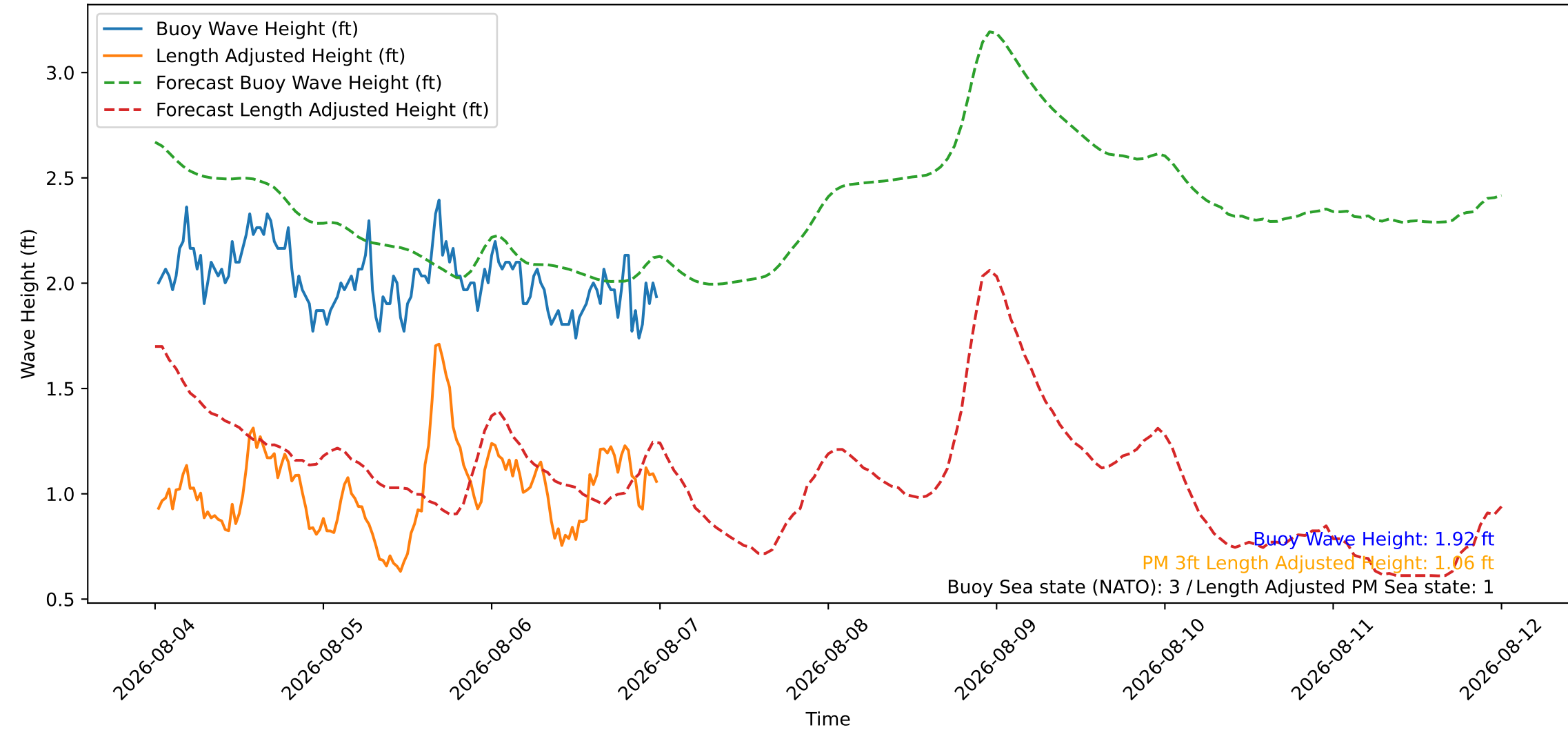
Wave Heights over Time for Red Beach at 2026-08-07 00:10:45
