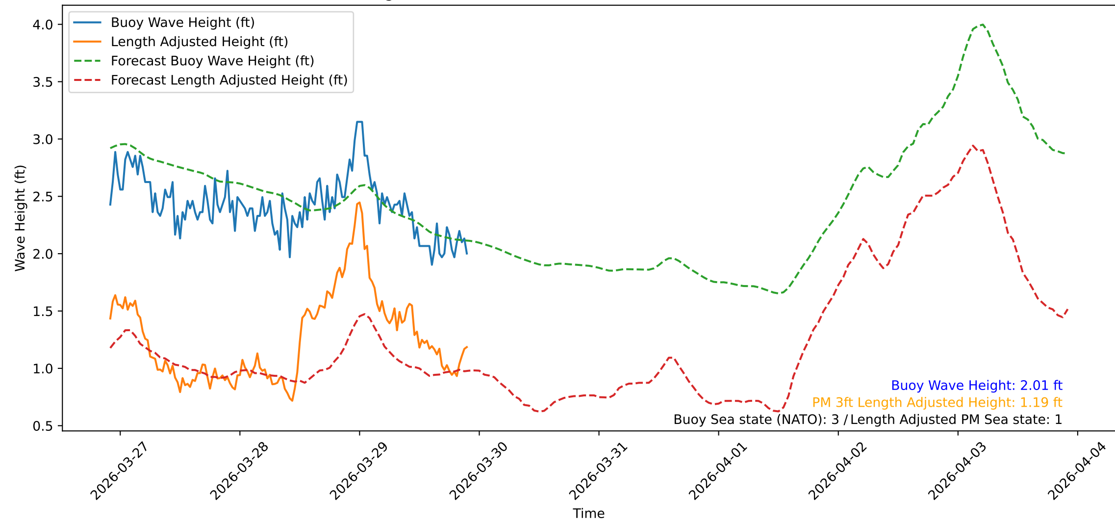
Wave Heights over Time for Oceanside Harbor at 2026-03-29 22:00:31
