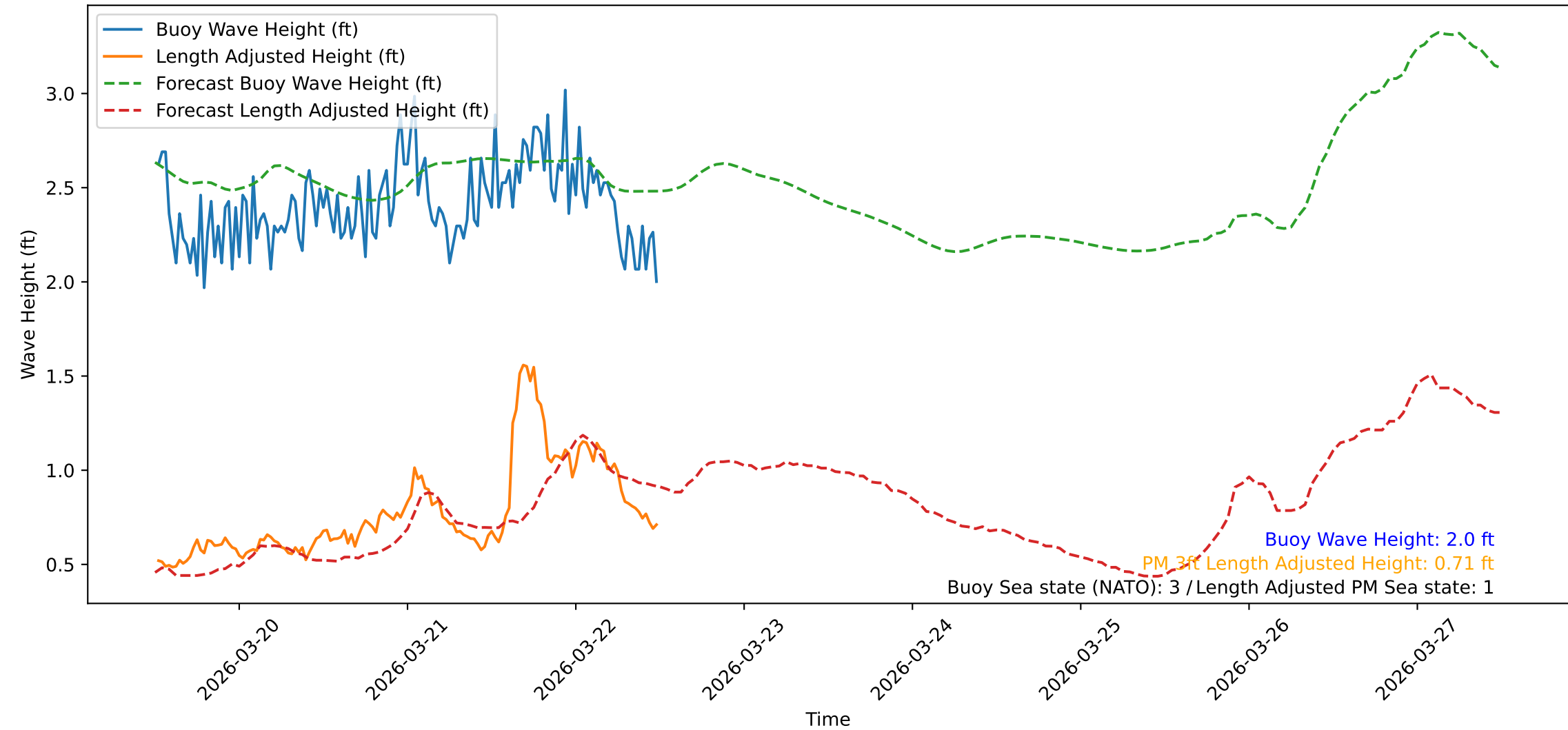
Wave Heights over Time for Oceanside Harbor at 2026-03-22 12:20:32
