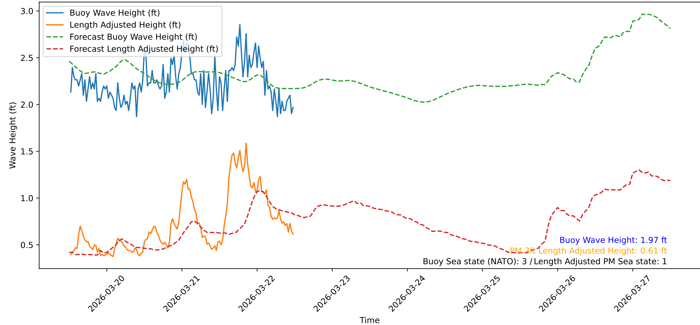
Wave Heights over Time for Red Beach at 2026-03-22 12:20:47
