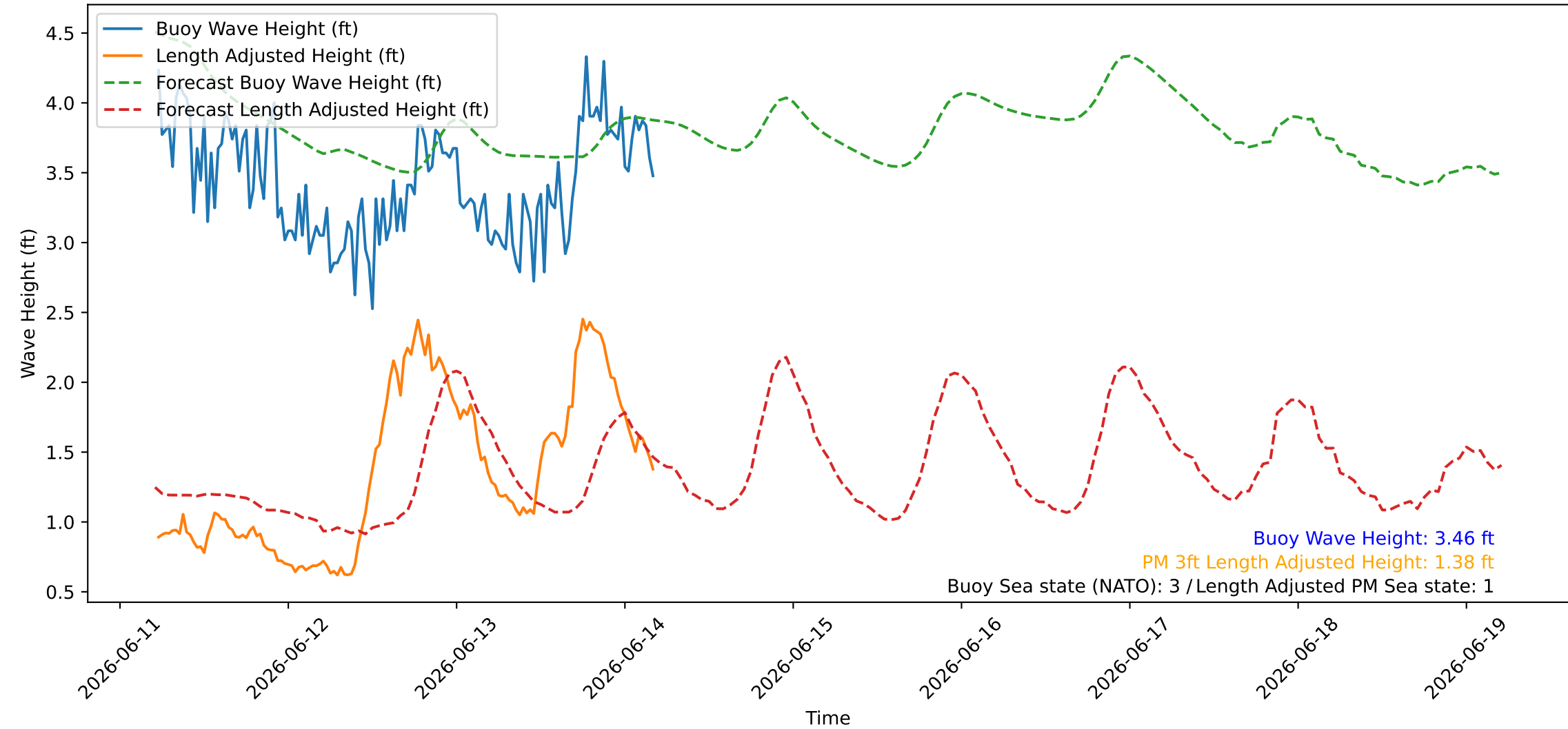
Wave Heights over Time for Red Beach at 2026-06-14 05:00:46
