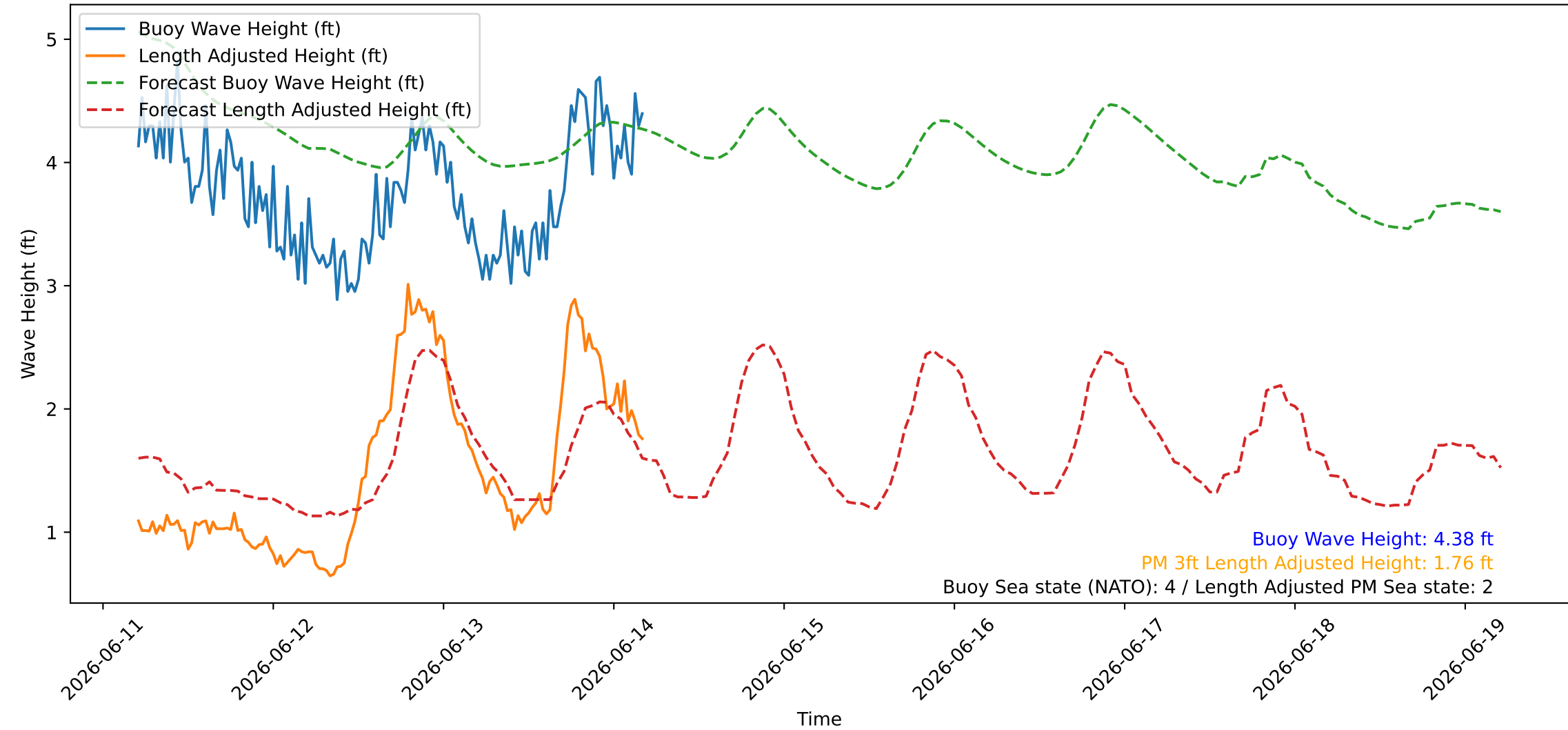
Wave Heights over Time for Green Beach at 2026-06-14 05:01:09
