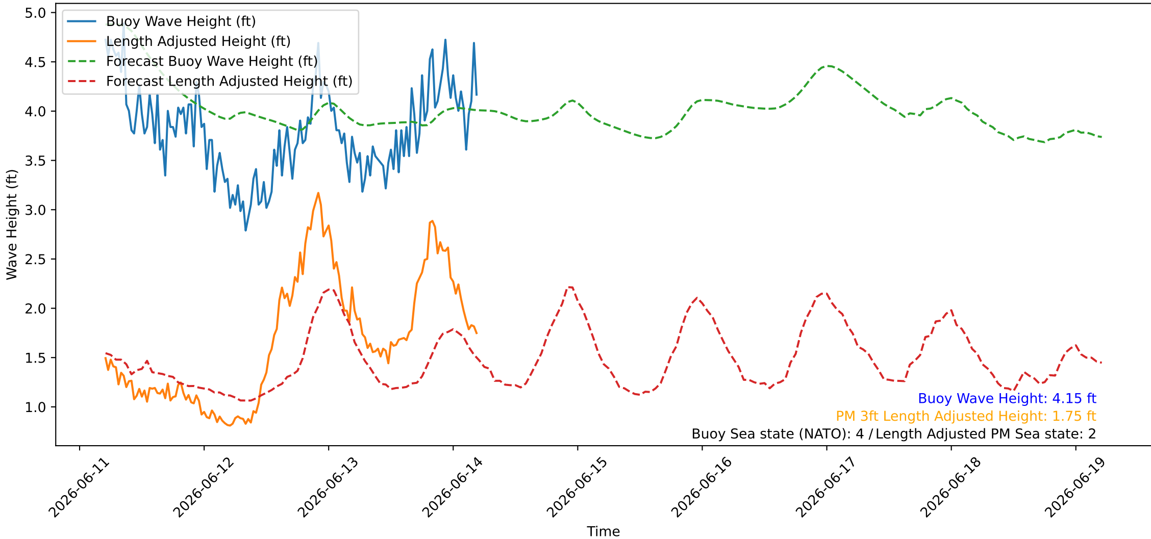
Wave Heights over Time for Oceanside Harbor at 2026-06-14 05:00:27
