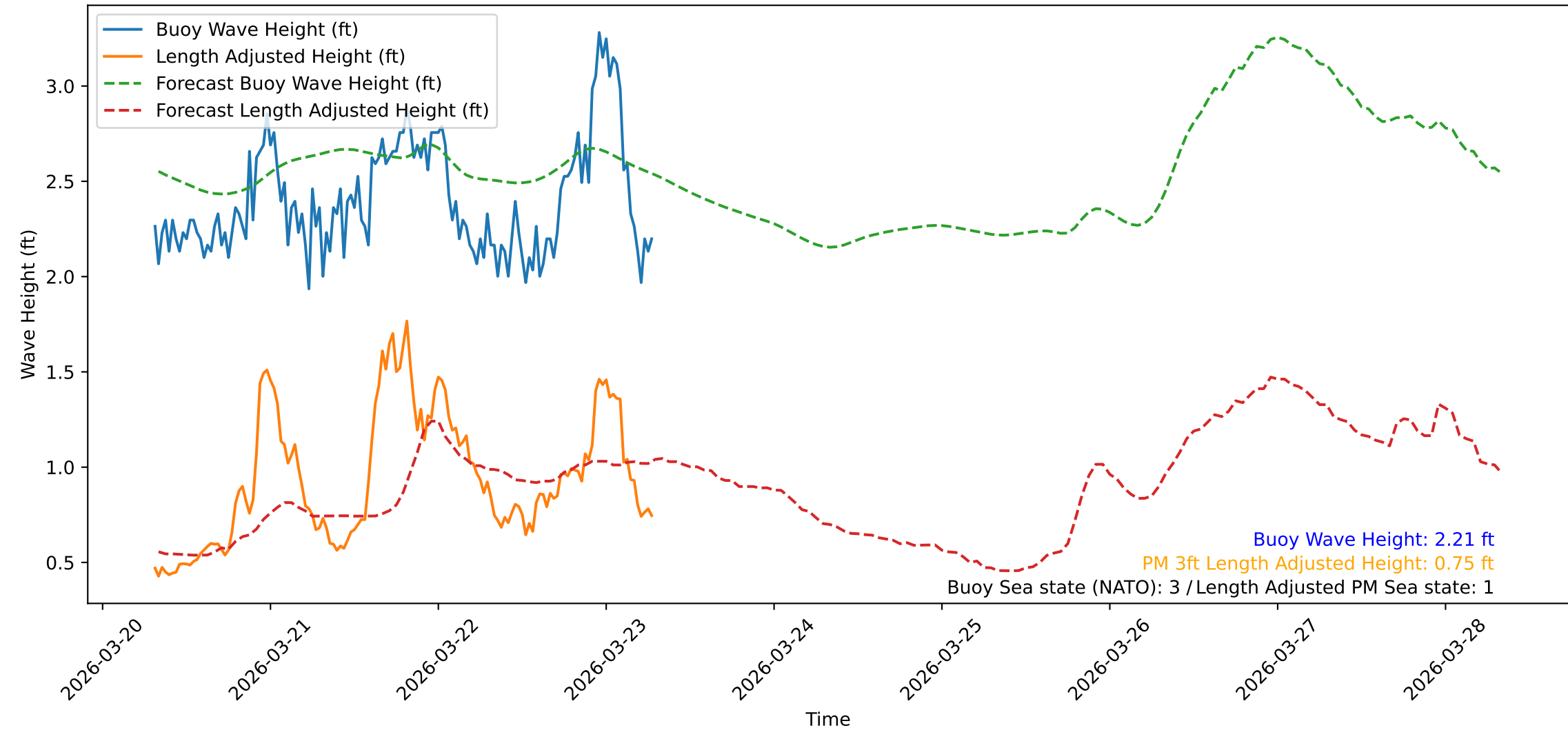
Wave Heights over Time for Green Beach at 2026-03-23 07:31:10
