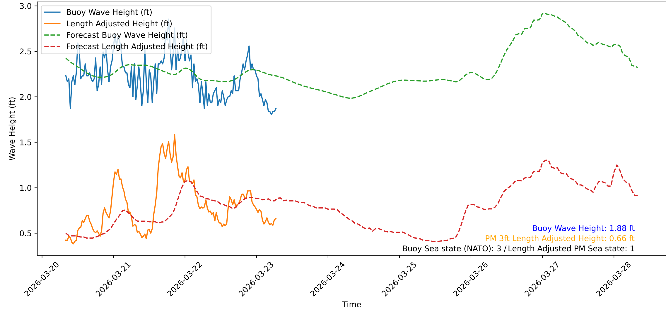
Wave Heights over Time for Red Beach at 2026-03-23 07:30:48
