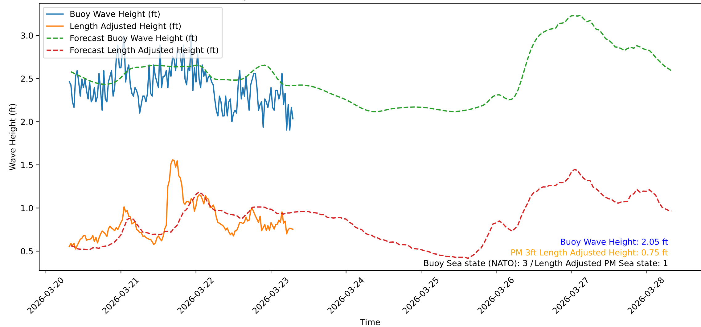
Wave Heights over Time for Oceanside Harbor at 2026-03-23 07:30:32
