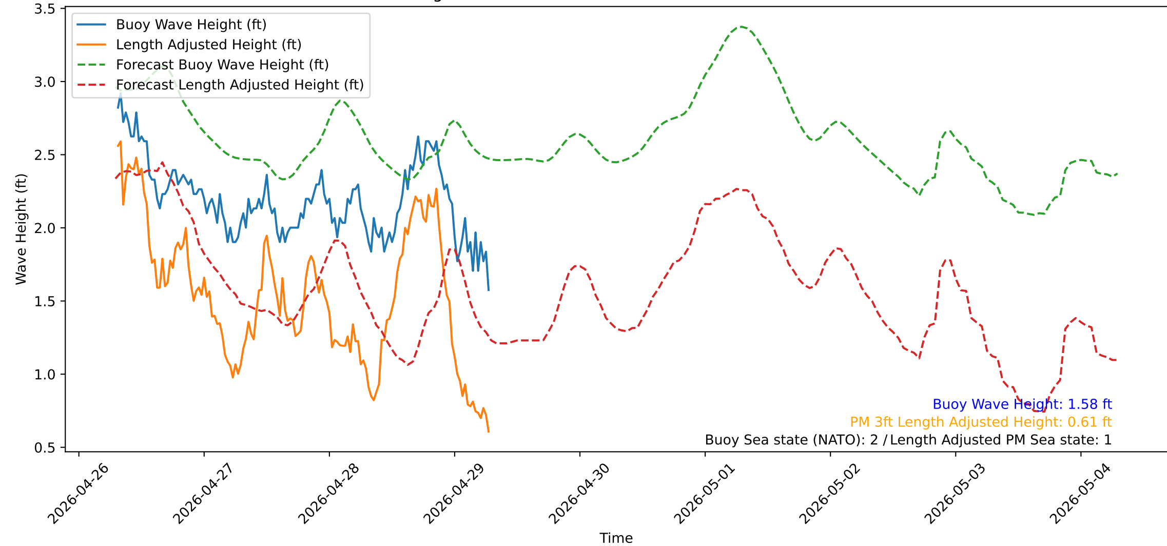
Wave Heights over Time for Red Beach at 2026-04-29 07:10:51
