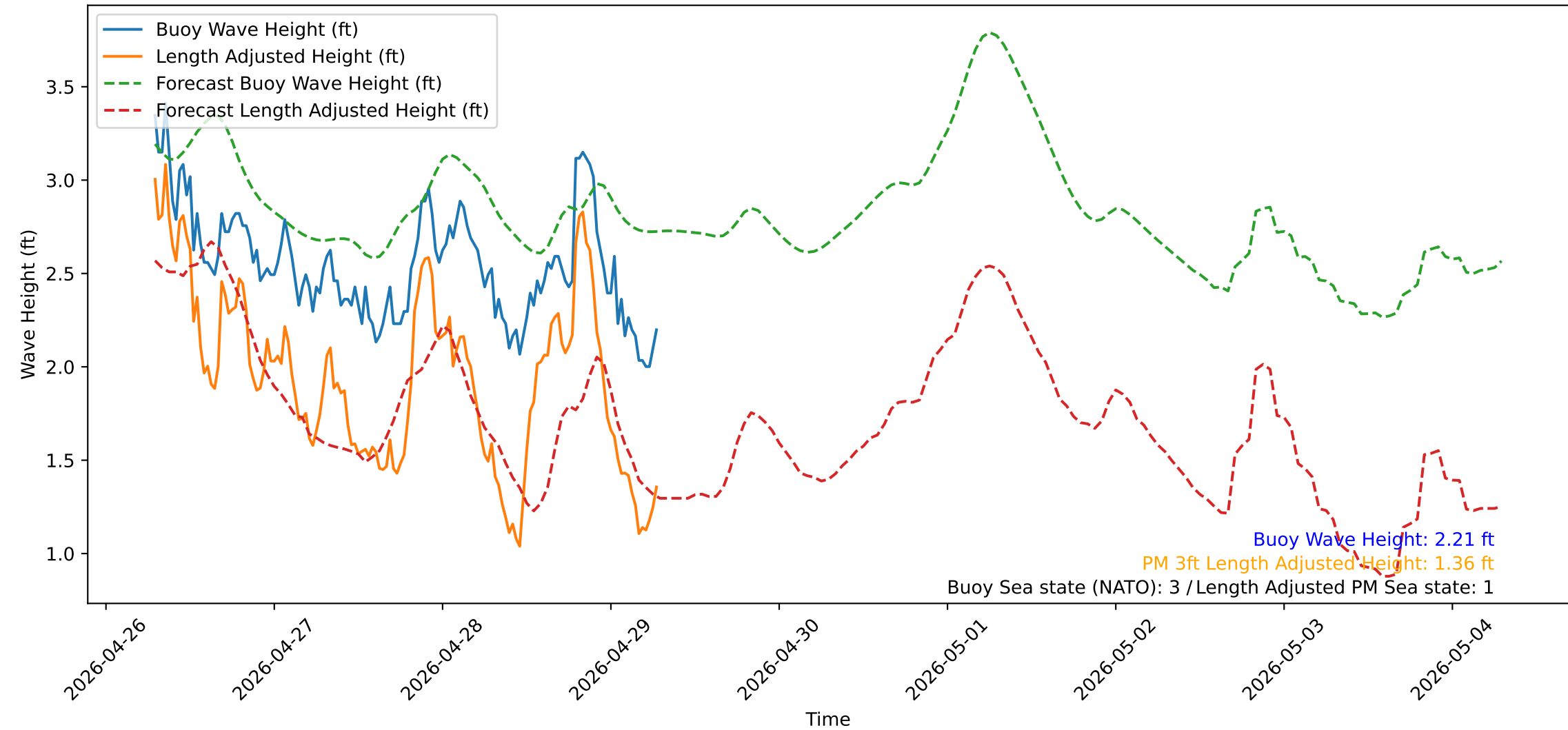
Wave Heights over Time for Green Beach at 2026-04-29 07:11:14
