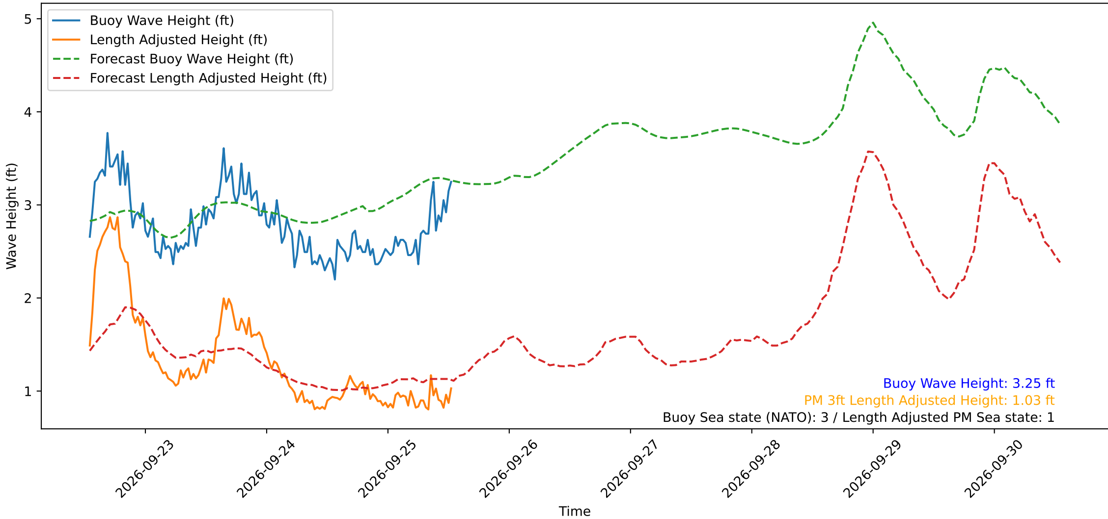
Wave Heights over Time for Oceanside Harbor at 2026-09-25 13:00:30
