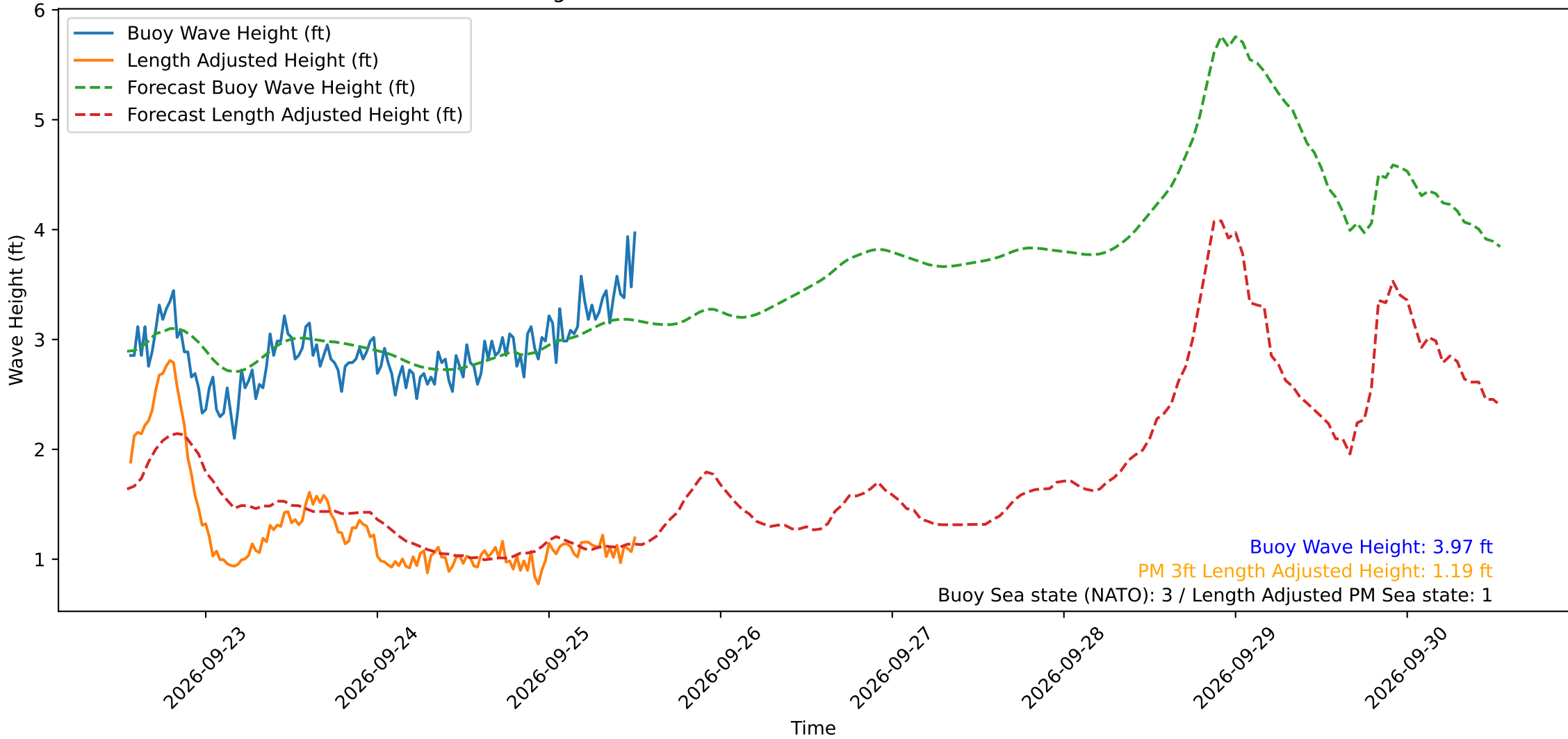
Wave Heights over Time for Green Beach at 2026-09-25 13:01:12
