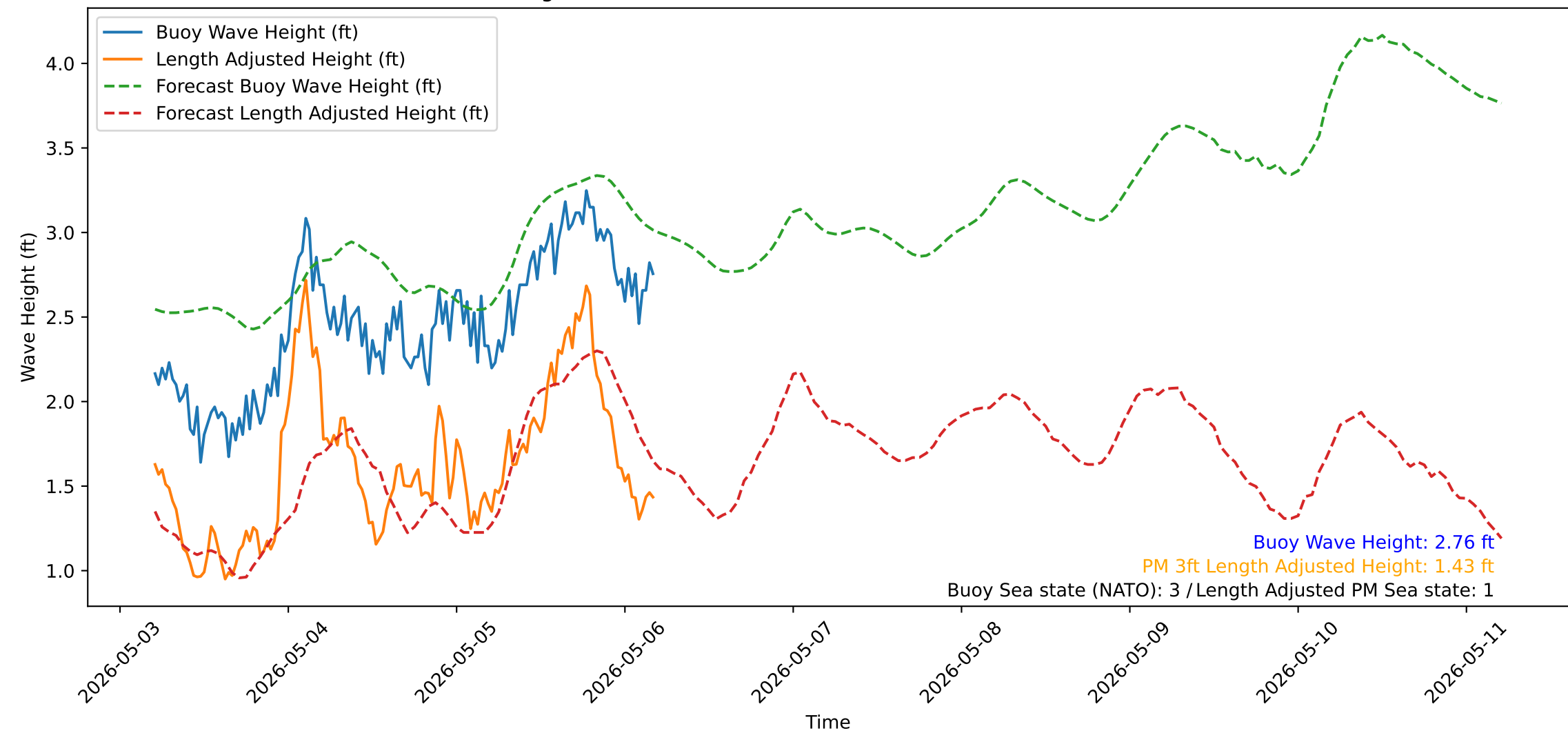
Wave Heights over Time for Oceanside Harbor at 2026-05-06 04:50:31
