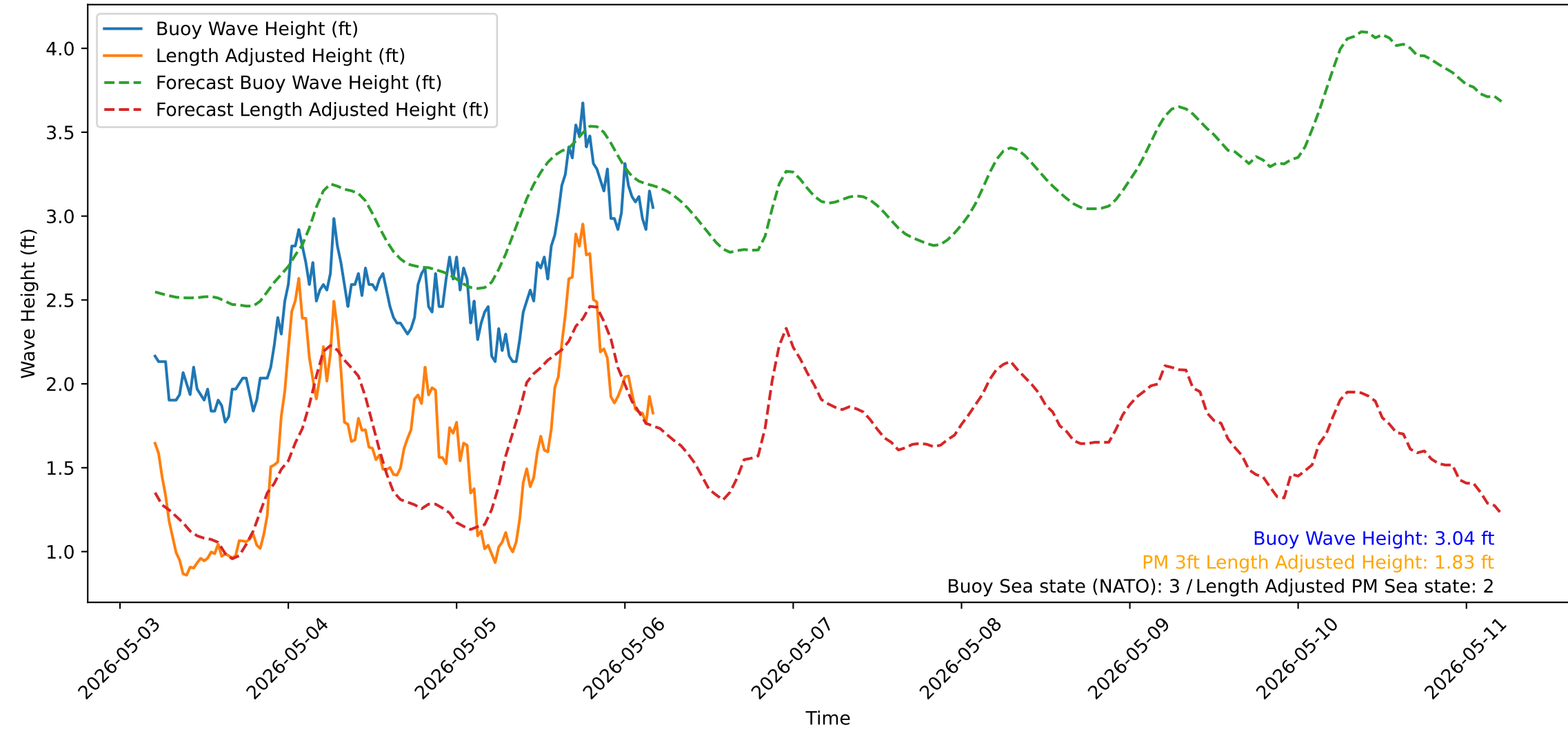
Wave Heights over Time for Green Beach at 2026-05-06 04:51:13
