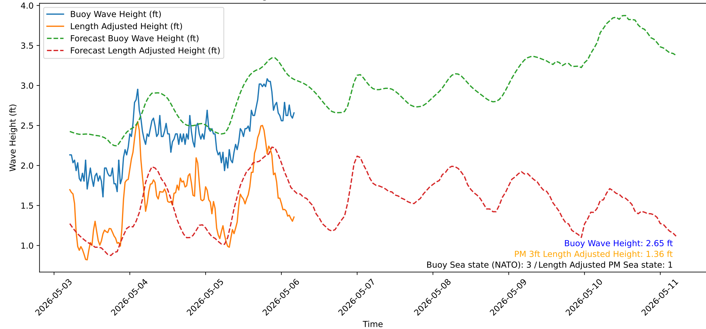
Wave Heights over Time for Red Beach at 2026-05-06 04:50:51
