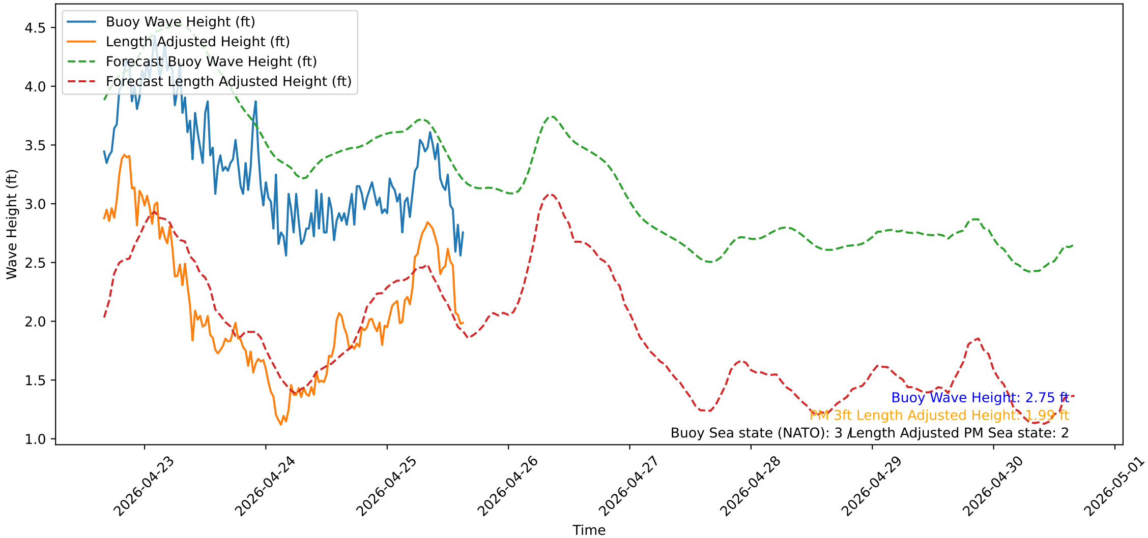
Wave Heights over Time for Oceanside Harbor at 2026-04-25 16:00:31
