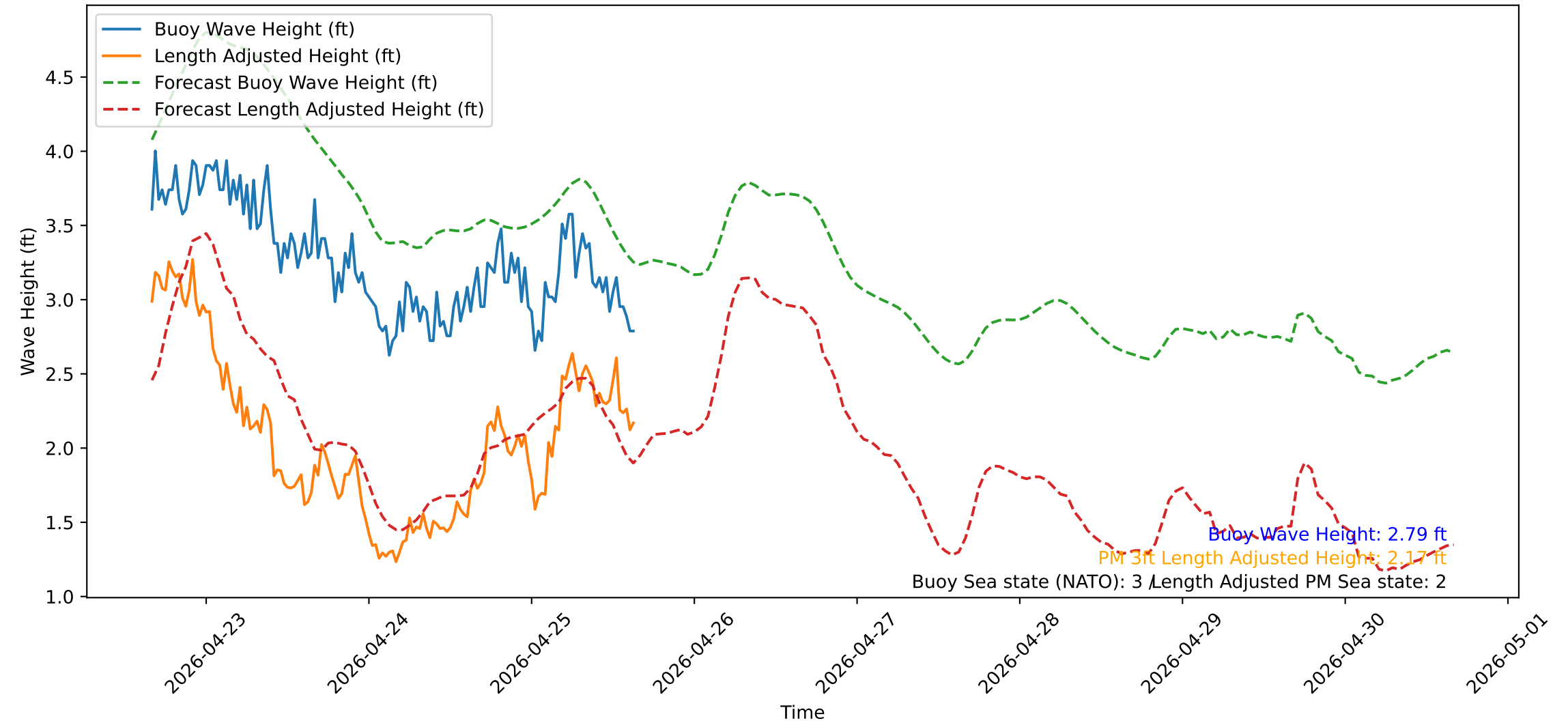
Wave Heights over Time for Green Beach at 2026-04-25 16:01:12
