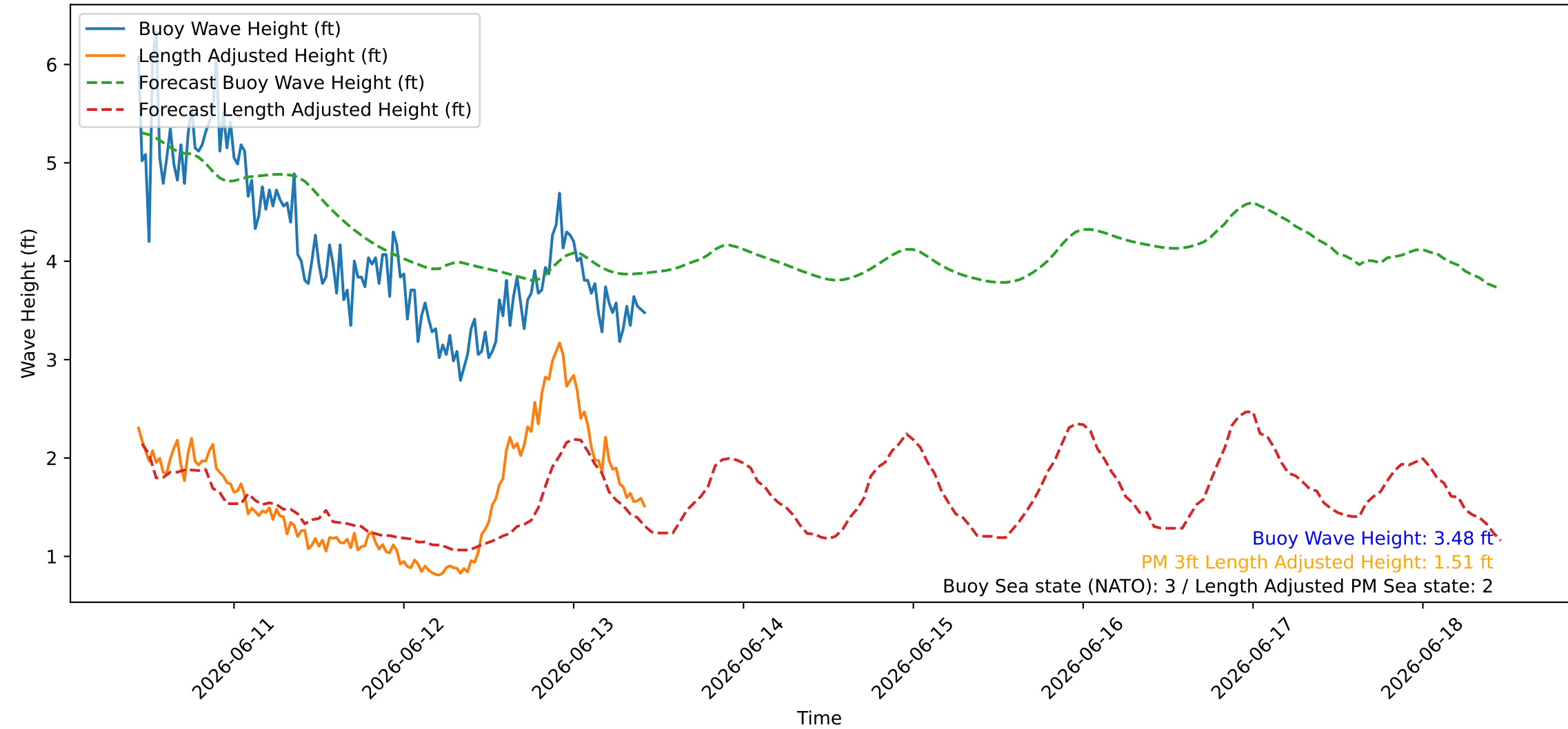
Wave Heights over Time for Oceanside Harbor at 2026-06-13 10:30:26
