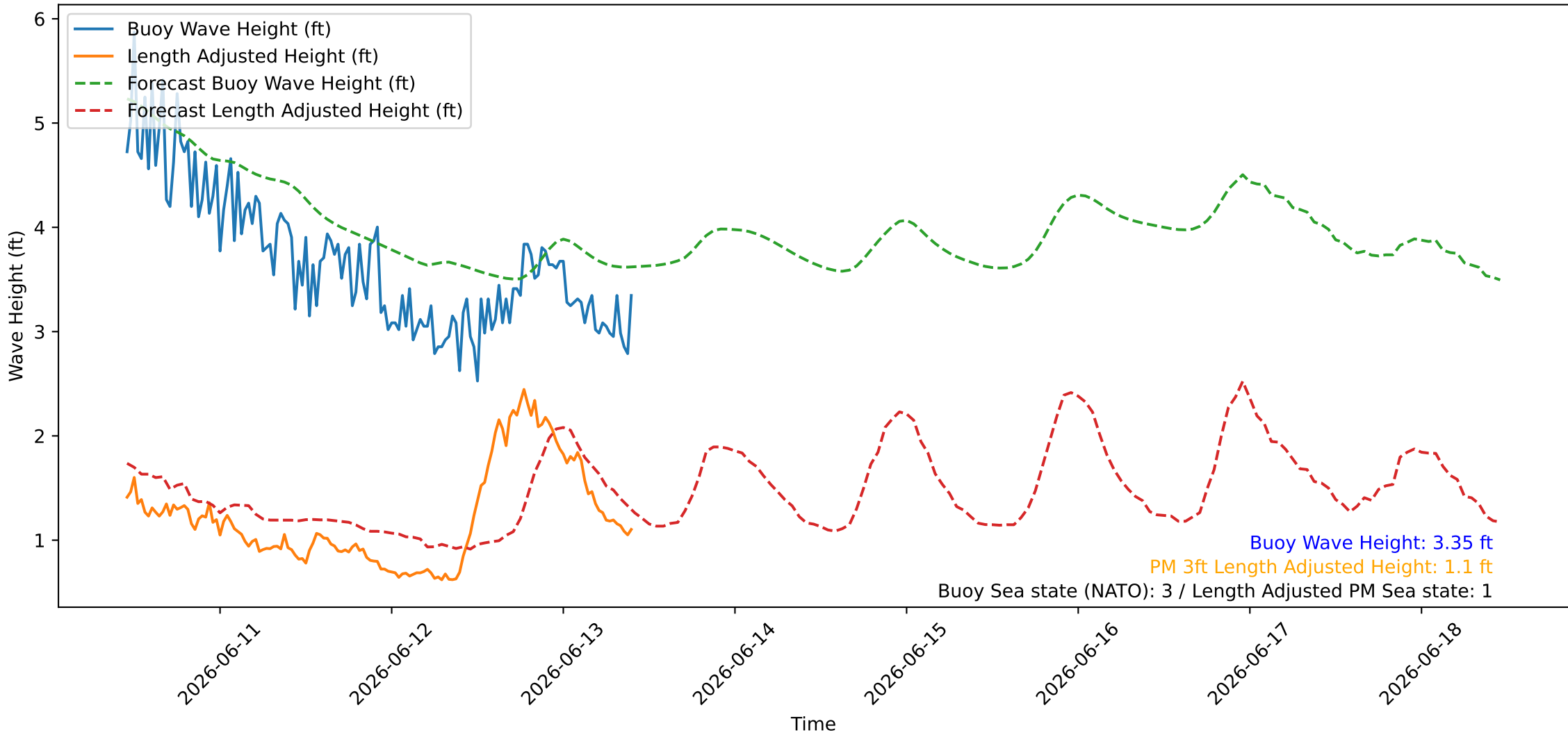
Wave Heights over Time for Red Beach at 2026-06-13 10:30:45
