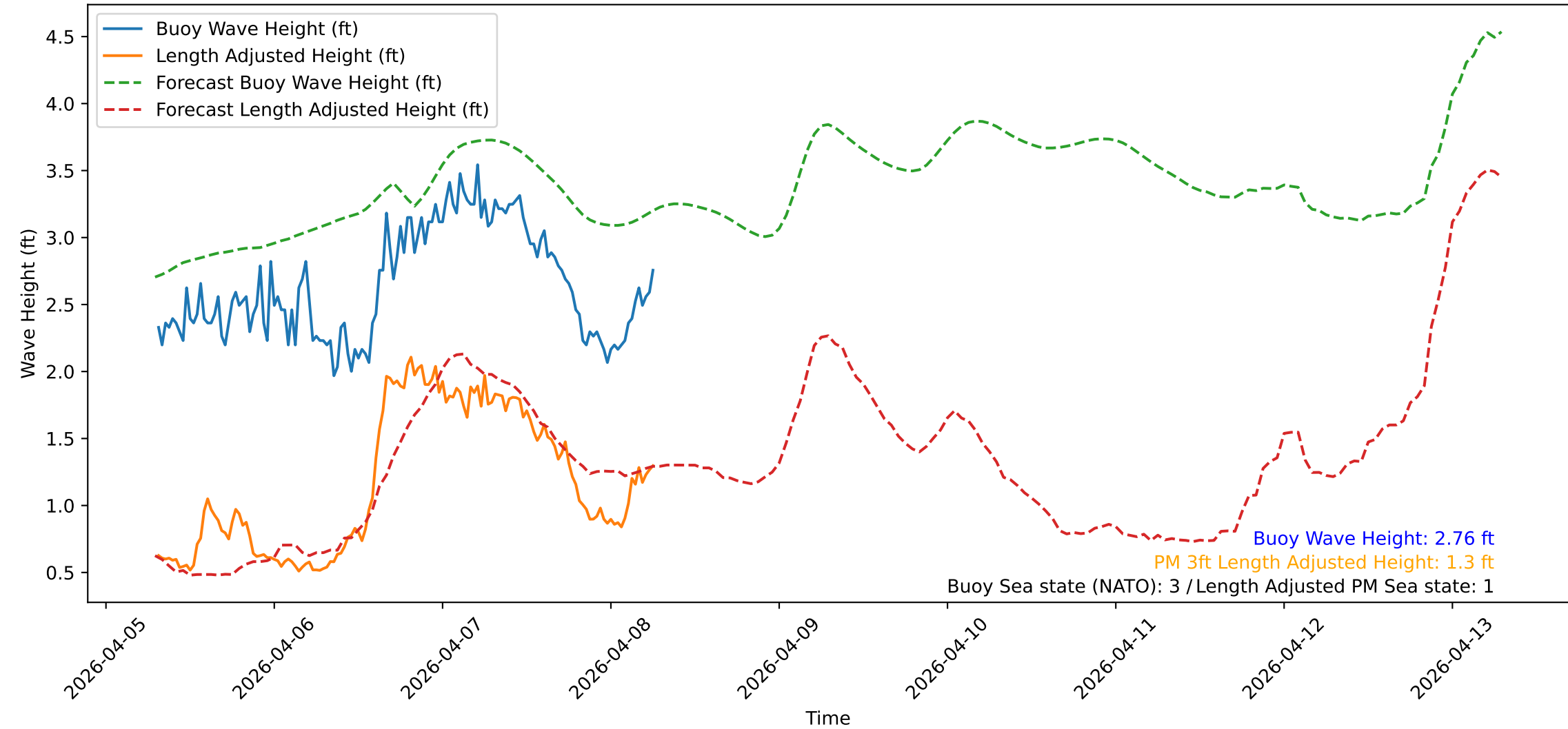
Wave Heights over Time for Red Beach at 2026-04-08 07:00:47
