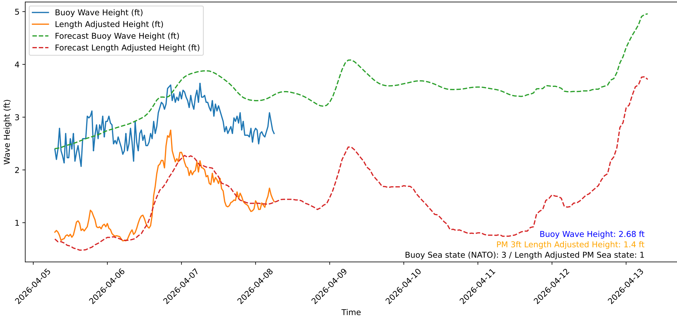
Wave Heights over Time for Oceanside Harbor at 2026-04-08 07:00:31
