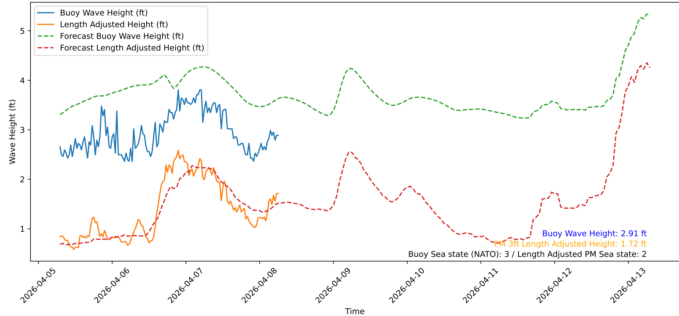
Wave Heights over Time for Green Beach at 2026-04-08 07:01:10
