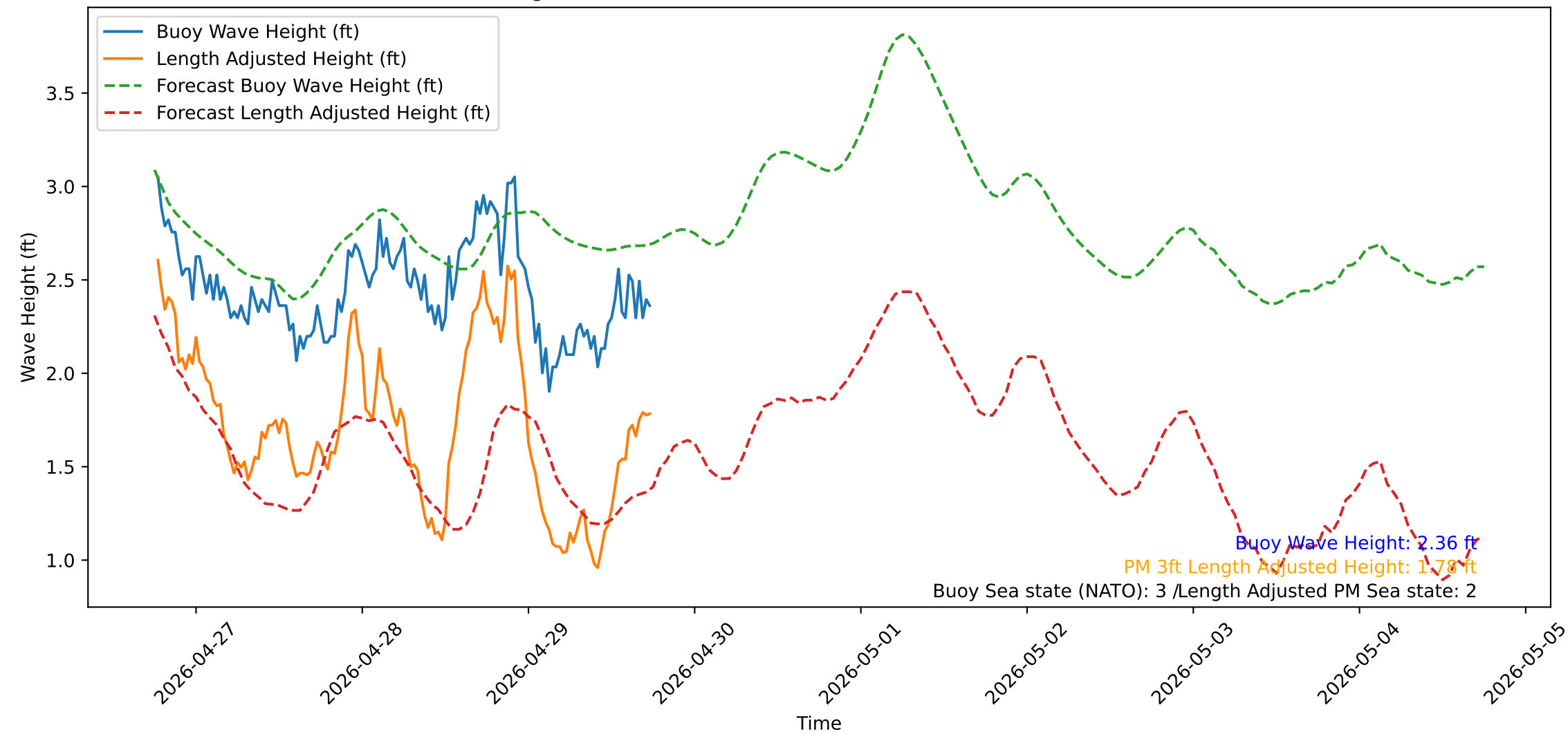
Wave Heights over Time for Oceanside Harbor at 2026-04-29 18:20:31
