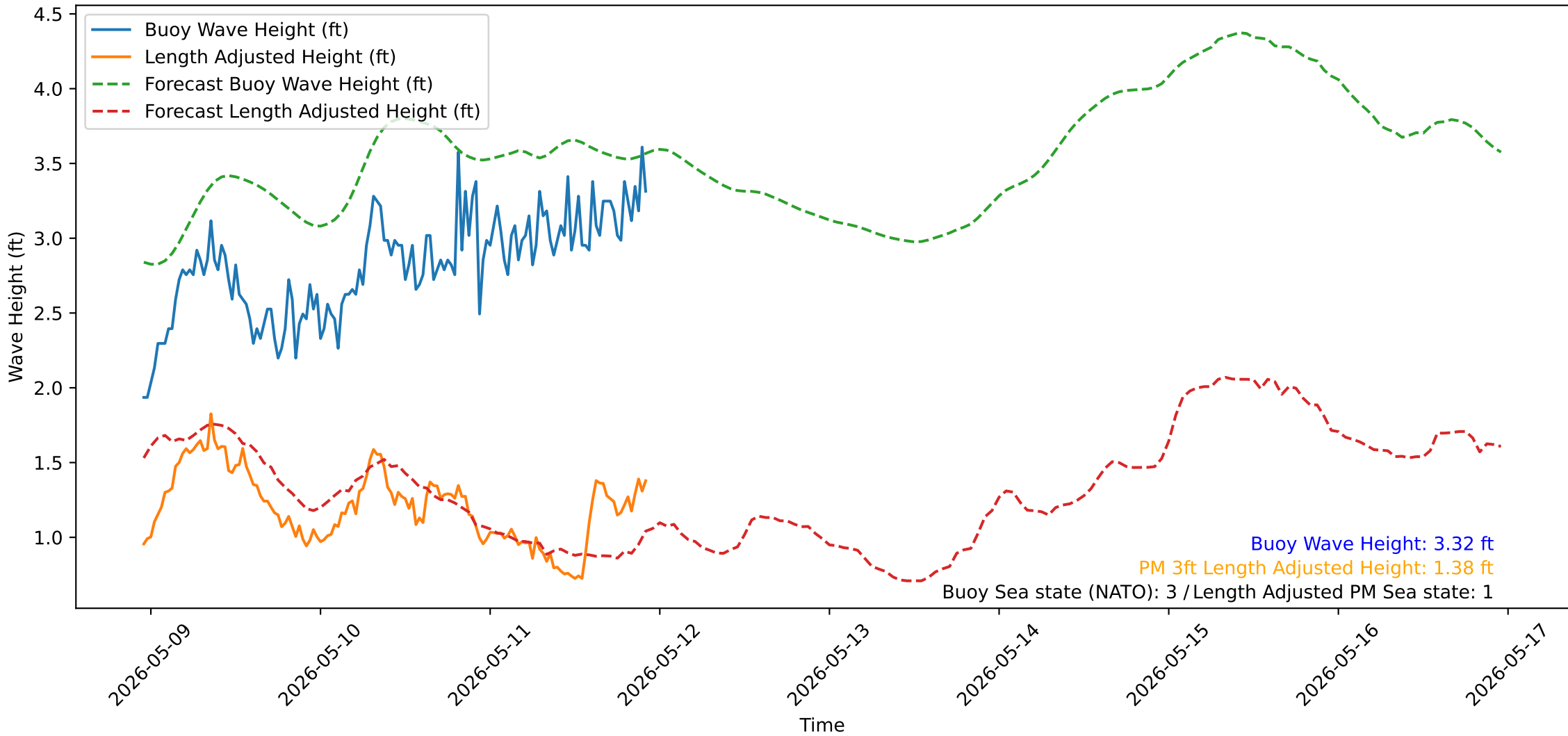
Wave Heights over Time for Oceanside Harbor at 2026-05-11 22:50:31
