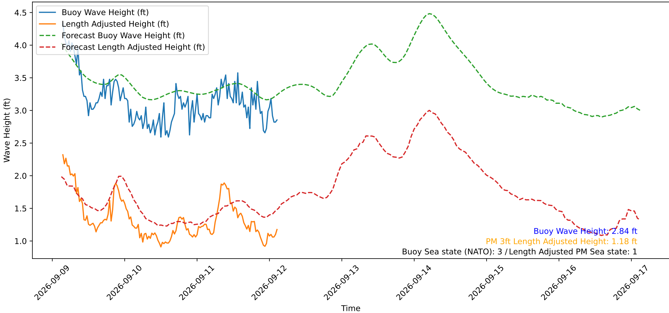
Wave Heights over Time for Green Beach at 2026-09-12 03:11:11
