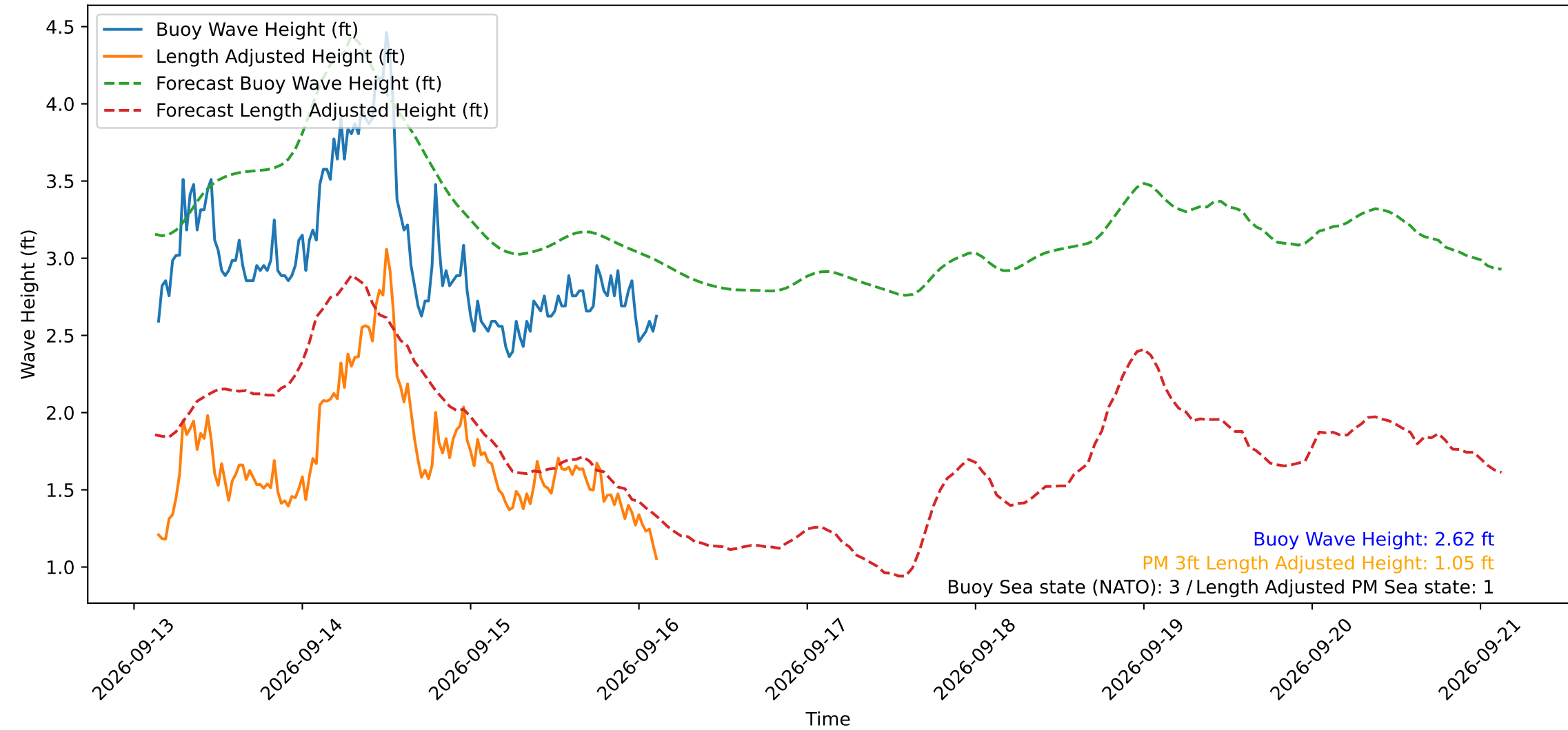
Wave Heights over Time for Oceanside Harbor at 2026-09-16 03:20:29
