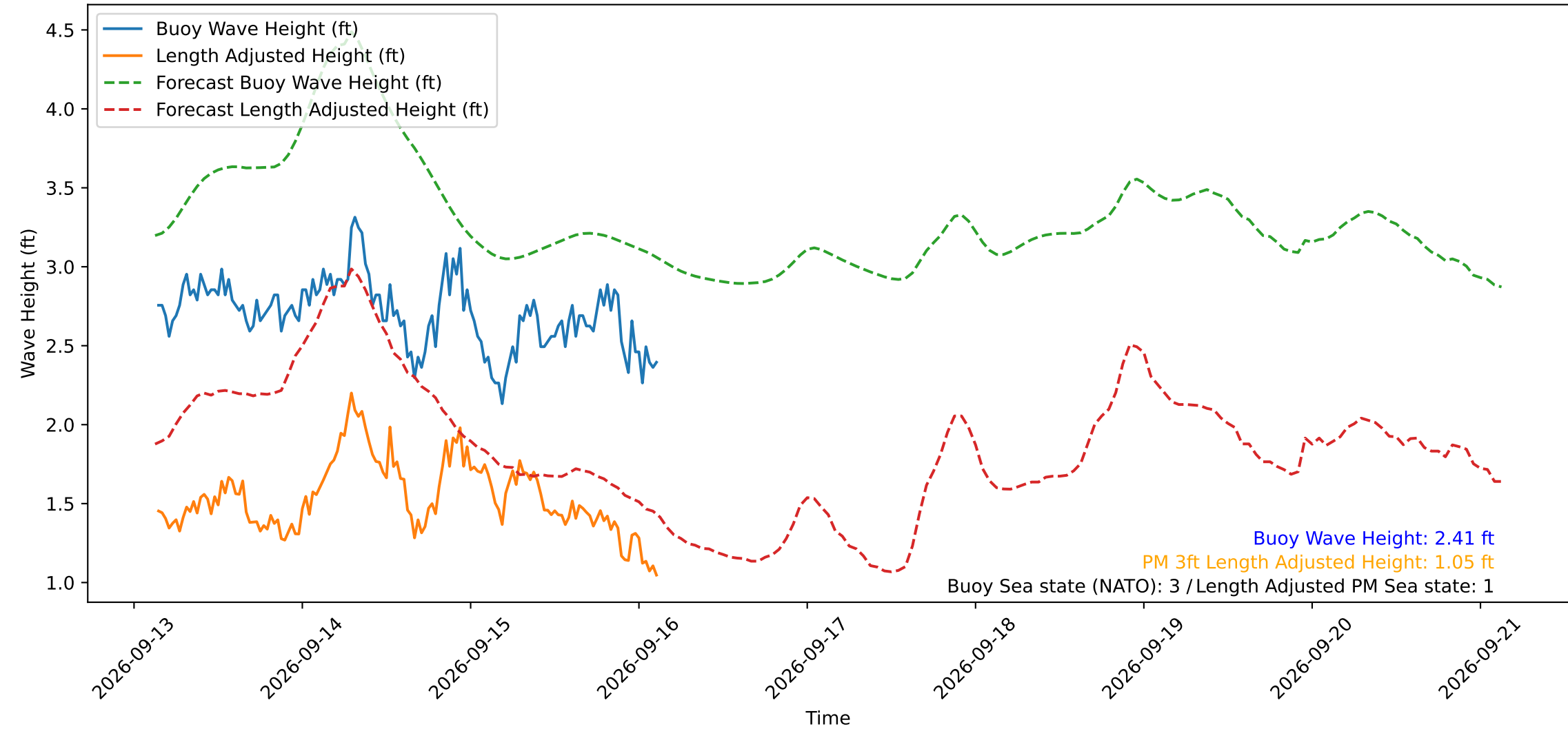
Wave Heights over Time for Green Beach at 2026-09-16 03:21:14
