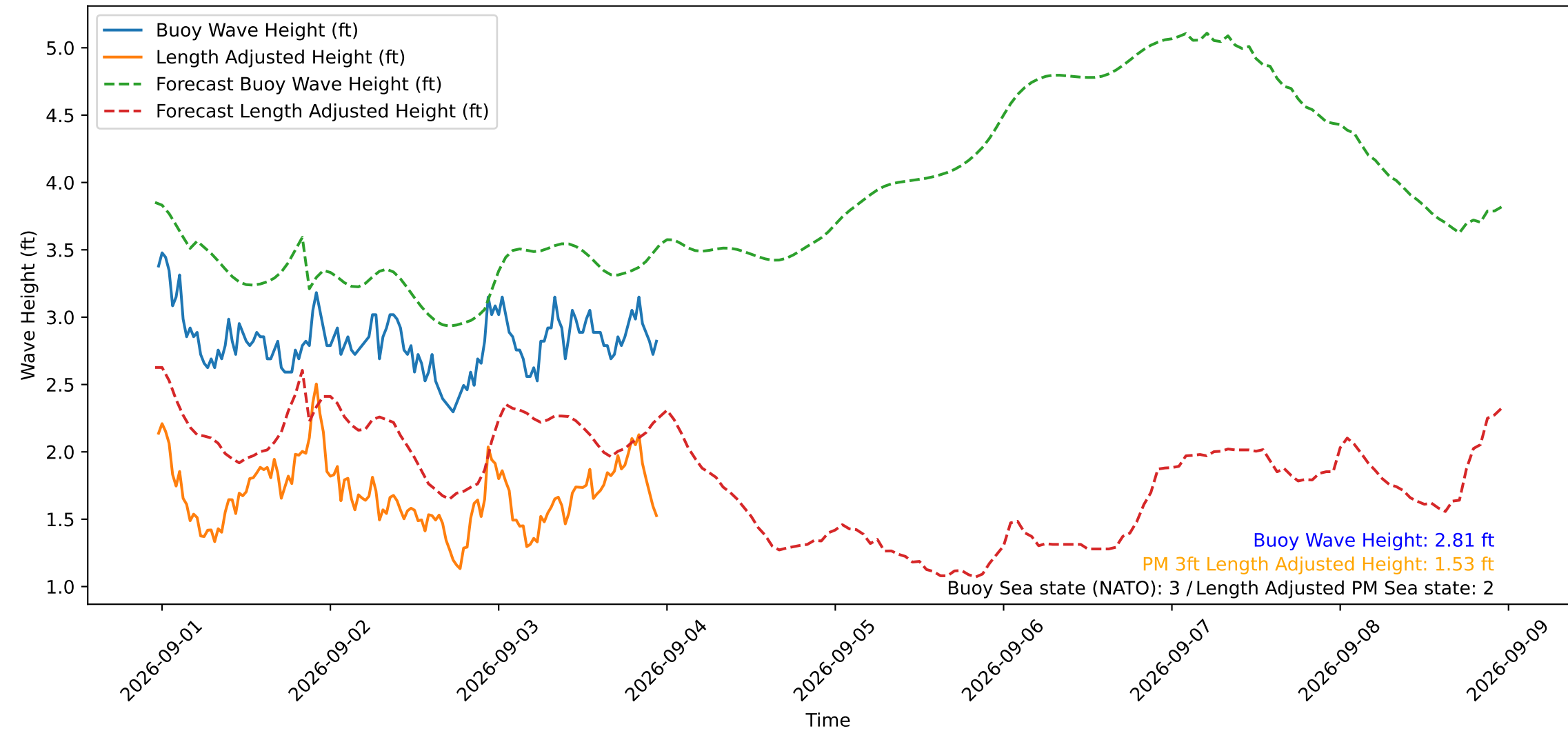
Wave Heights over Time for Red Beach at 2026-09-03 23:20:51
