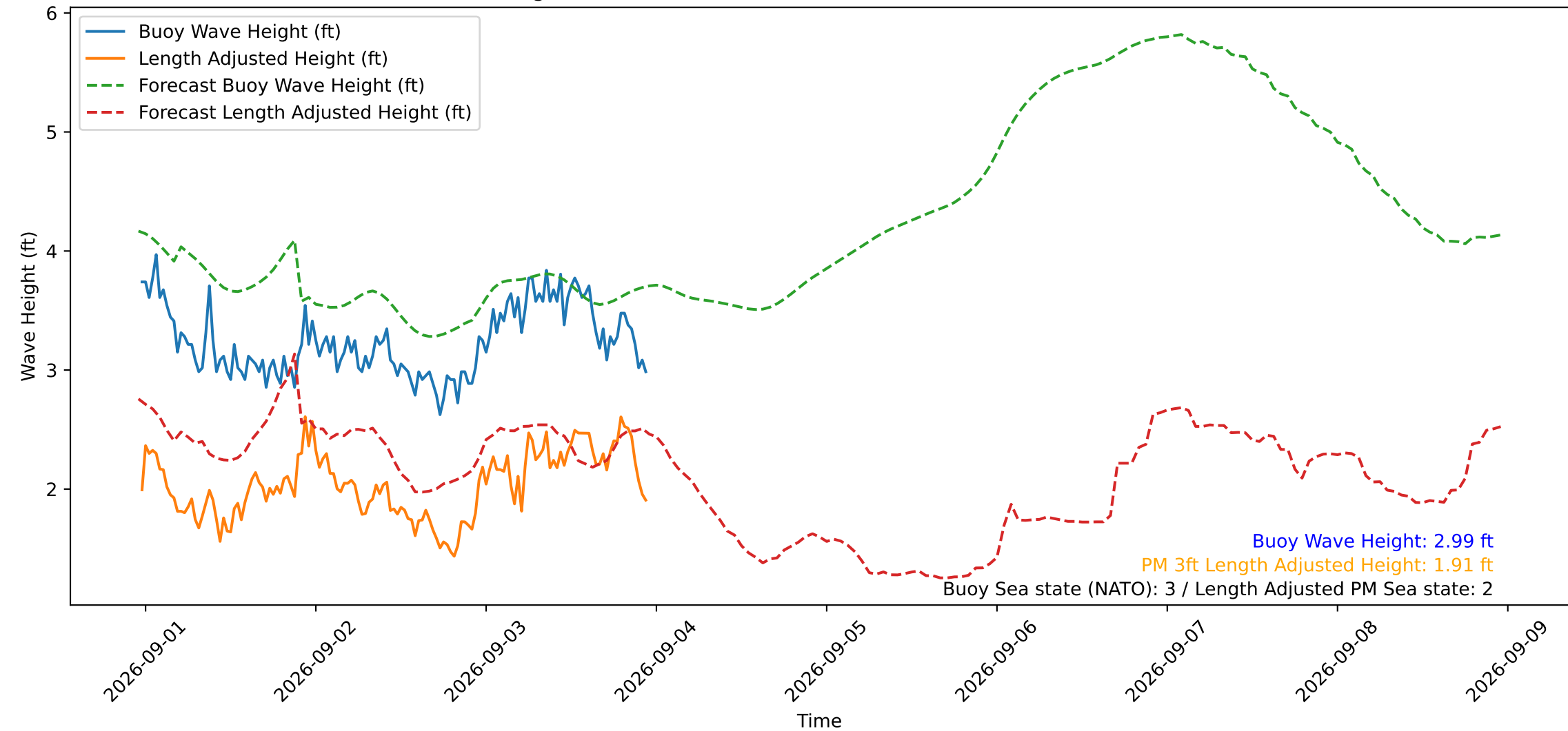
Wave Heights over Time for Oceanside Harbor at 2026-09-03 23:20:30
