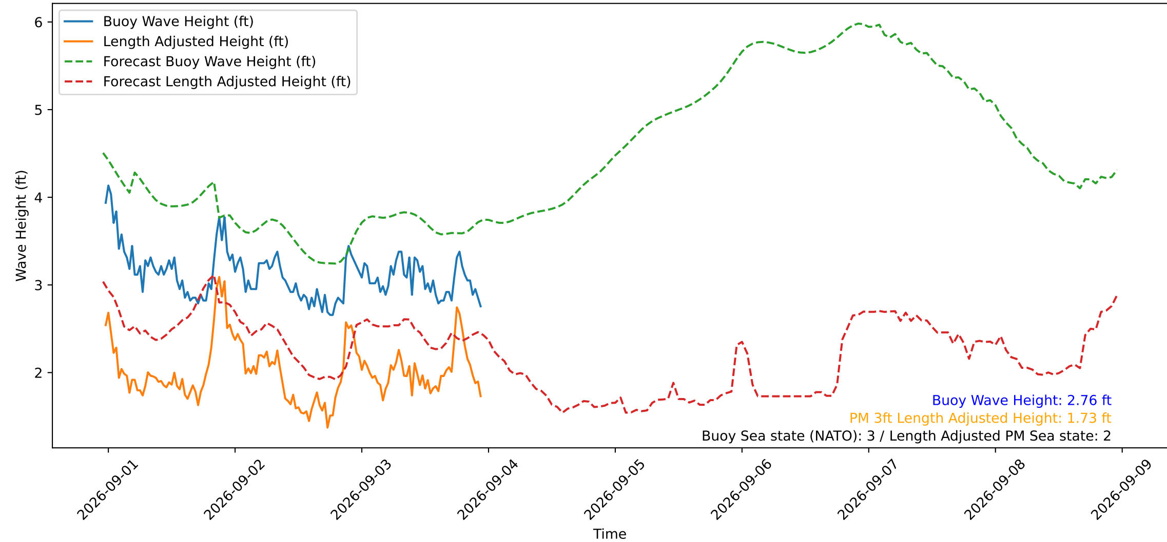
Wave Heights over Time for Green Beach at 2026-09-03 23:21:15
